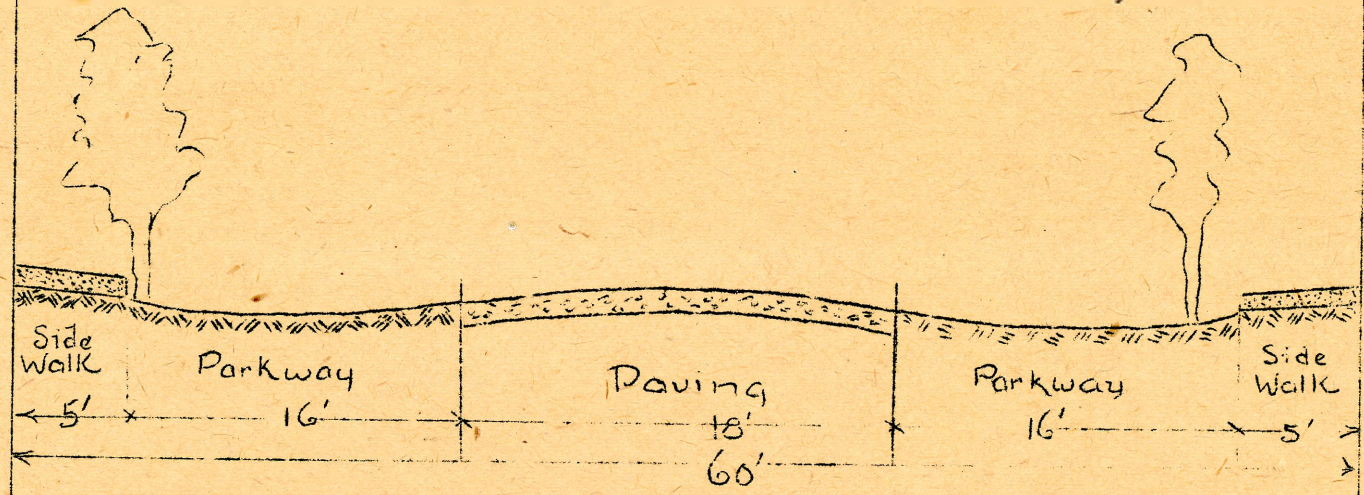
18 FOOT SINGLE DRIVEWAY ON 60' STREET
