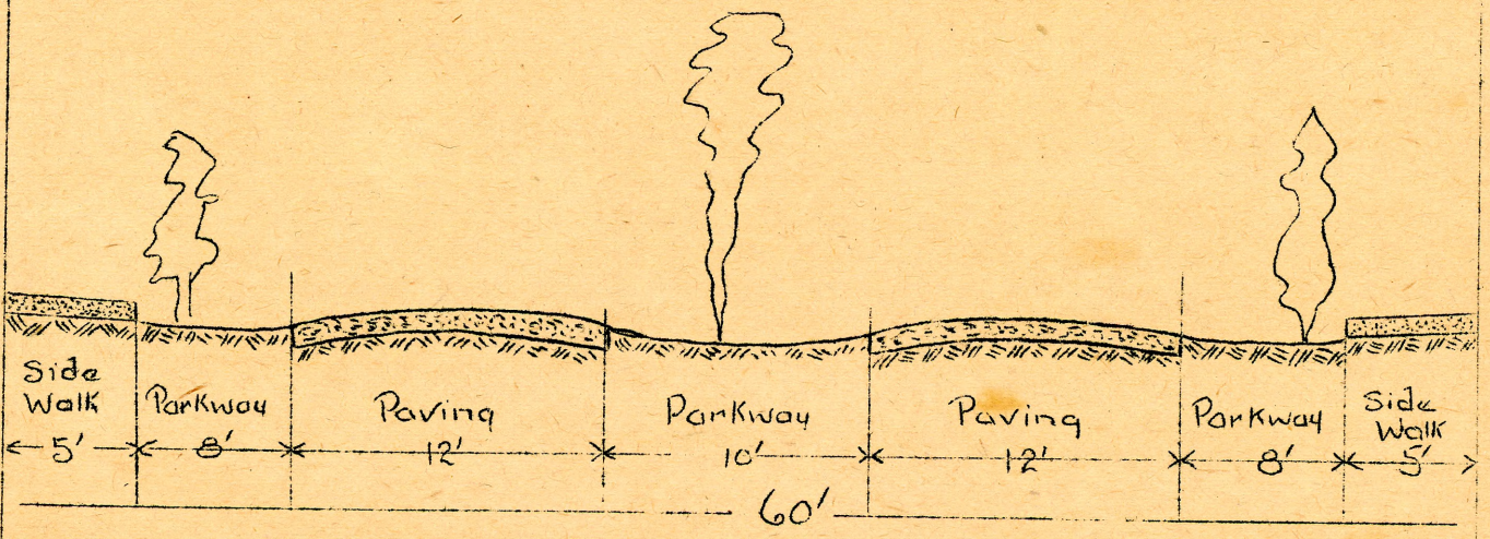
2- 12' FOOT DRIVEWAYS ON 60 FOOT STREET
