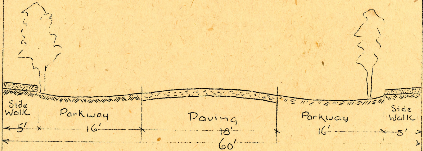
18 FOOT SINGLE DRIVEWAY ON 60' STREET
