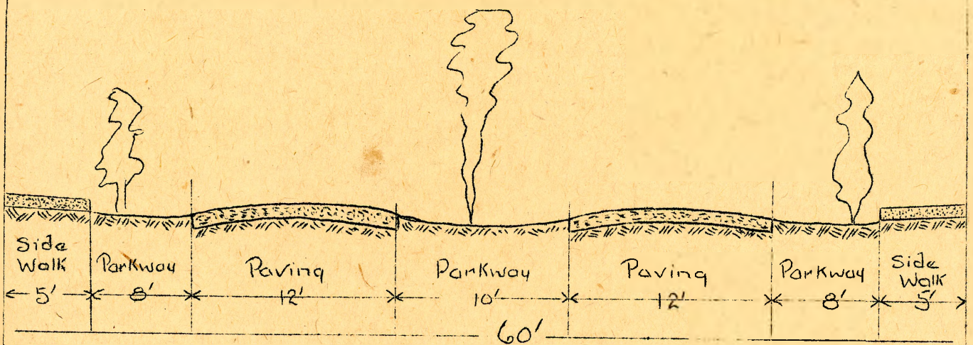
2- 12' FOOT DRIVEWAYS ON 60 FOOT STREET
