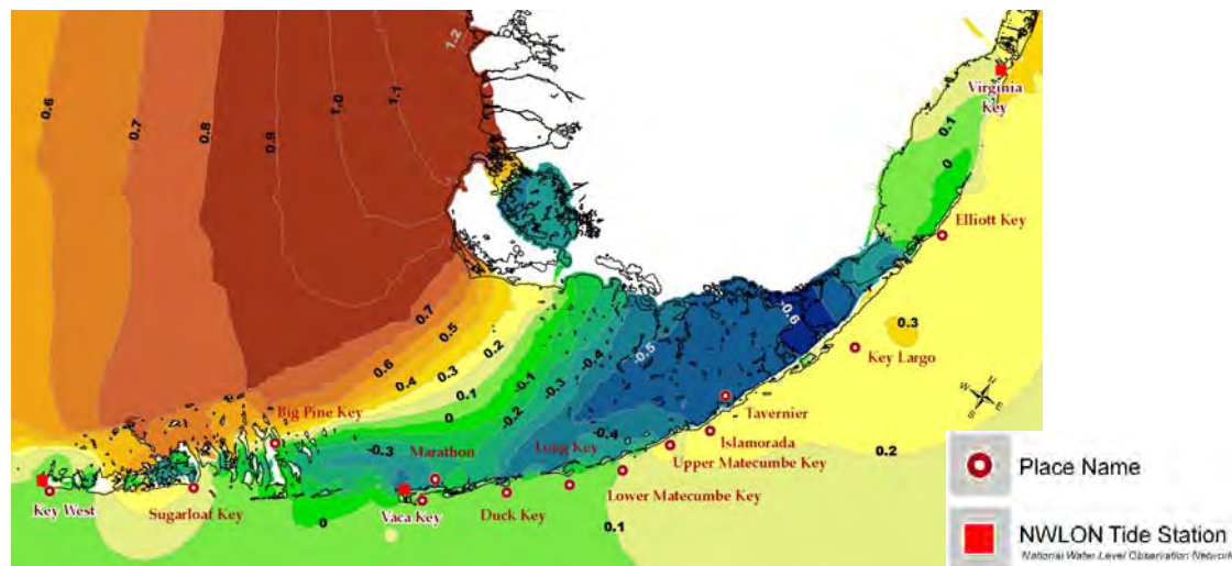
Figure 7 - VDatum MHHW Tidal Variability by Florida Bay, in NAVD88 ft (FLsouth01) - Without inland extrapolation
