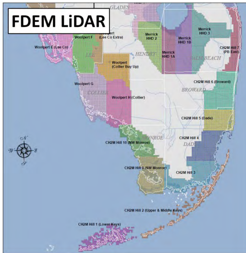
Figure 1 – Geographic Extent of the 2007-08 FDEM LiDAR Dataset within South Florida.
