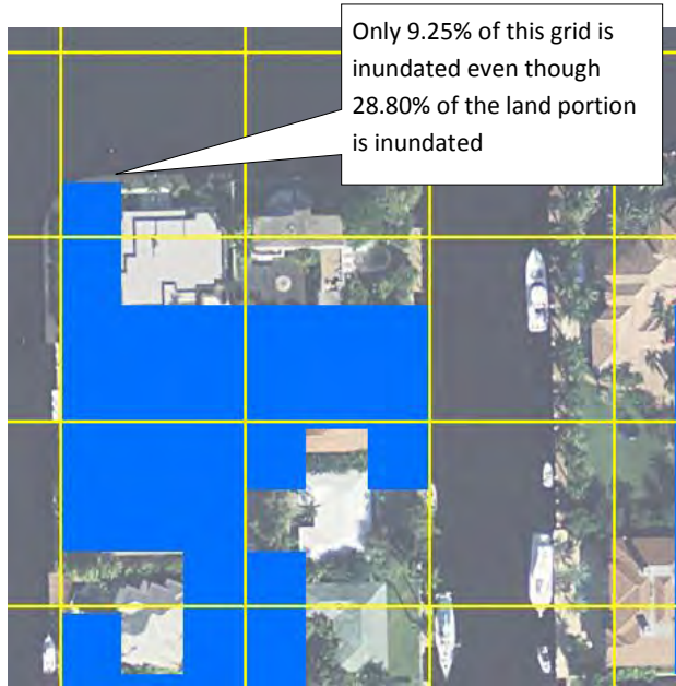
Figure 6: pGrids without water features removed
