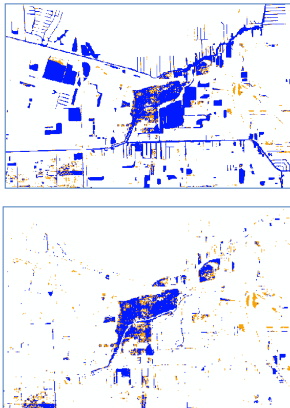
Figure 1: (Top) Inundation grid without water features removed. (Bottom) Inundation grid after water feature removal
