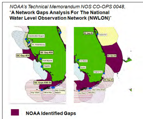
Figure 16 – NWLON Network Gaps Identified by NOAA Credit: NOAA CO-OPS. (Gill, March 2008).
