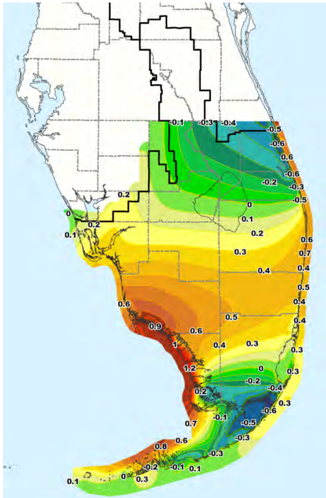
Figure 8 – NOAA CSC's MHHW Tidal Surface, Version 1 (After Inland Extrapolation) (NAVD88 in ft) – 1500-ft cell size
