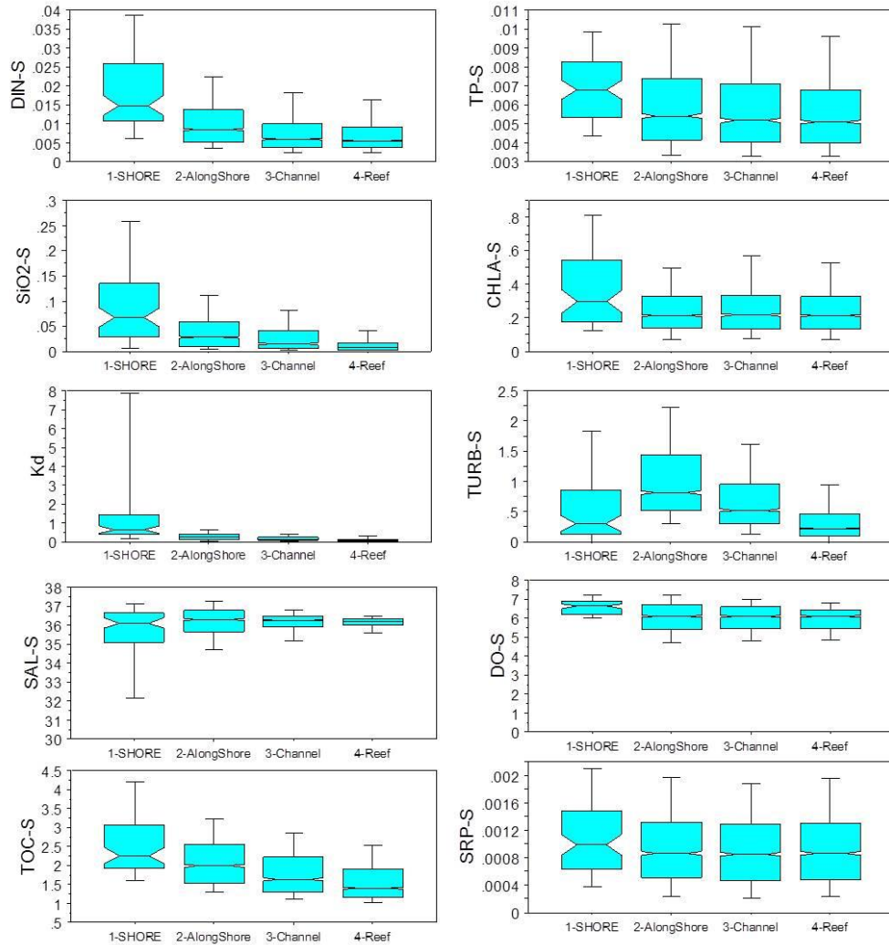
Figure 14: Nutrient and response changes along transect from close-to-shore sites to the reef-track
