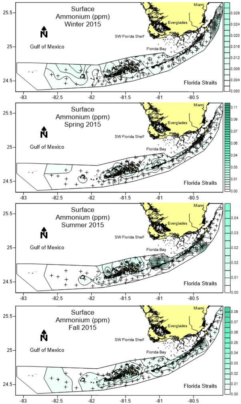
Figure 19. Surface ammonium distributions across the region during 2015.
