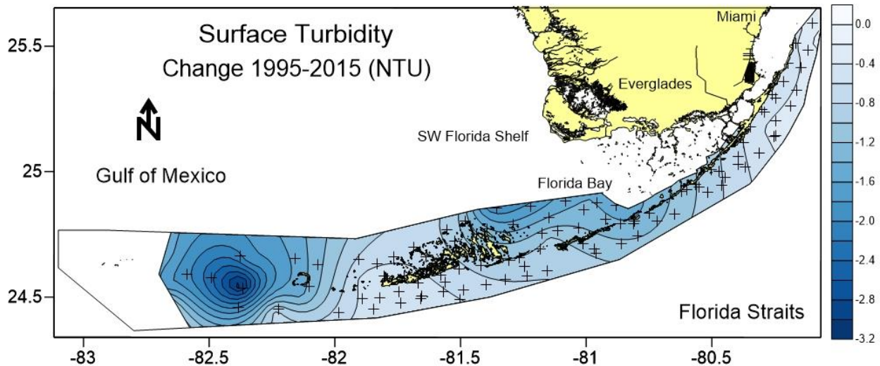
Figure iv. Total change in Turbidity in surface waters for 20 year period calculated from significant trends.
