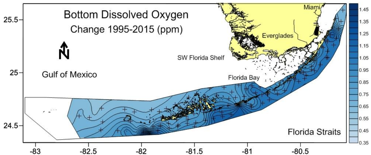
Figure 9. Total change in DO of bottom waters for 20 year period calculated from significant trends.
