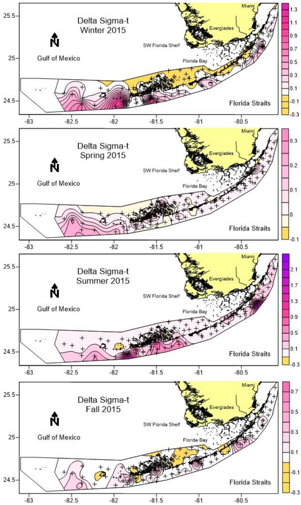
Figure 20. Surface and bottom density differences ( \Delta\sigma_t ) across the region during 2015.
