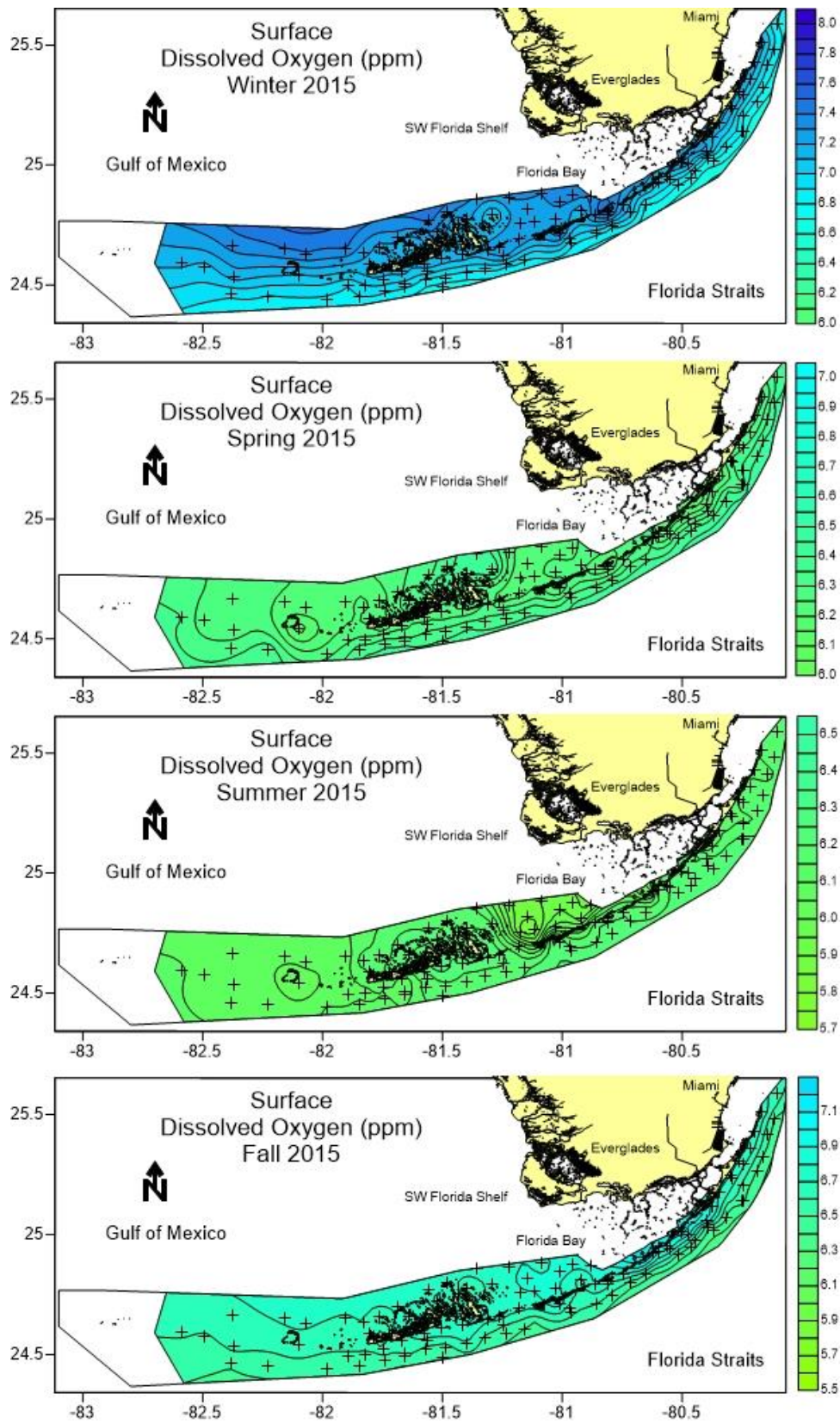
Figure 16. Surface dissolved oxygen distributions across the region during 2015.
