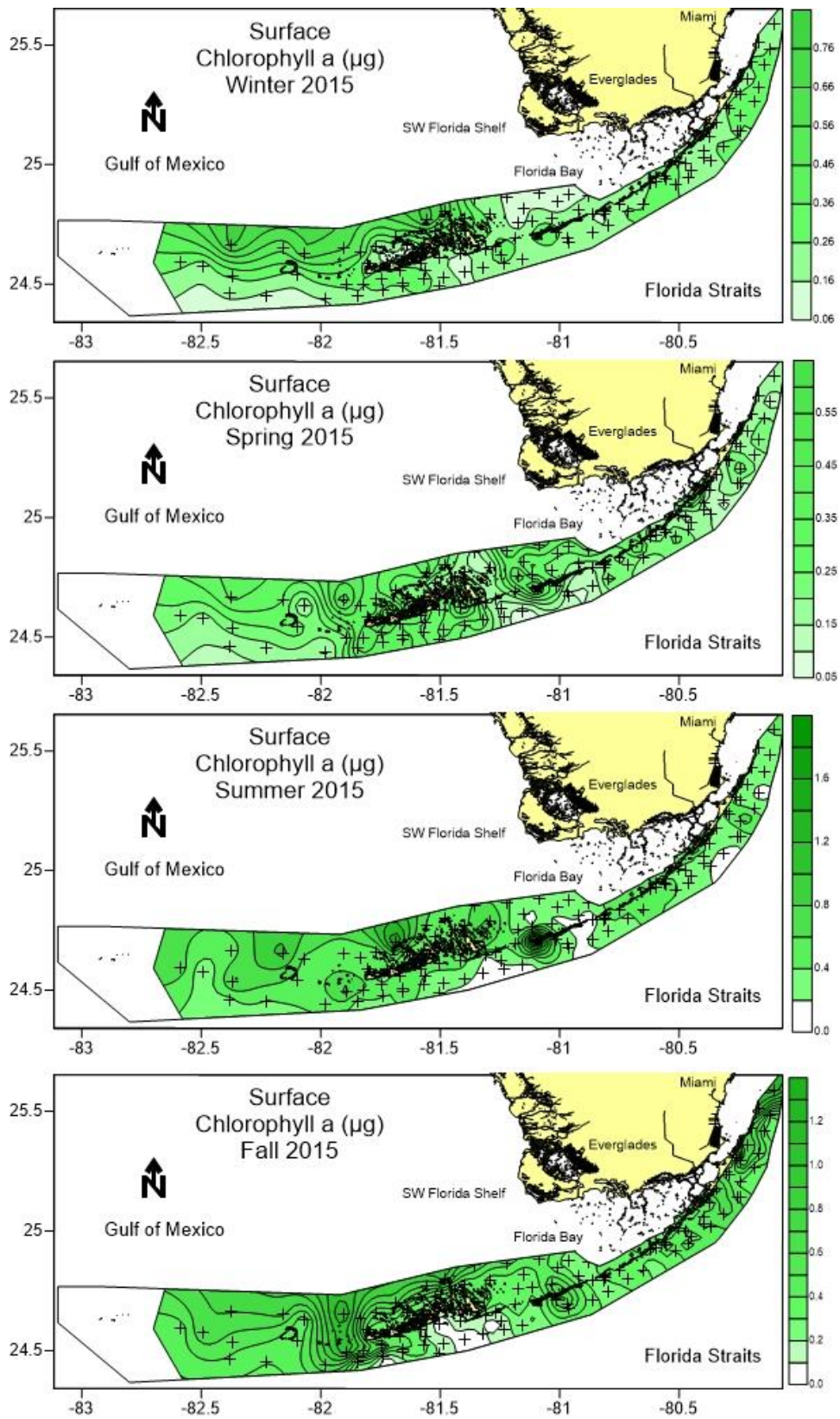
Figure 24. Distributions of surface chlorophyll a across the region during 2015.
