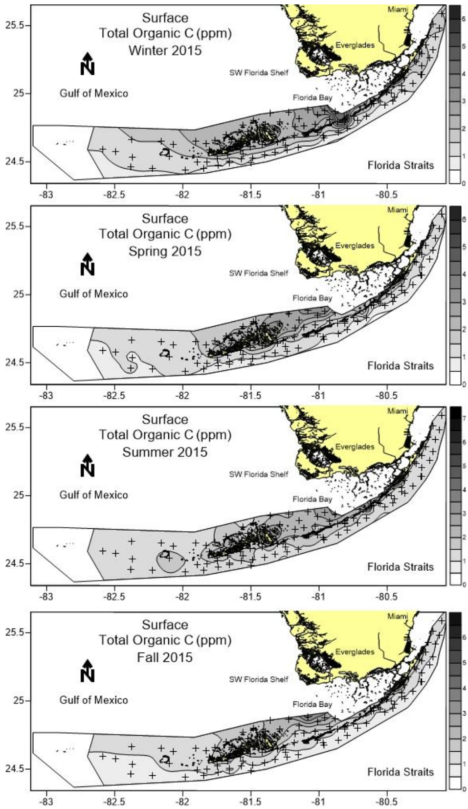
Figure 22. Distributions of surface total organic carbon across the region during 2015.
