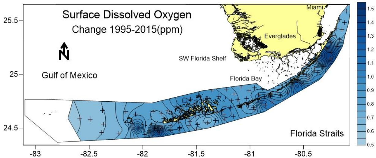
Figure ii. Total change in DO of surface waters for 20 year period calculated from significant trends.
