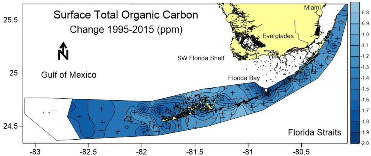
Figure vii. Total change in TOC in surface waters for 20 year period calculated from significant trends.
