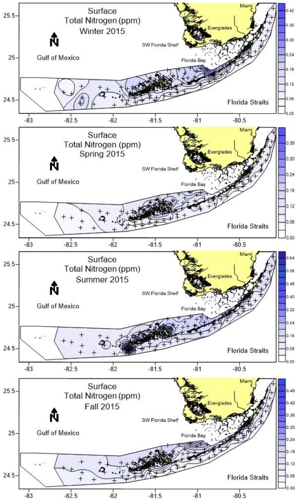
Figure 23. Distributions of surface total nitrogen across the region during 2015.
