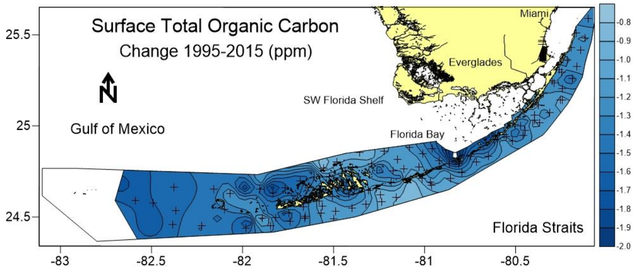
Figure 13. Total change in TOC in surface waters for 20 year period calculated from significant trends.
