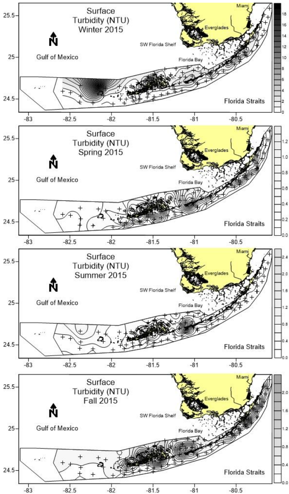
Figure 25. Distributions of surface turbidity across the region during 2015.
