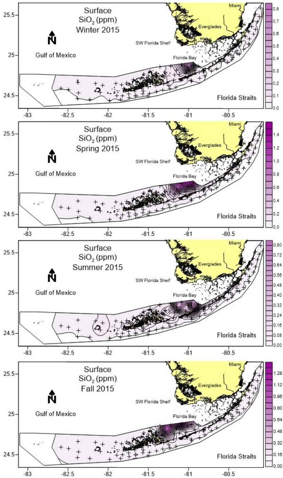
Figure 27. Distributions of surface silicate across the region during 2015.
