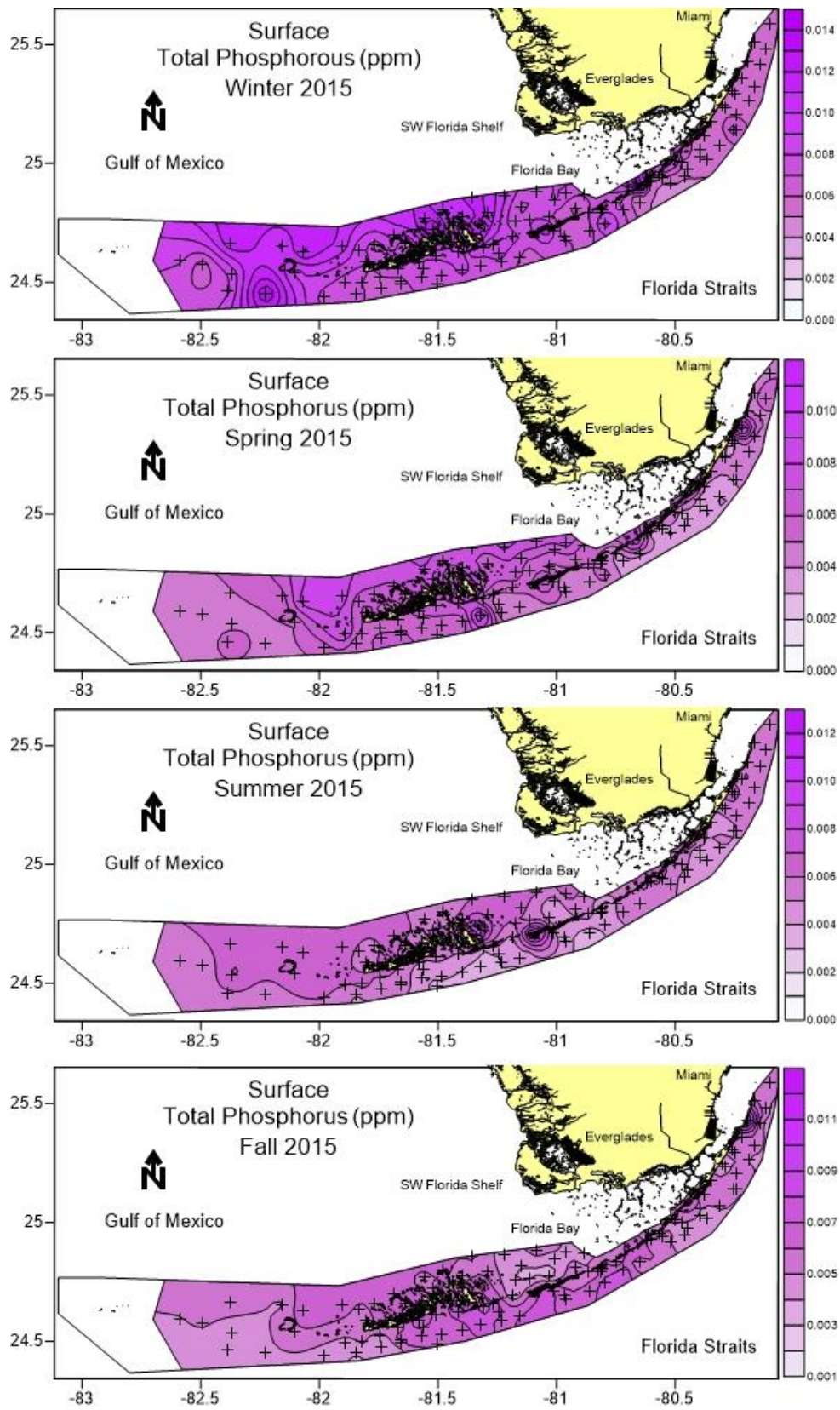
Figure 21. Distributions of surface total phosphorus across the region during 2015.
