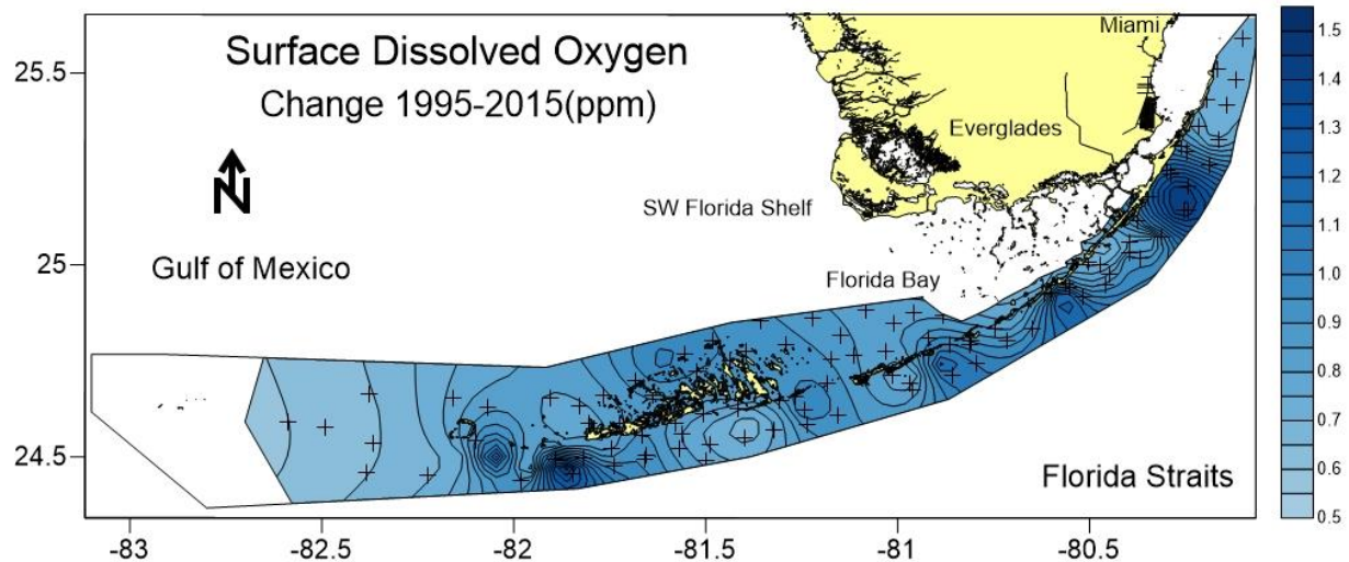
Figure 8. Total change in DO of surface waters for 20 year period calculated from significant trends.
