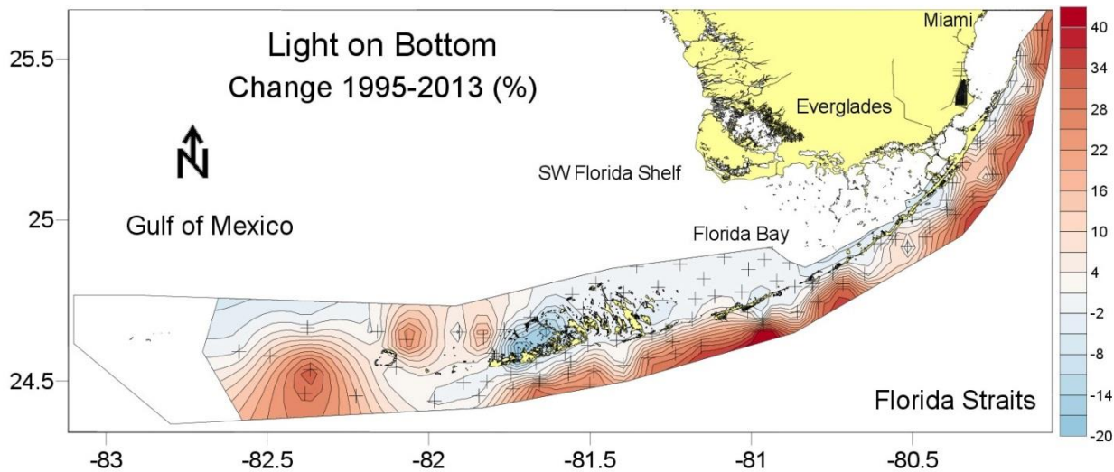
Figure v. Total change in bottom I_0 for 20 year period calculated from significant trends.
