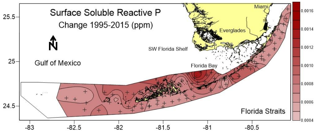
Figure vi. Total change in SRP in surface waters for 20 year period calculated from significant trends.
