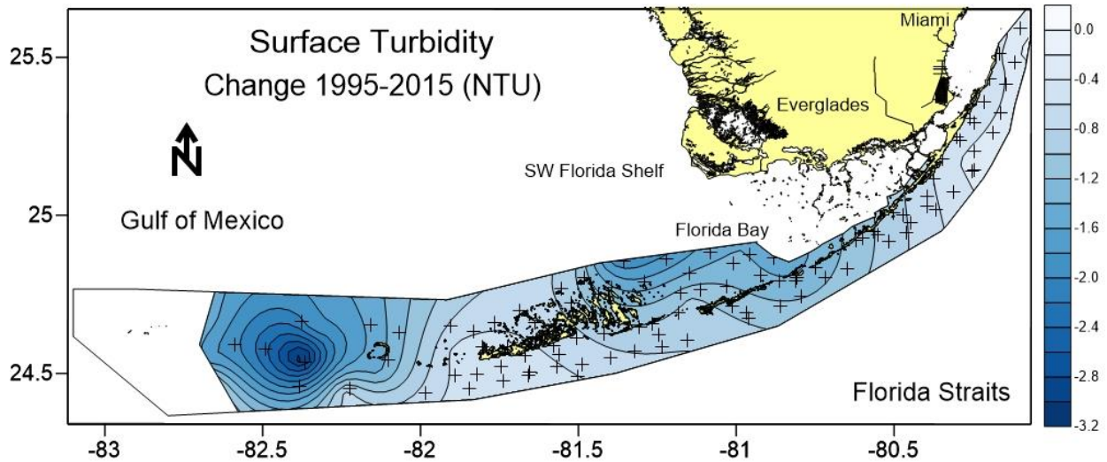
Figure 10. Total change in surface turbidity for 20 year period calculated from significant trends.
