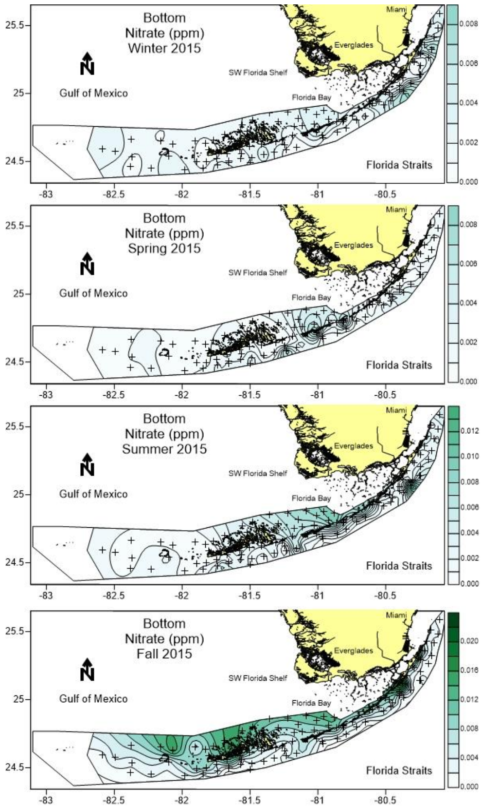
Figure 18. Bottom nitrate distributions across the region during 2015.
