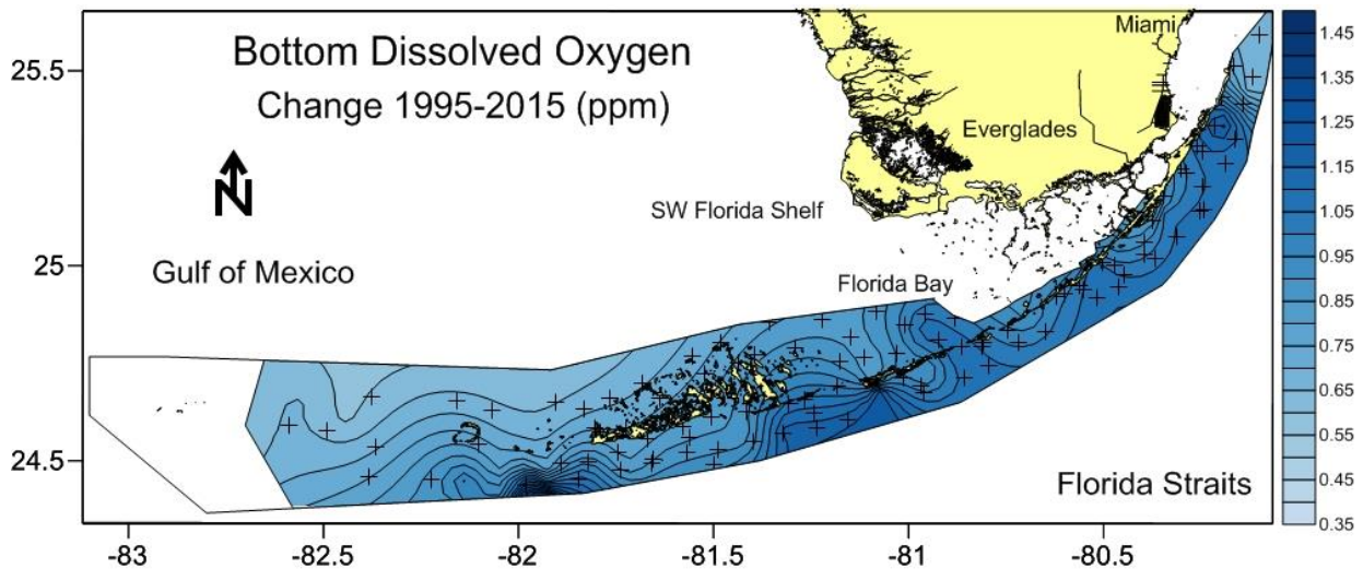
Figure iii. Total change in DO of bottom waters for 20 year period calculated from significant trends.
