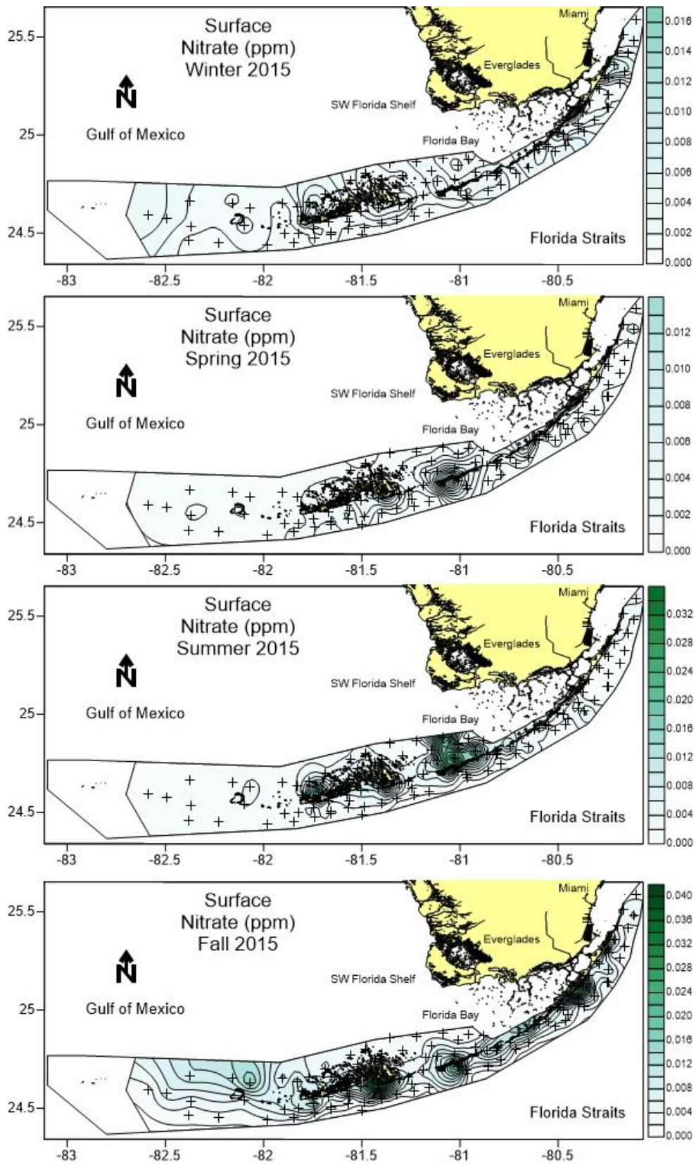
Figure 17. Surface nitrate distributions across the region during 2015.
