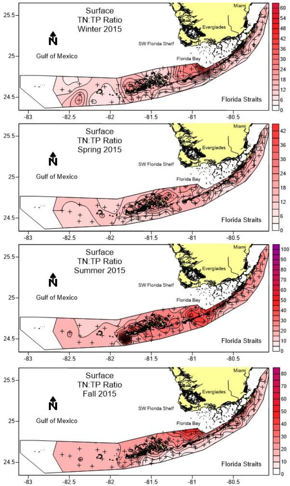
Figure 28. Distributions of surface TN:TP ratio across the region during FY2015.
