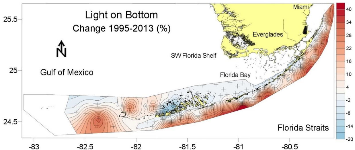
Figure 11. Total change in bottom I_o for 20 year period calculated from significant trends.
