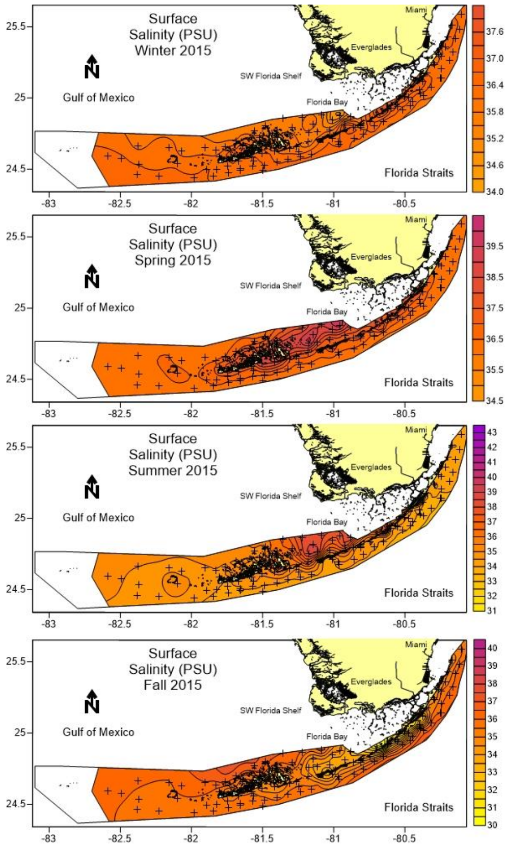
Figure 15. Surface salinity distributions across the region during 2015.
