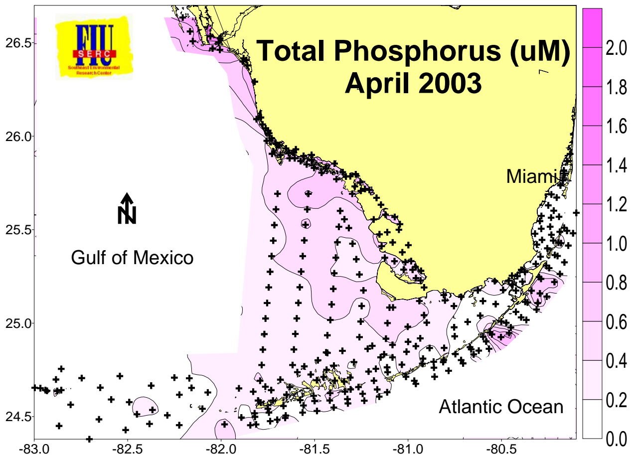
Figure 13. Example of total phosphorus distributions across the region during spring 2003.
