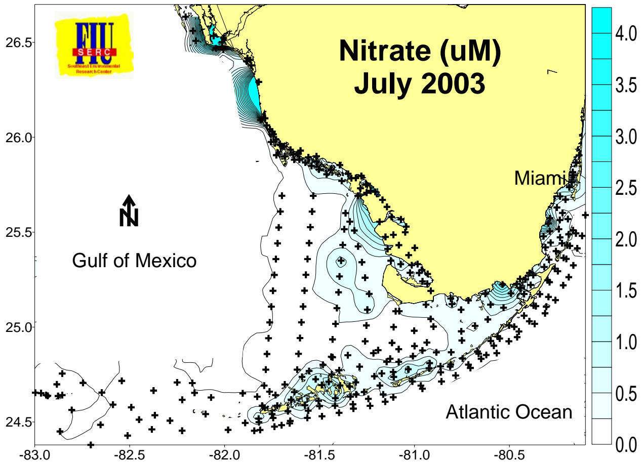
Figure 12. Example of nitrate distributions across the region during summer 2003.
