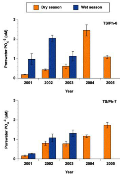
Figure 2-10. Porewater SRP concentrations (mean \pm SE) in mangrove forest soils at TS/Ph-6 and 7.
