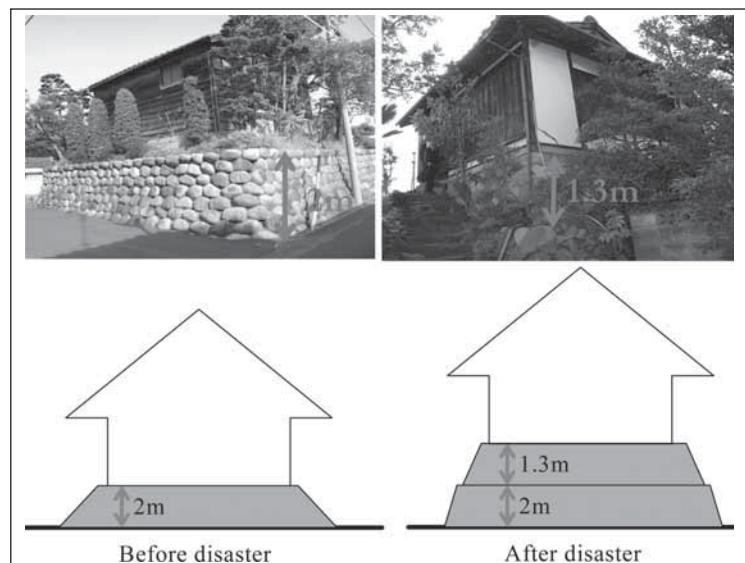
Figure 6. The Mizuya's plinth height was increased after the 1896 flood disaster (Photo by NIED-KU, 2007)
