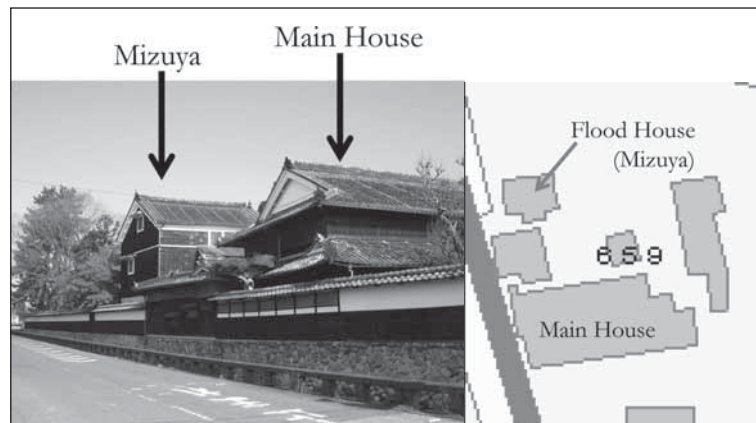
Figure 5. Mizuya, the flood house (Photo by NIED-KU, 2007)
