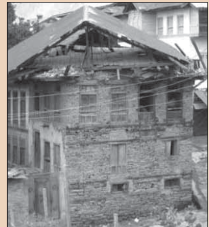
Figure 3. a) Portions where Dhajji-Dewari system (gable portion) and b) Taq system (entire structure except gable portion) survived the destruction of the 2005 earthquake.
