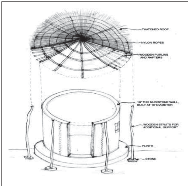
Figure 1. A diagram of the dhani
