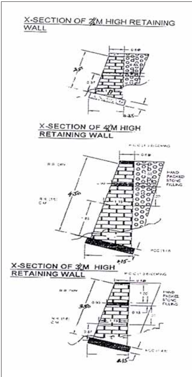
Figure 4. Specifications of retaining wall against landslides
