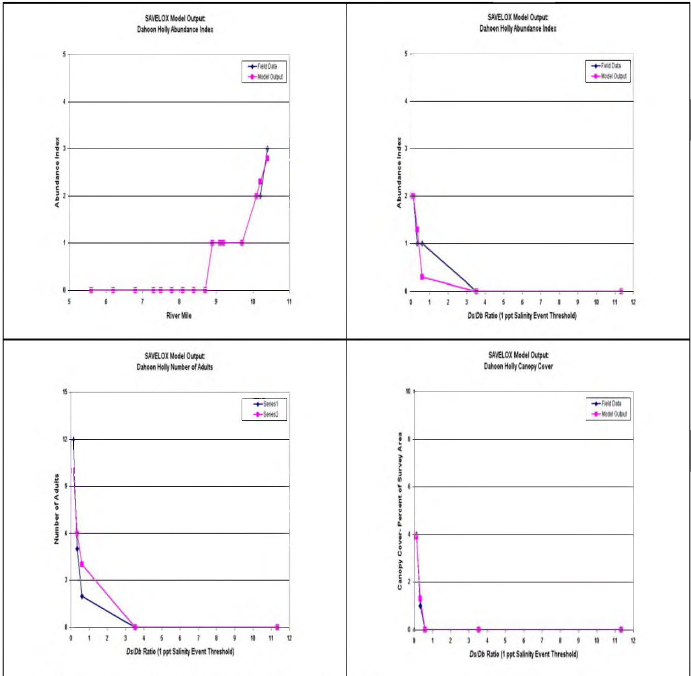
Figure D-3. Comparison of Field Data with Model Output for Dahoon Holly.
