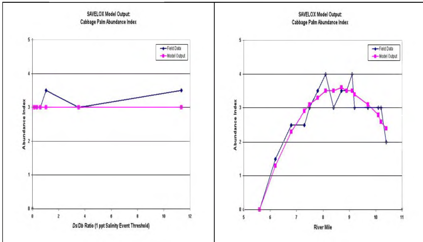
Figure D-2. Comparison of Field Data with Model Output for Cabbage Palm.
