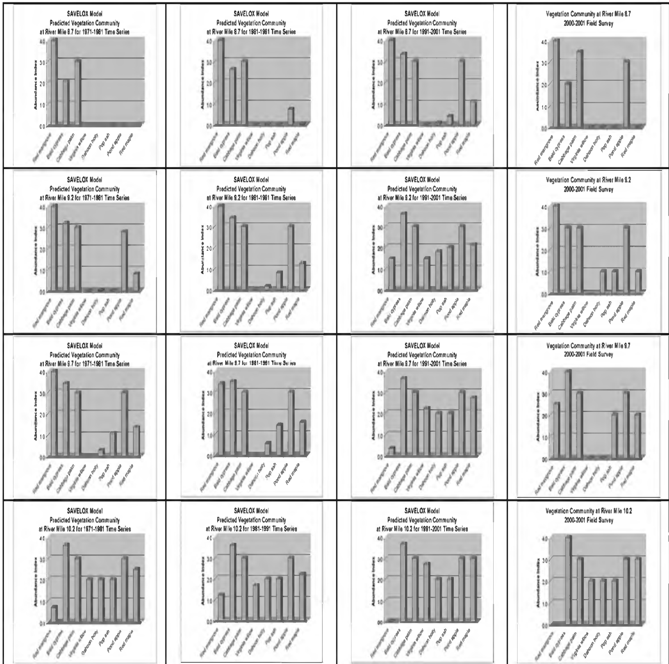
Figure 22. SAVeLOX Model Output for Three Decades and Vegetation Survey Results (see Figure 10 for Abundance Index).
