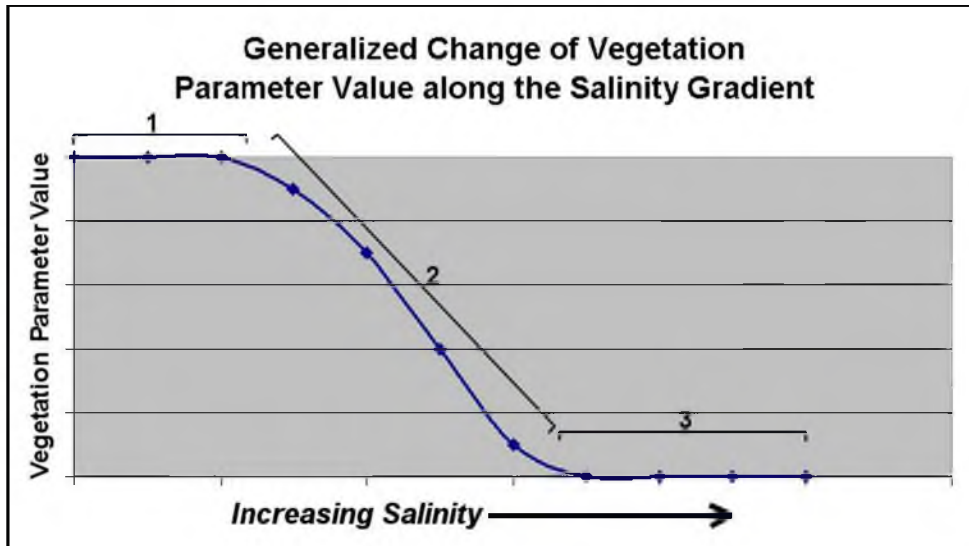
Figure 12. Generalized Pattern of Change in a Freshwater Species Vegetation Parameter Value along the Salinity Gradient of the Northwest Fork.
