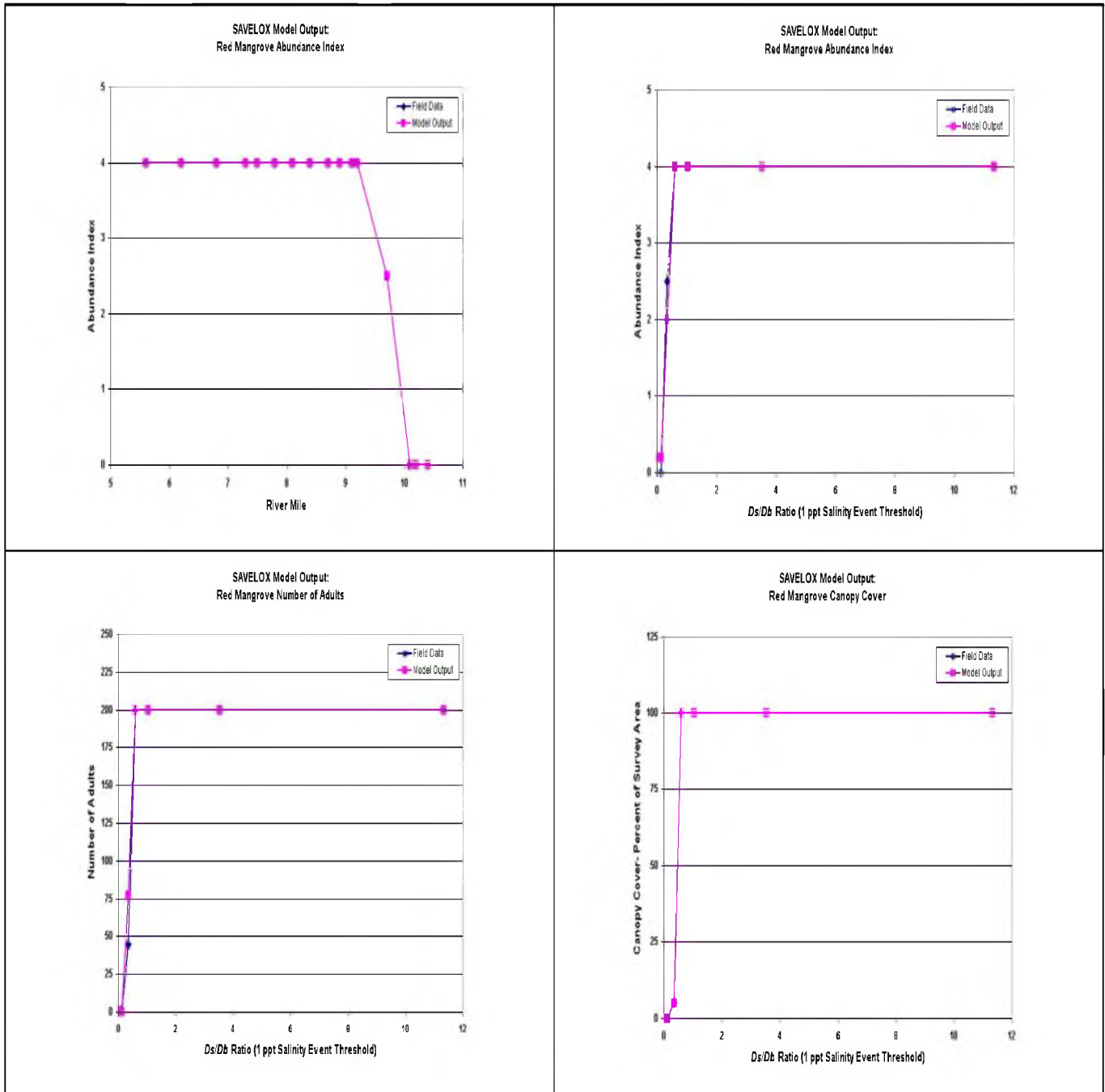
Figure D-6. Comparison of Field Data with Model Output for Red Mangrove.
