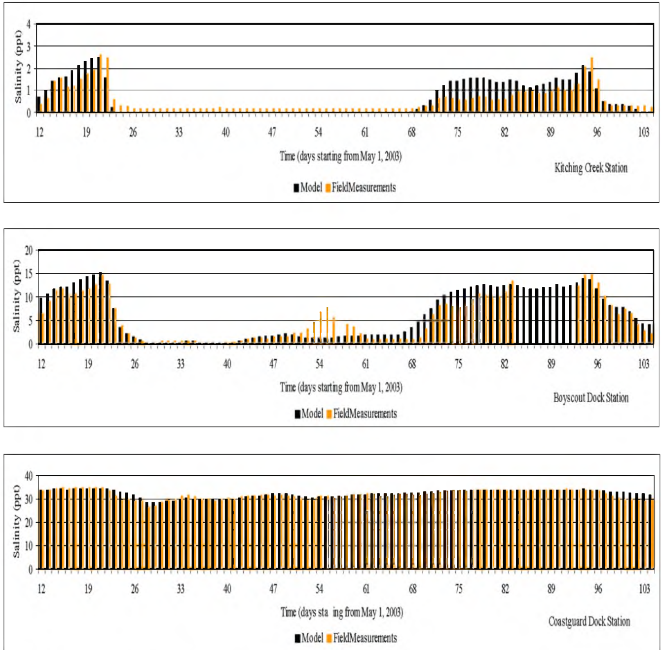
Figure A-18. Daily Average Salinity Based on Model Output and Field Measurements.
