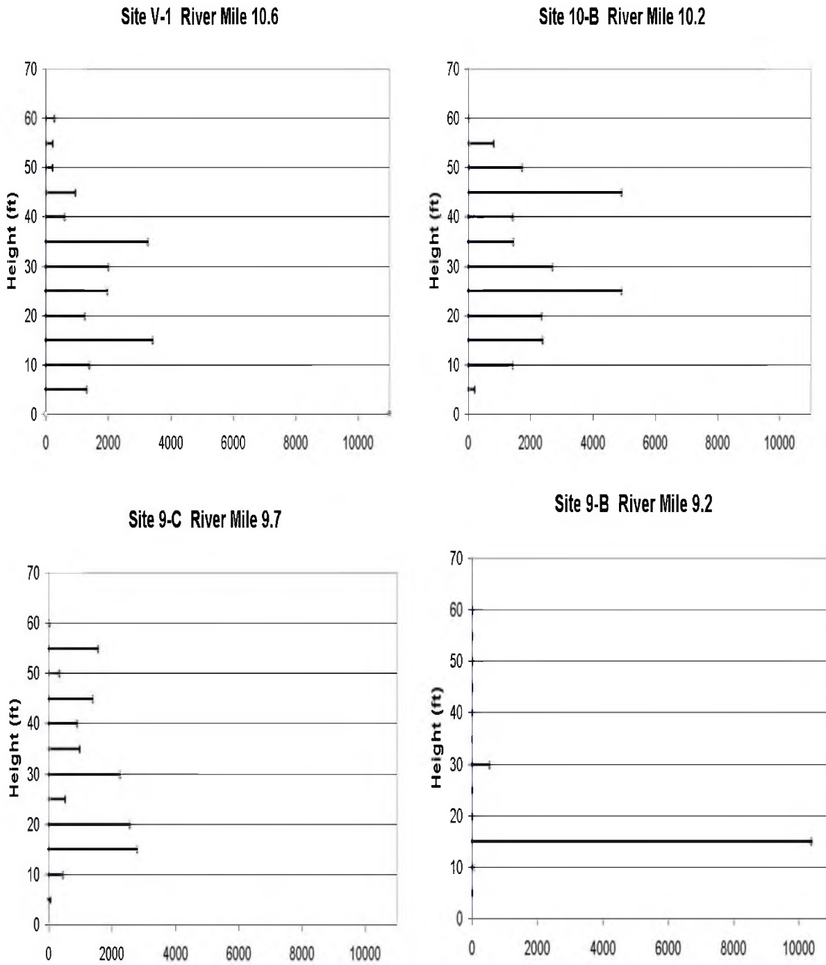
Figure 20. Total Forest Canopy Area within Height Classes for four sites along the Northwest Fork of the Loxahatchee River. Values are Canopy Area (ft 2 ).
