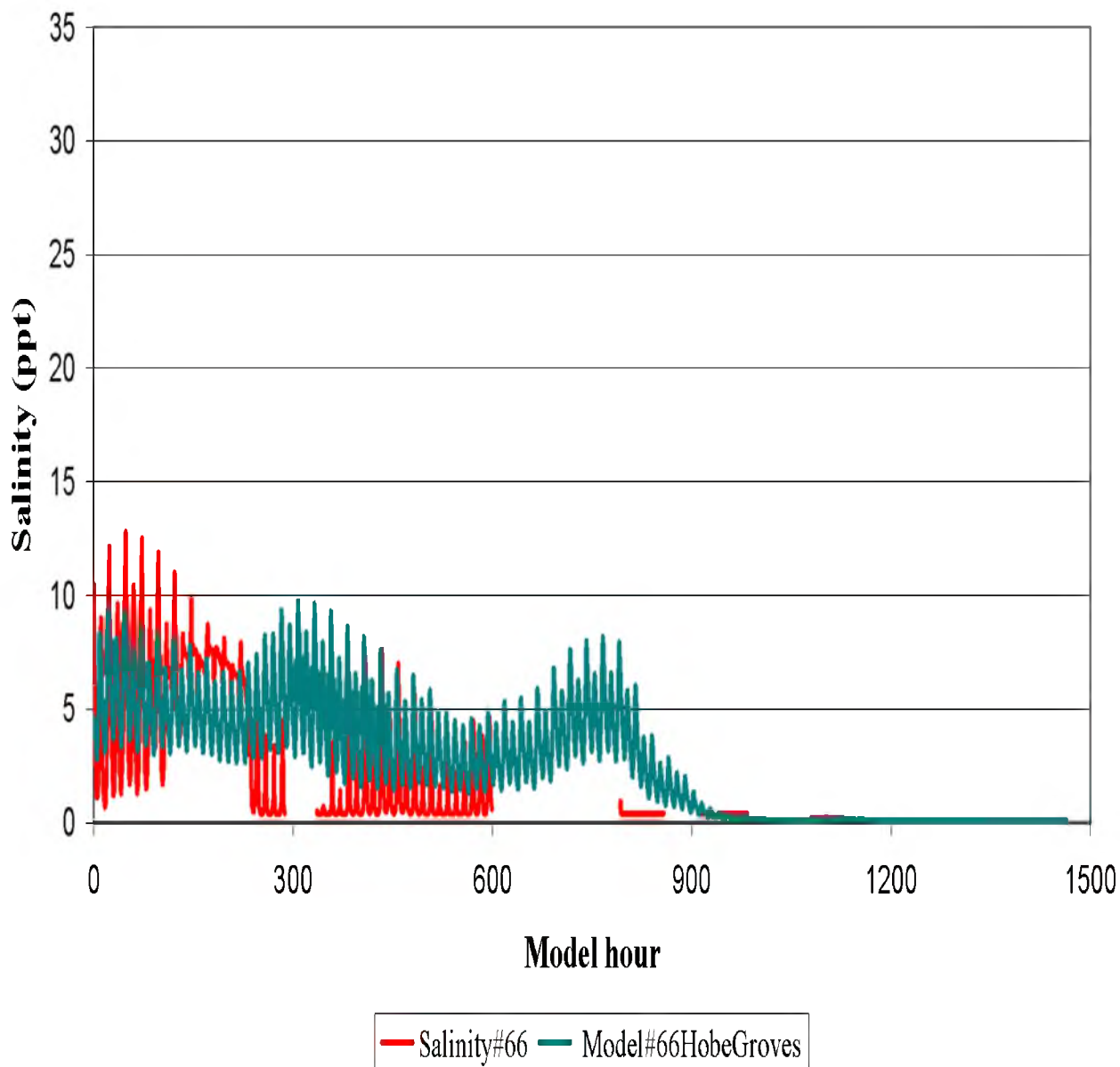
Figure A-5. Comparison of Model Output and Field Record at Station 66 (RM 9.4).
