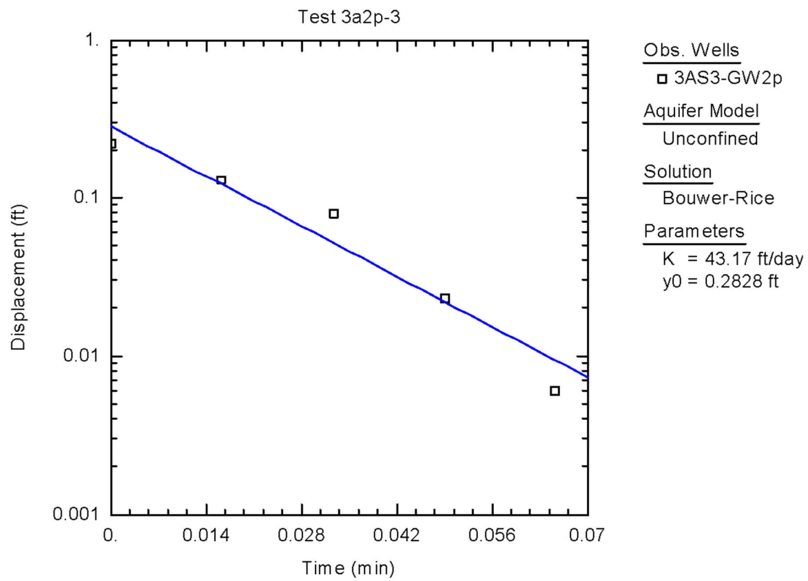
Figure C-7. Graphical Representation of Raw Data Obtained from Slug Test of 3AS3-GW2p, Bouwer-Rice Solution
