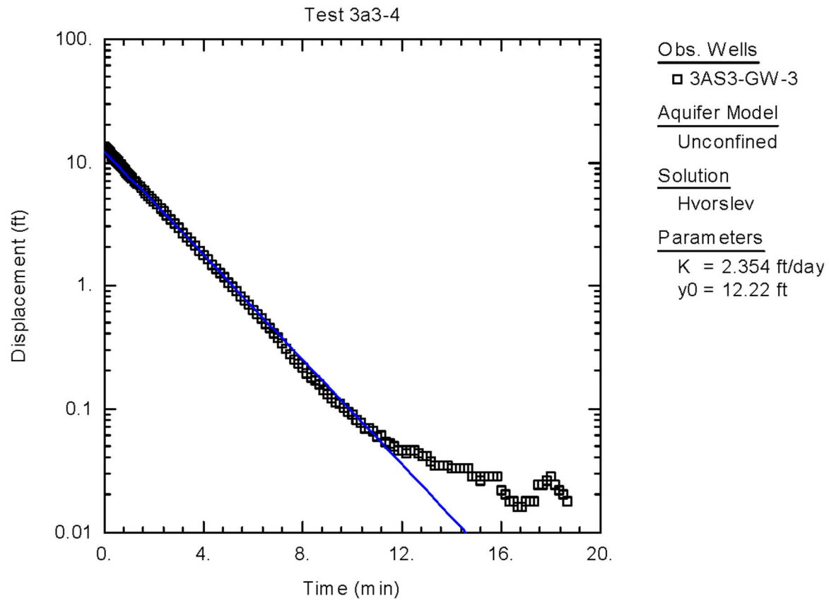
Figure C-10. Graphical Representation of Raw Data Obtained from Slug Test of 3AS3-GW3, Hvorslev Solution
