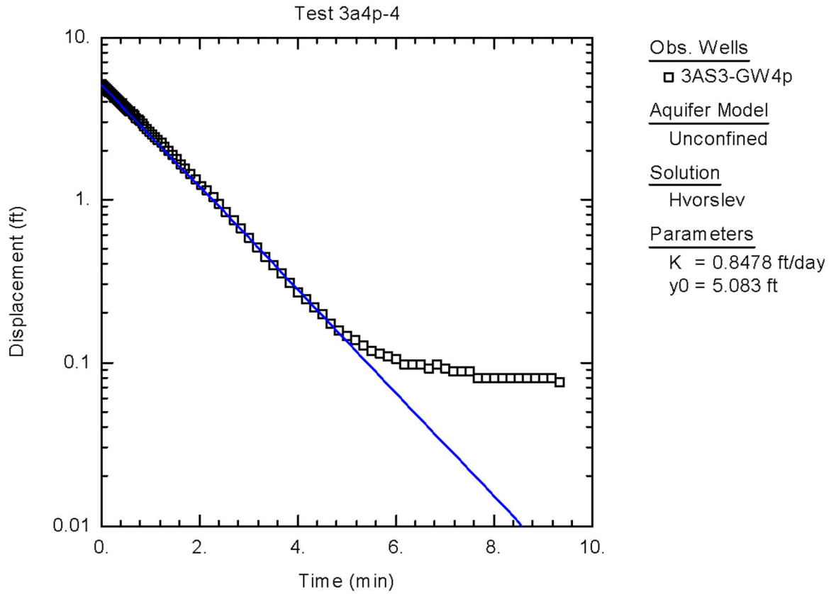
Figure C-16. Graphical Representation of Raw Data Obtained from Slug Test of 3AS3-GW4p, Hvorslev Solution
