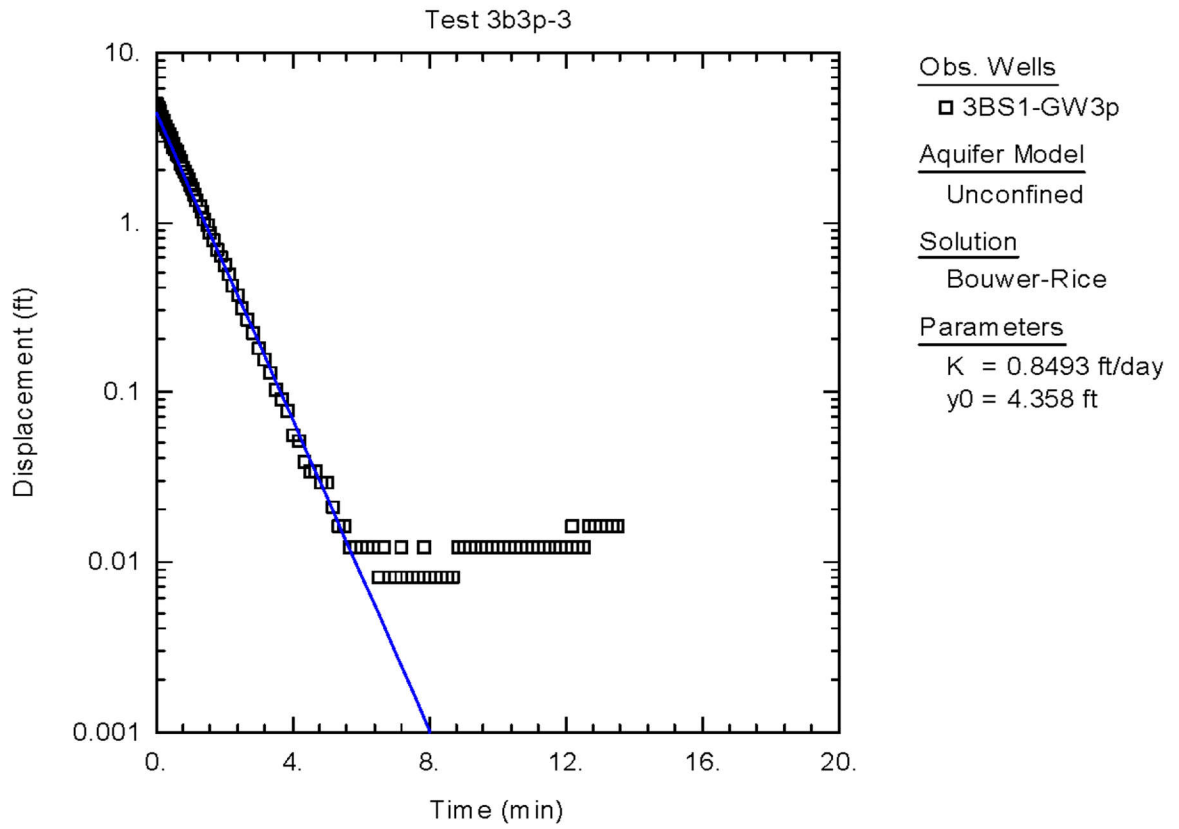
Figure C-19. Graphical Representation of Raw Data Obtained from Slug Test of 3BS1-GW3p, Bower-Rice Solution
