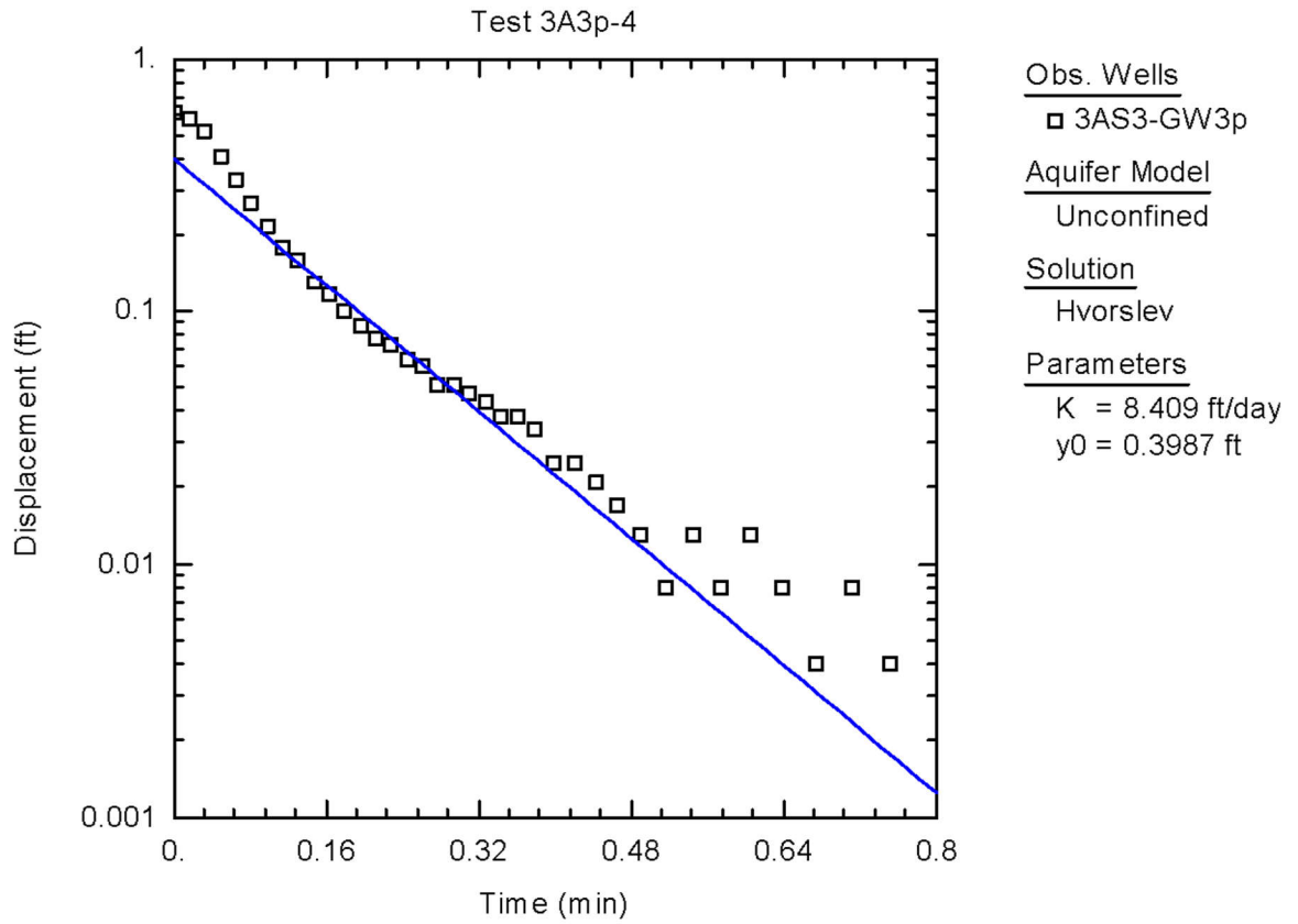
Figure C-12. Graphical Representation of Raw Data Obtained from Slug Test of 3AS3-GW3p, Hvorslev Solution
