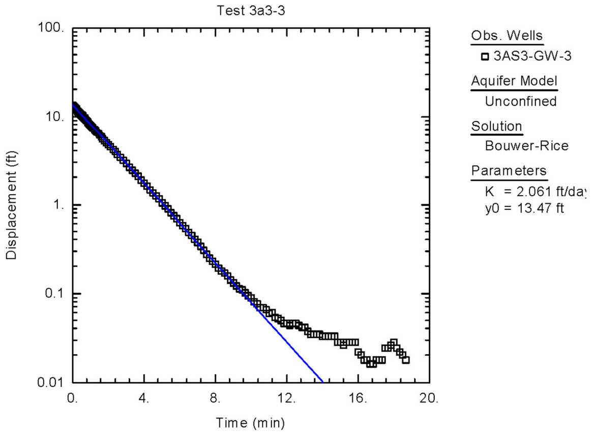
Figure C-9. Graphical Representation of Raw Data Obtained from Slug Test of 3AS3-GW3, Bouwer-Rice Solution
