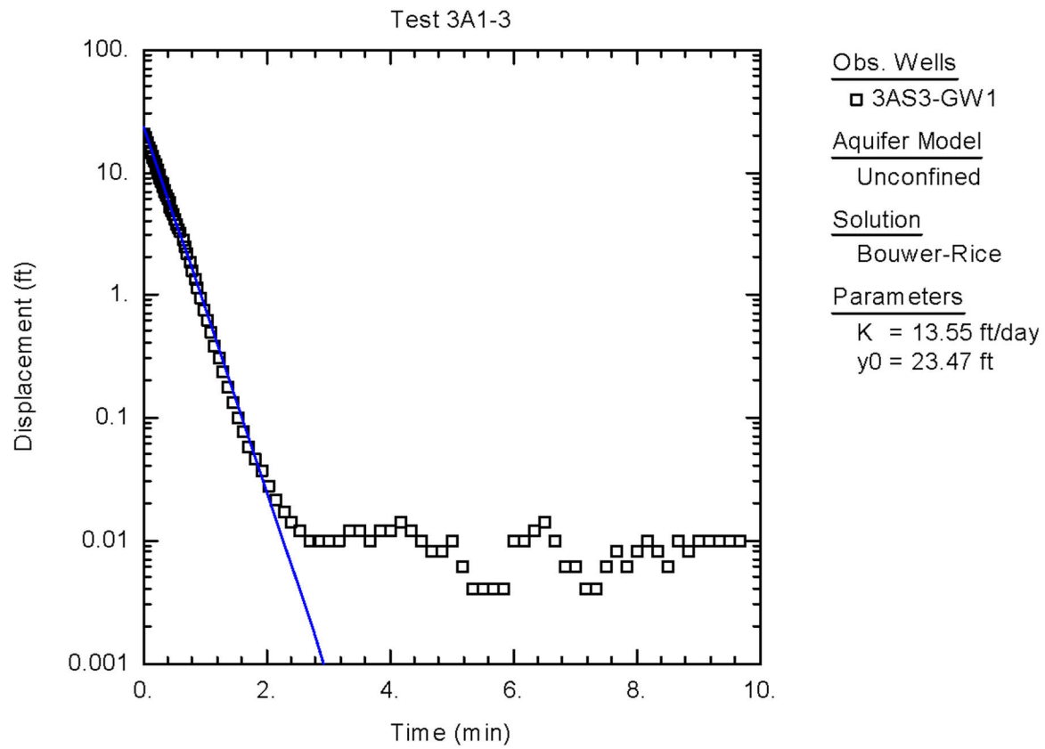
Figure C-1. Graphical Representation of Raw Data Obtained from Slug Test of 3AS3-GW1, Bouwer-Rice Solution
