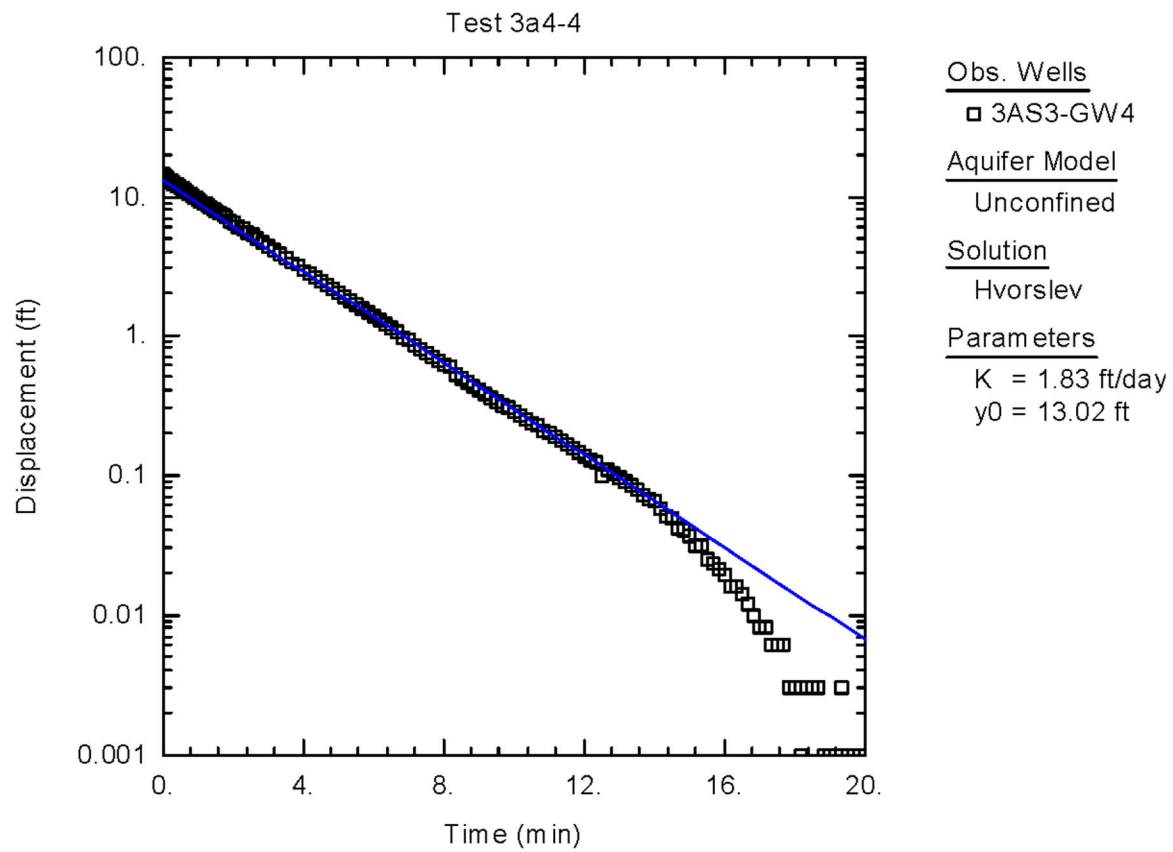
Figure C-14. Graphical Representation of Raw Data Obtained from Slug Test of 3AS3-GW4, Hvorslev Solution
