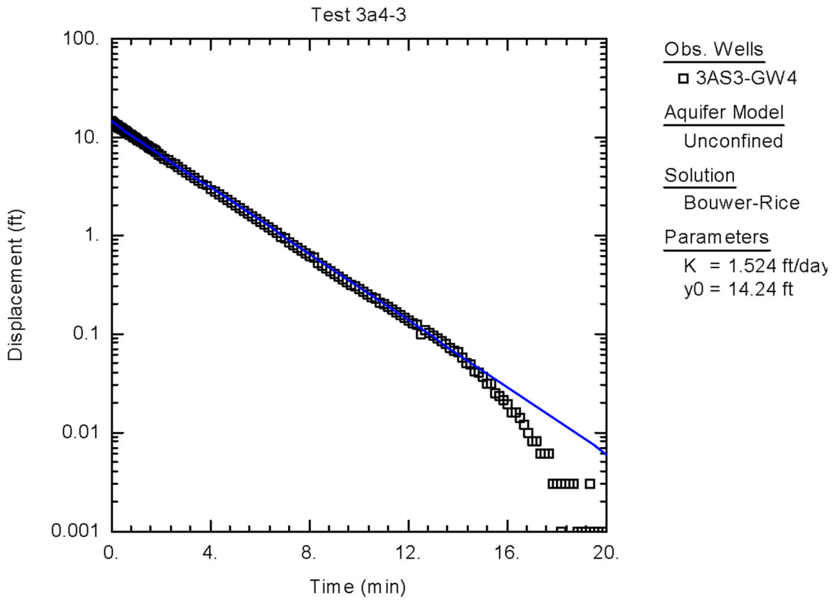
Figure C-13. Graphical Representation of Raw Data Obtained from Slug Test of 3AS3-GW4, Bouwer-Rice Solution
