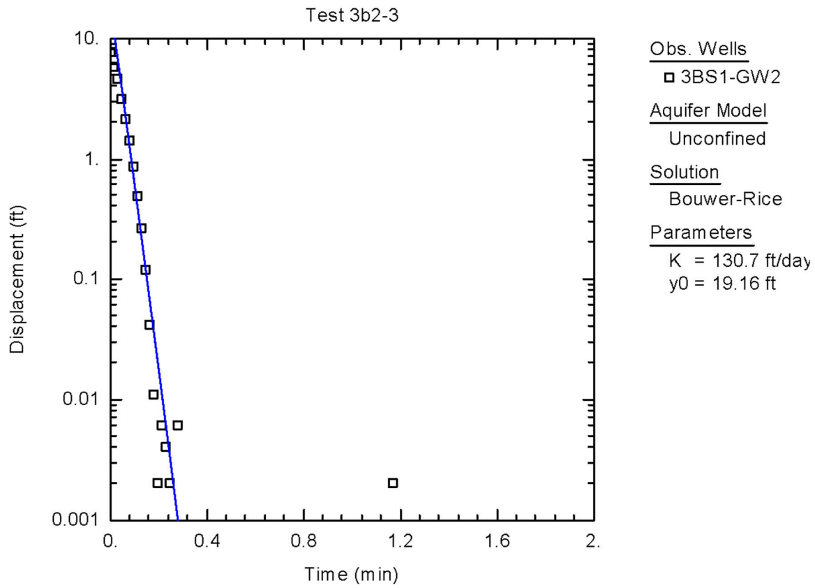
Figure C-17. Graphical Representation of Raw Data Obtained from Slug Test of 3BS1-GW2, Bouwer-Rice Solution
