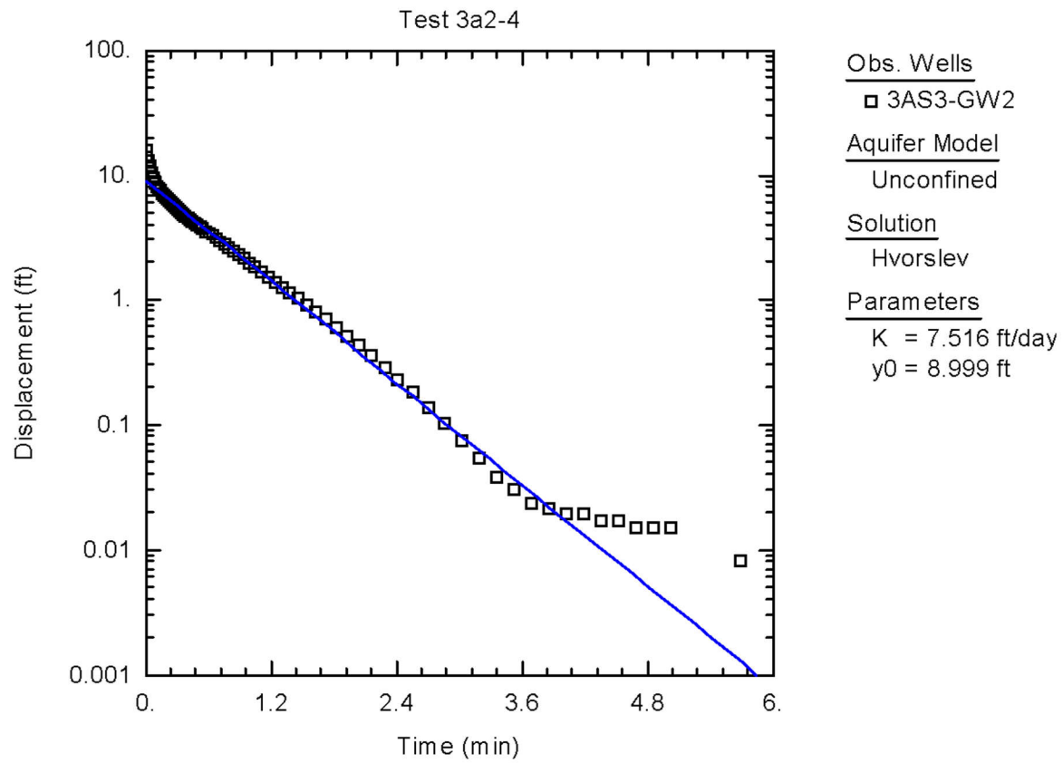
Figure C-6. Graphical Representation of Raw Data Obtained from Slug Test of 3AS3-GW2, Hvorslev Solution
