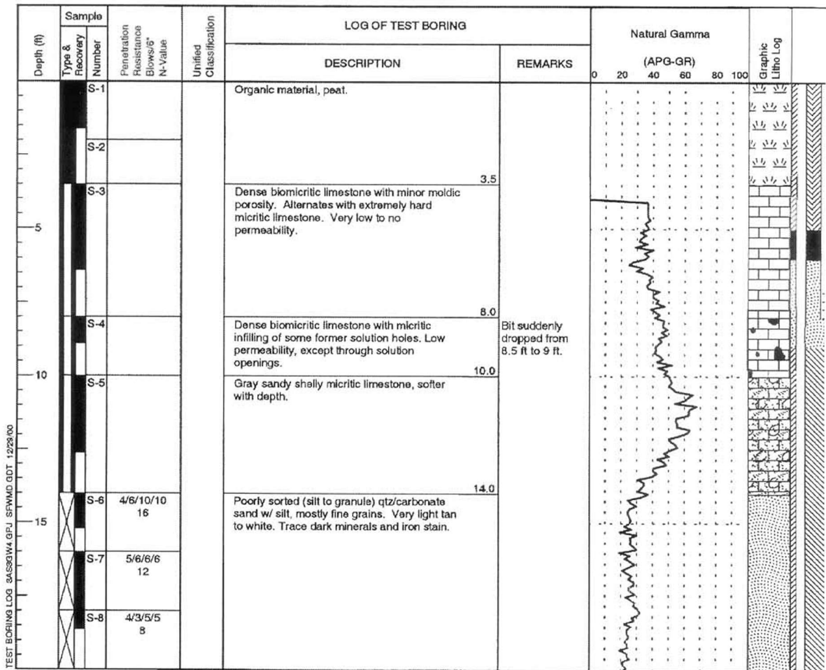
Figure B-22. Test Boring Log for Well 3AS3-GW4 (Sheet 1 of 2)
