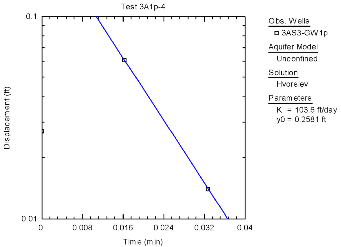
Figure C-4. Graphical Representation of Raw Data Obtained from Slug Test of 3AS3-GW1p, Hvorslev Solution
