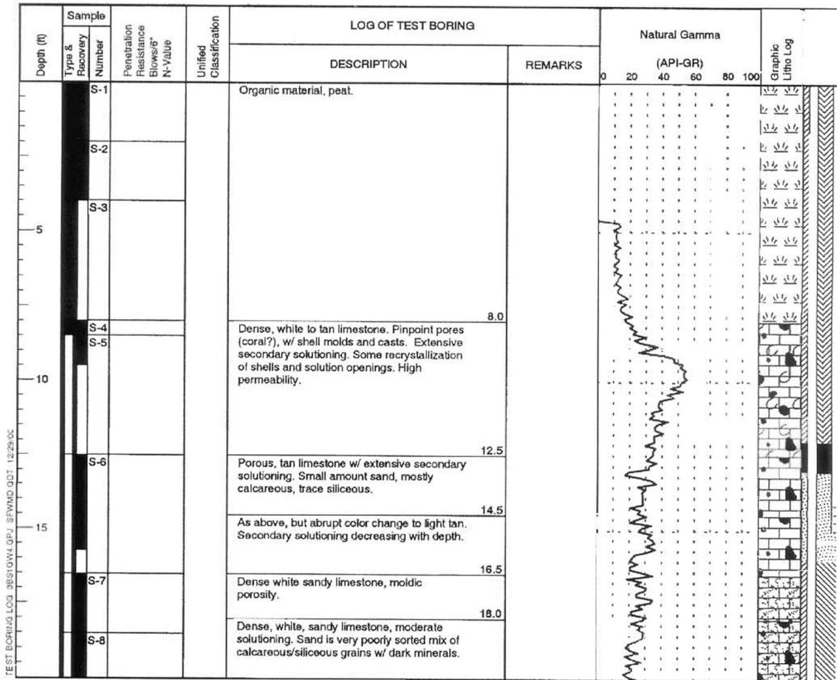
Figure B-30. Test Boring Log for Well 3BS1-GW4 (Sheet 1 of 2)
