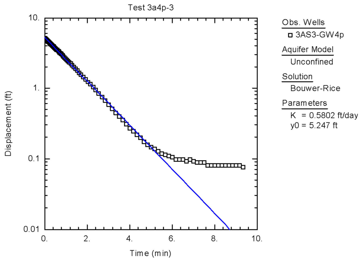
Figure C-15. Graphical Representation of Raw Data Obtained from Slug Test of 3AS3-GW4p, Bouwer-Rice Solution
