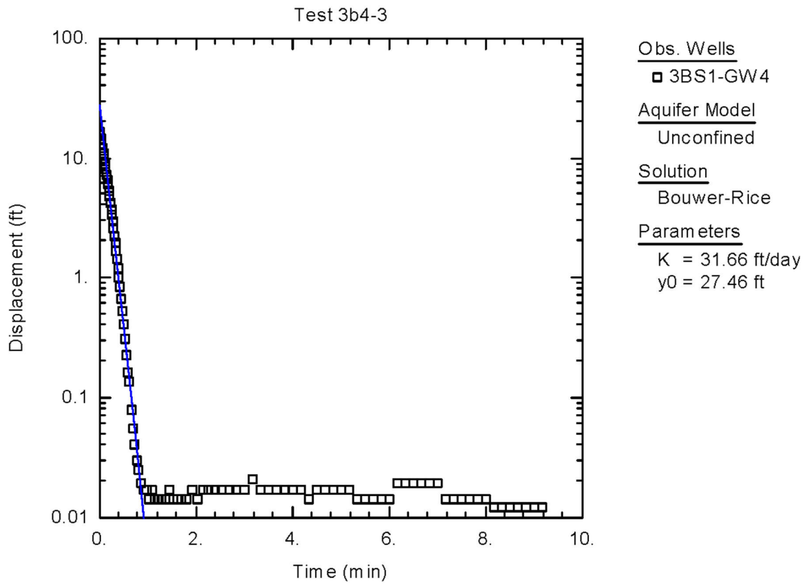
Figure C-21. Graphical Representation of Raw Data Obtained from Slug Test of 3BS1-GW4, Bouwer-Rice Solution
