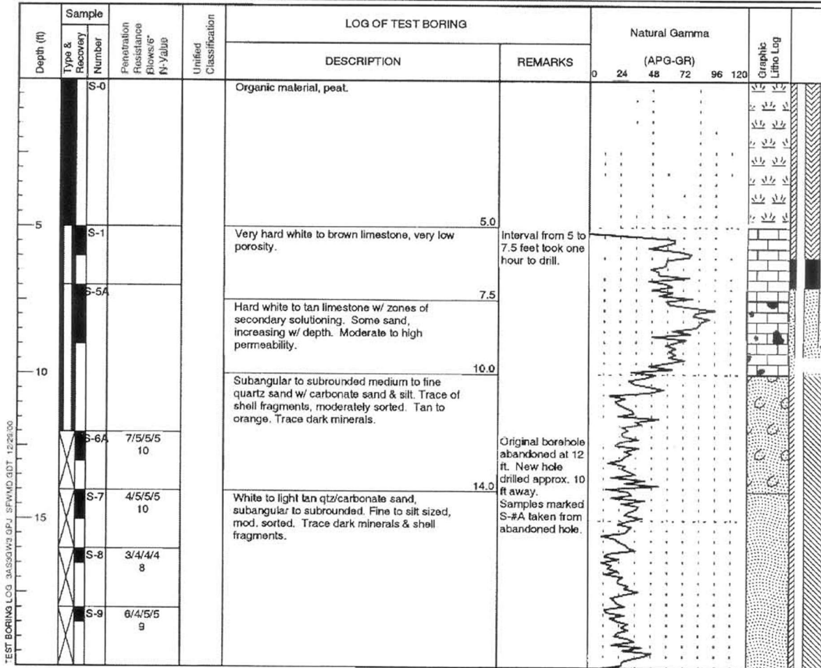
Figure B-20. Test Boring Log for Well 3AS3-GW3 (Sheet 1 of 2)
