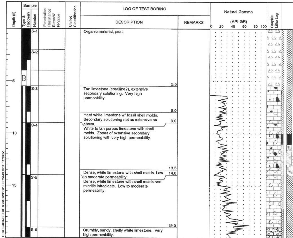
Figure B-26. Test Boring Log for Well 3BS1-GW2 (Sheet 1 of 2)
