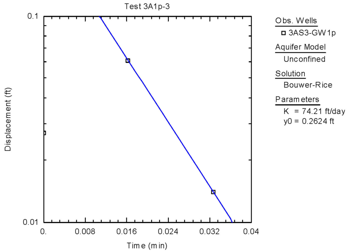
Figure C-3. Graphical Representation of Raw Data Obtained from Slug Test of 3AS3-GW1p, Bouwer-Rice Solution
