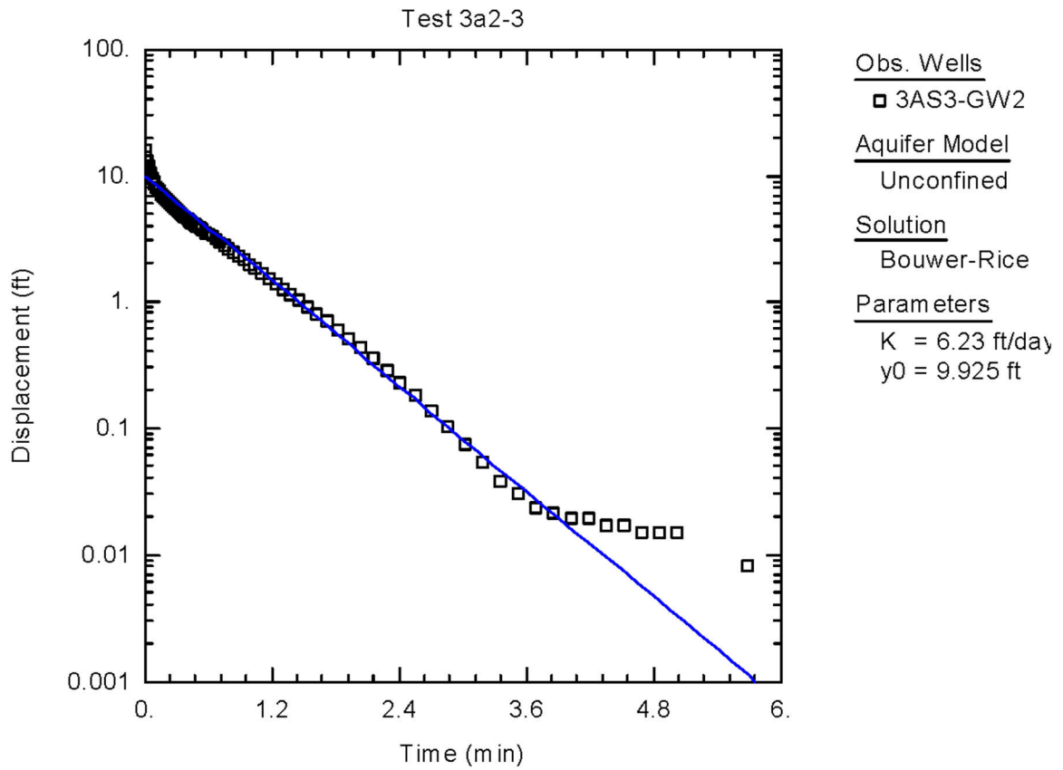
Figure C-5. Graphical Representation of Raw Data Obtained from Slug Test of 3AS3-GW2, Bouwer-Rice Solution
