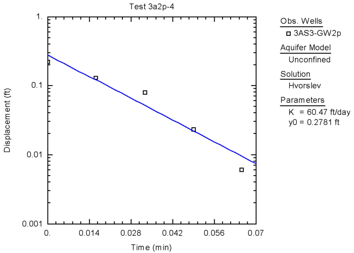
Figure C-8. Graphical Representation of Raw Data Obtained from Slug Test of 3AS3-GW2p, Hvorslev Solution
