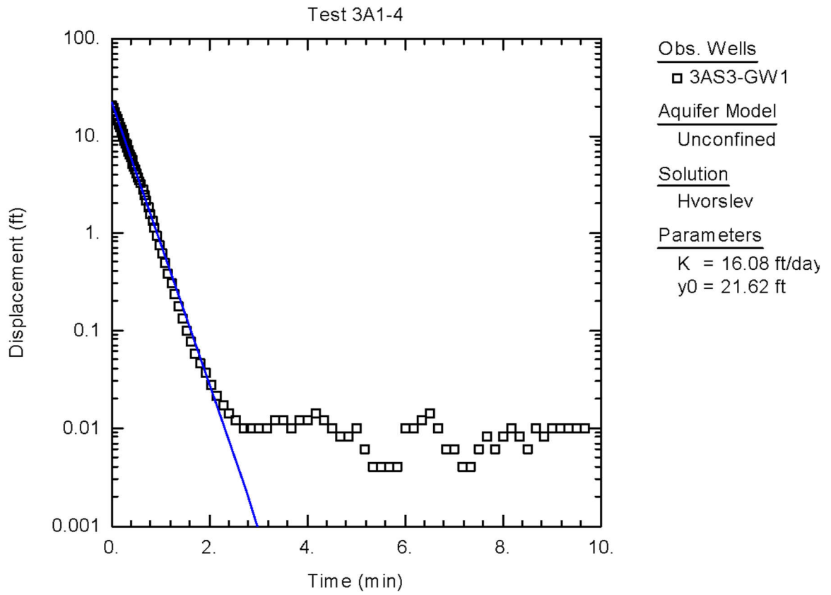
Figure C-2. Graphical Representation of Raw Data Obtained from Slug Test of 3AS3-GW1, Hvorslev Solution
