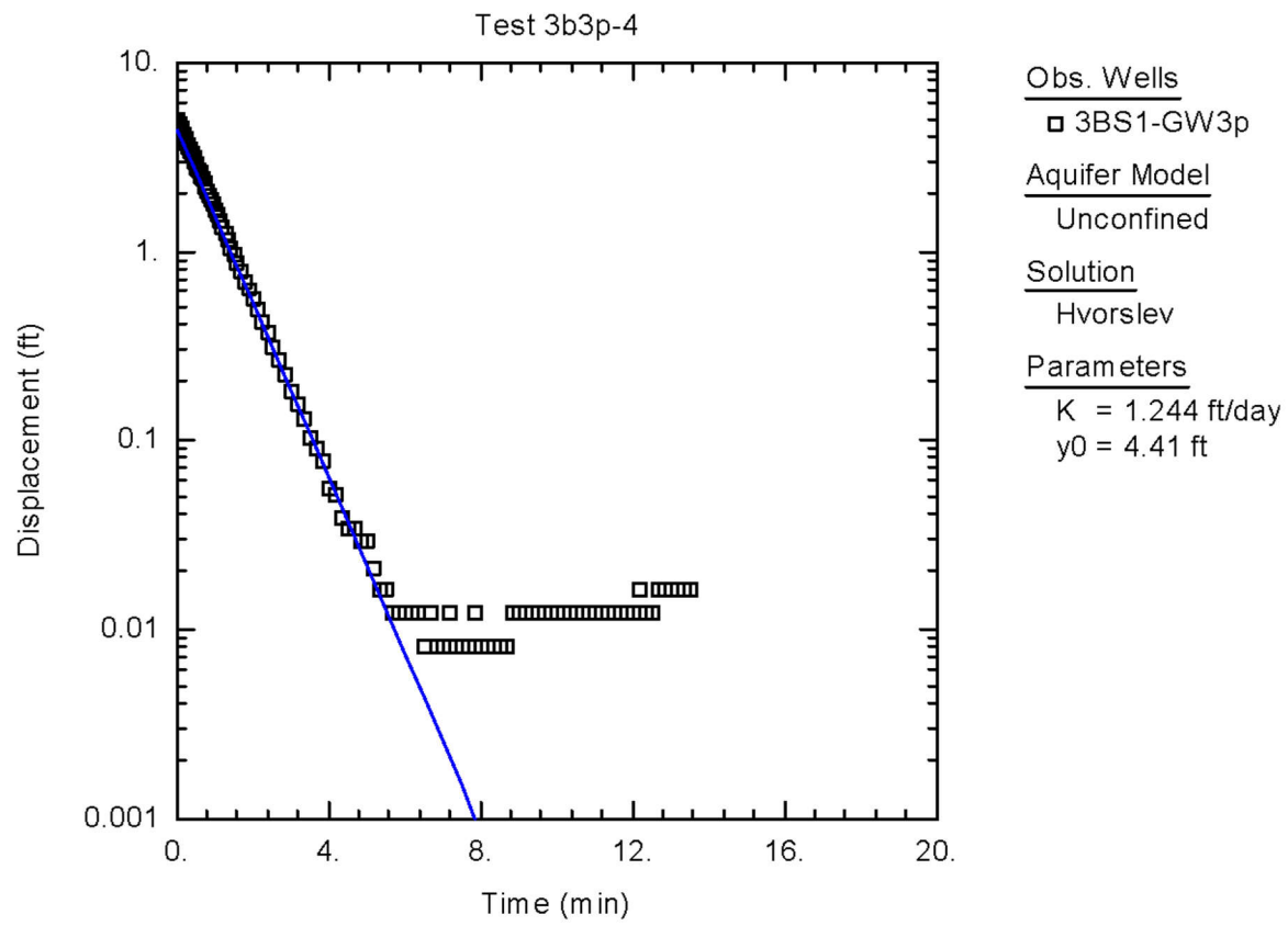
Figure C-20. Graphical Representation of Raw Data Obtained from Slug Test of 3BS1-GW3p, Hvorslev Solution
