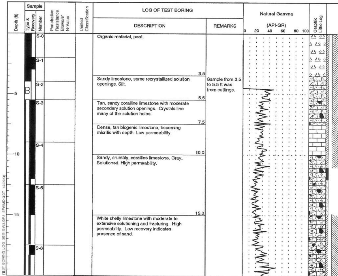
Figure B-28. Test Boring Log for Well 3BS1-GW3 (Sheet 1 of 2)
