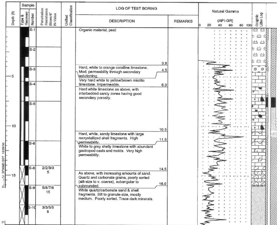
Figure B-16. Test Boring Log for Well 3AS3-GW1 (Sheet 1 of 2)
