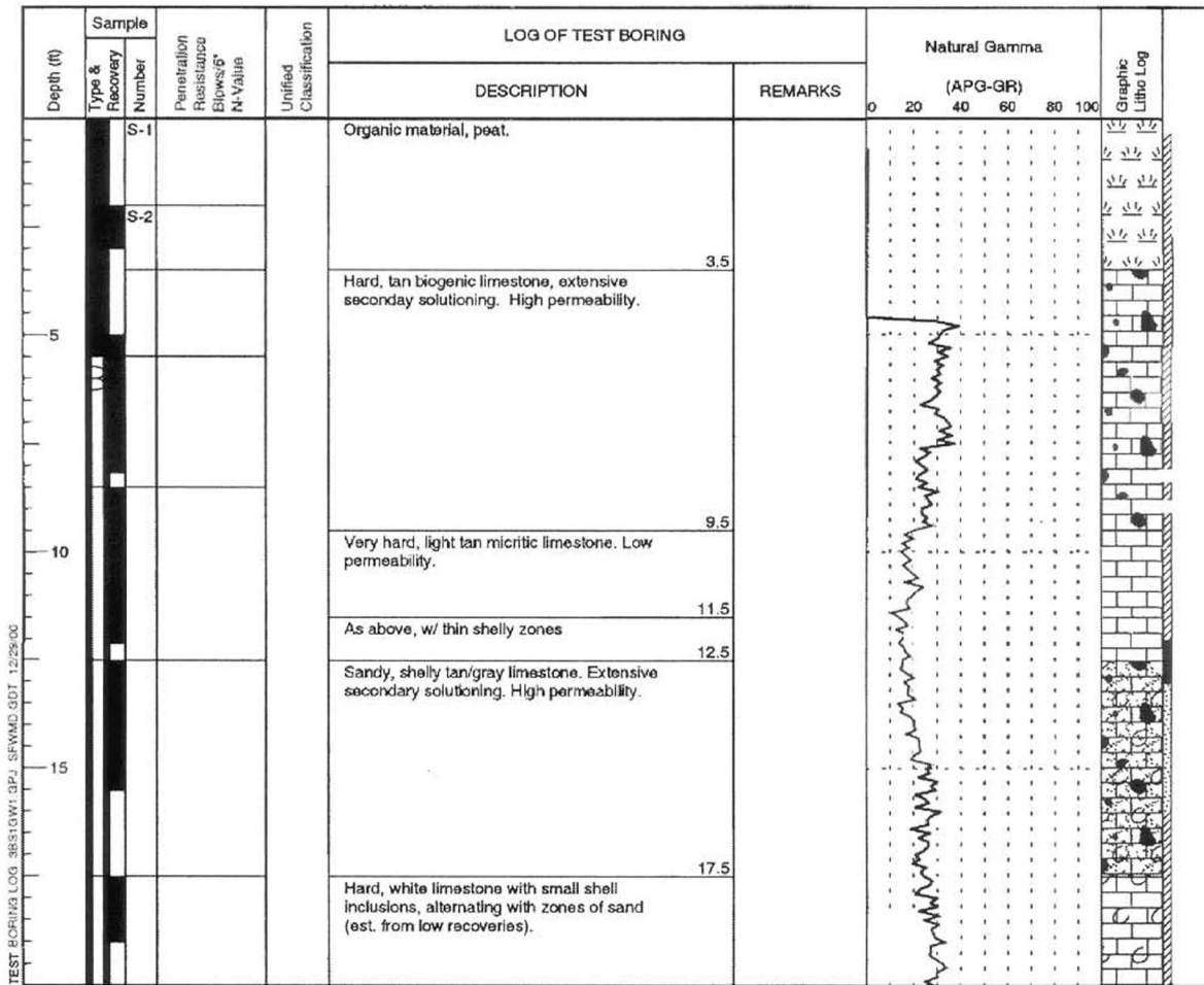
Figure B-24. Test Boring Log for Well 3BS1-GW1 (Sheet 1 of 2)
