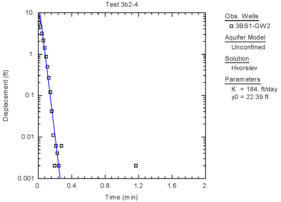
Figure C-18. Graphical Representation of Raw Data Obtained from Slug Test of 3BS1-GW2, Hvorslev Solution
