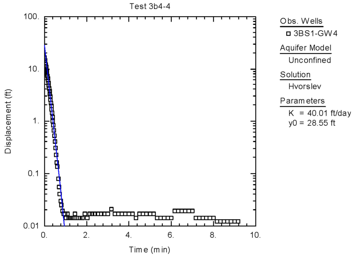
Figure C-22. Graphical Representation of Raw Data Obtained from Slug Test of 3BS1-GW4, Hvorslev Solution
