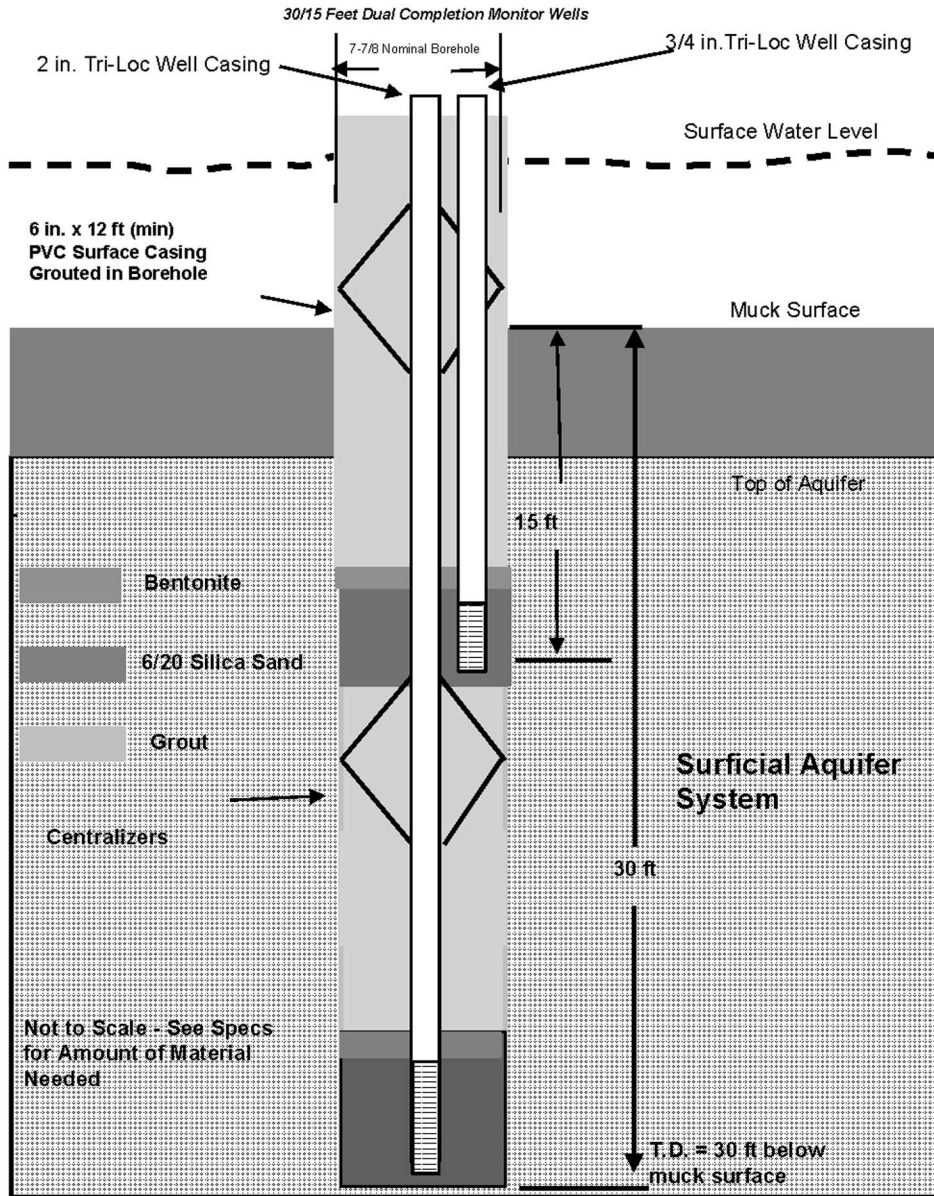
Figure 4. General Schematic of Dual Zone Monitor Well
