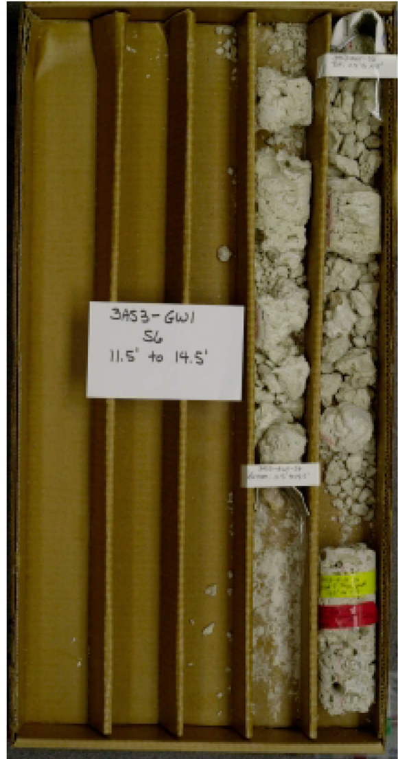
Figure B-2. Core from Well 3AS3-GW1, 11.5 to 14.5 ft below Peat
