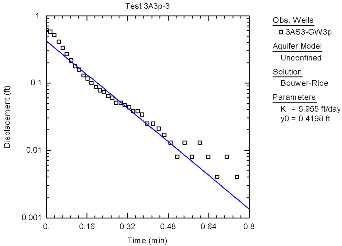
Figure C-11. Graphical Representation of Raw Data Obtained from Slug Test of 3AS3-GW3p, Bouwer-Rice Solution
