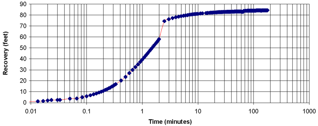
L-2 Canal Packer Test No. 2 -- Recovery Data Test Interval: 1,890 to 1,910 feet below land surface
