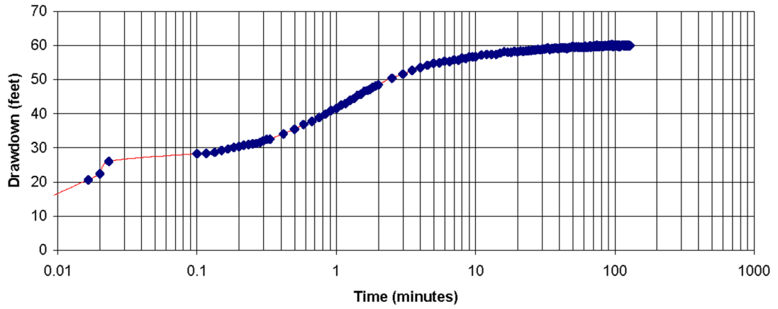
L-2 Canal Packer Test No. 4-- Drawdown Data Test Interval: 1,652 to 1,704 feet below land surface
