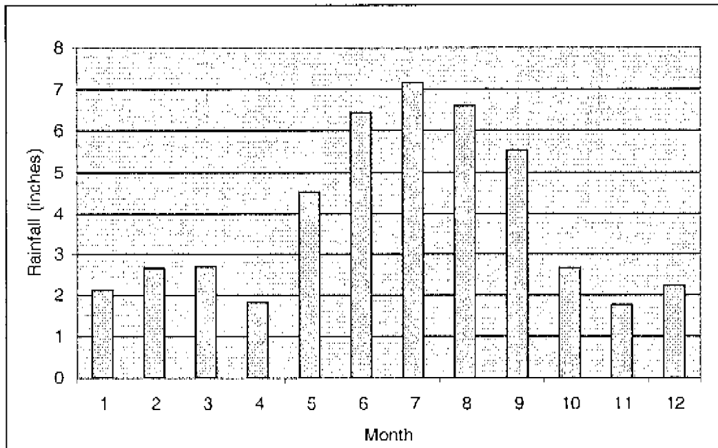
Figure 15a. Monthly mean of areal rainfall over the RCB.
