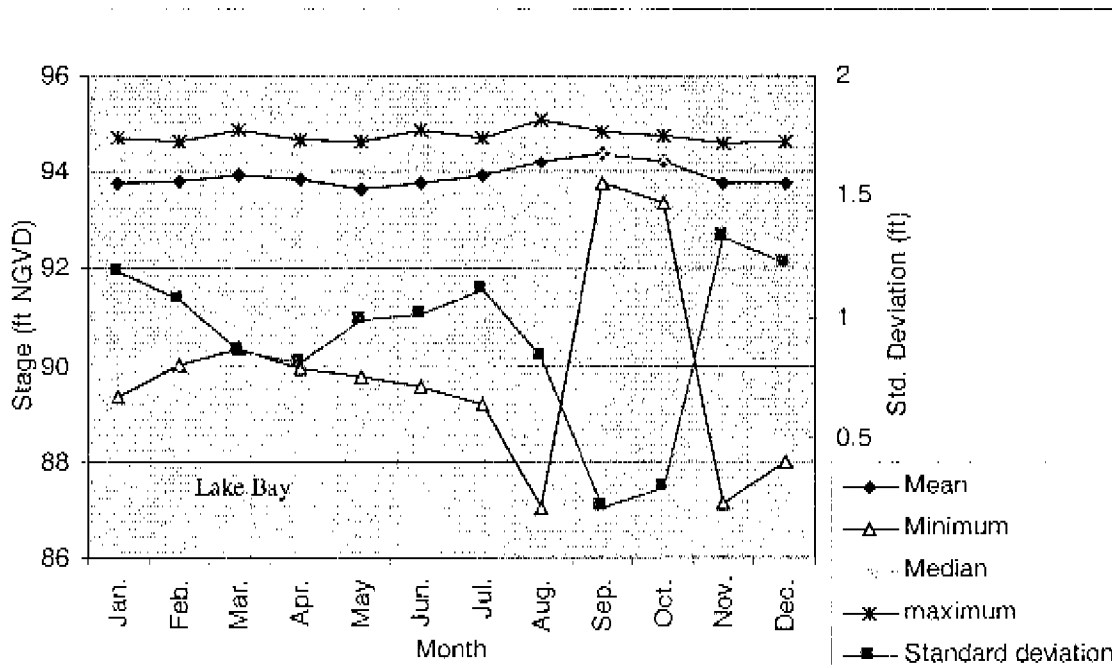
Figure C1-2. Monthly statistics for stage data at Lake Bay.
