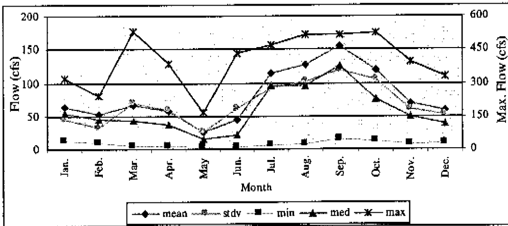
Figure 10b. Pre-67 flow monthly statistics at Reedy Creek, Loughman station.
