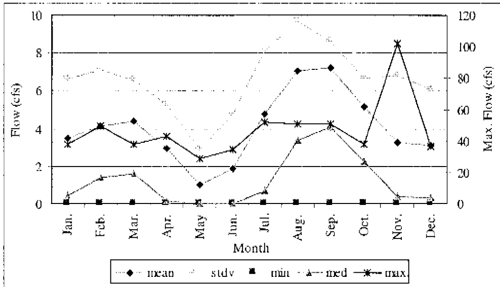
Figure 7b. Flow monthly statistics at Whittenthorpe, Vinland station.
