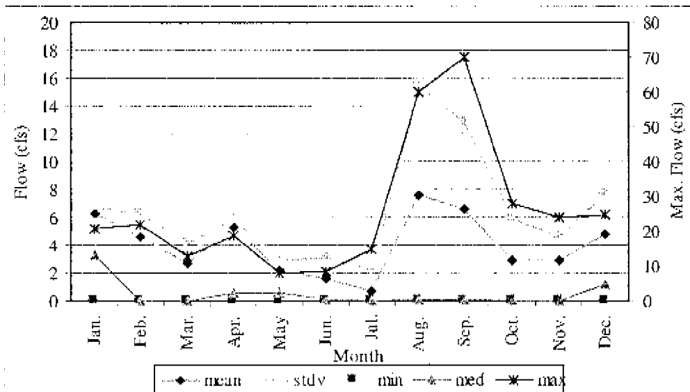
Figure 3b. Flow monthly statistics at Bay Lake outlet station.
