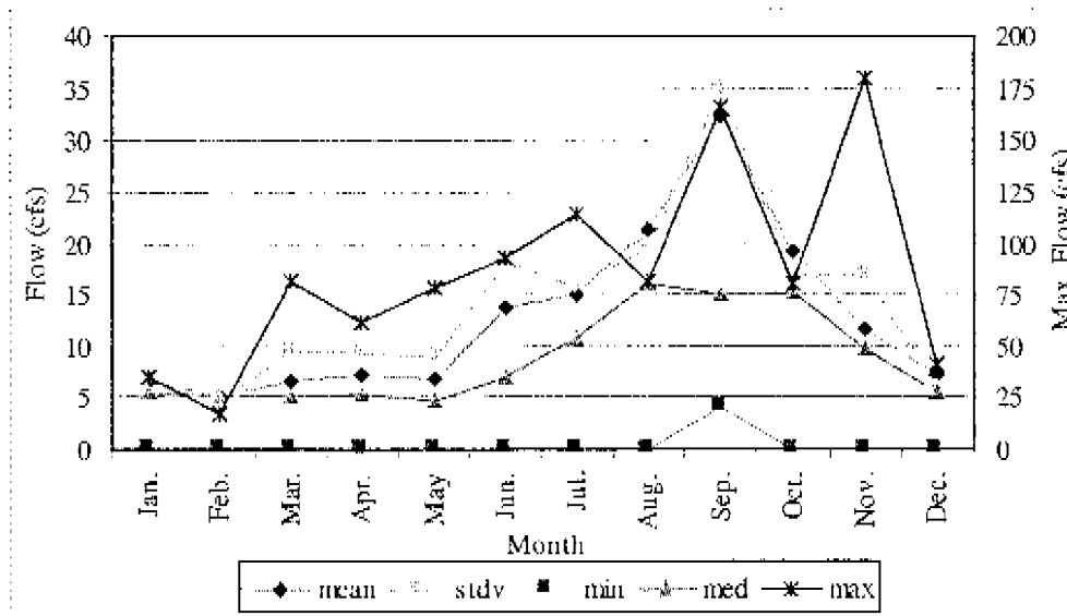
Figure 11b. Flow monthly statistics at Lateral 101 at S101 station.
