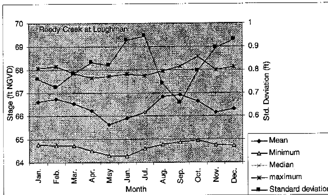
Figure C8-2. Monthly statistics for stage data at Reedy Creek at Loughman.
