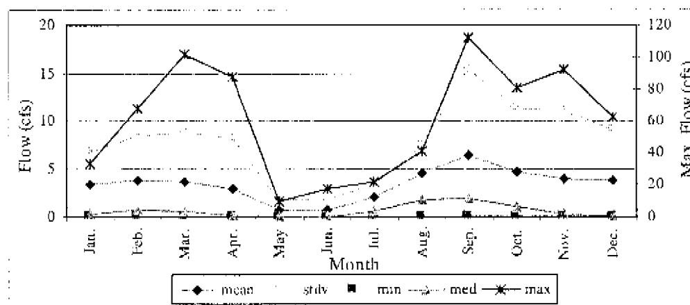
Figure 5c. Post-67 flow monthly statistics at Cypress Creek, Vineland station.
