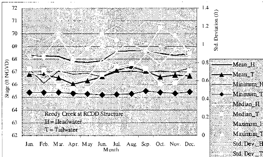
Figure C11-2. Monthly statistics for stage data (Headwater and Tailwater) at Reedy Creek, RCDD structure.
