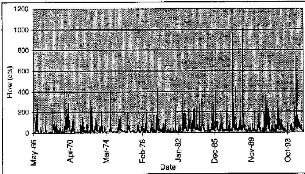
Figure 8a. Preferred flow data at Reedy Creek, Vineland station.
