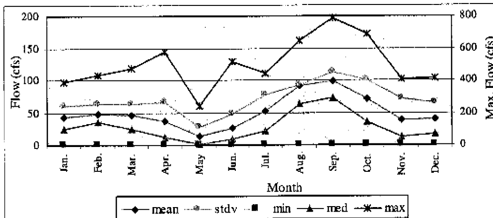
Figure 10c. Post-67 flow monthly statistics at Reedy Creek, Loughman station.
