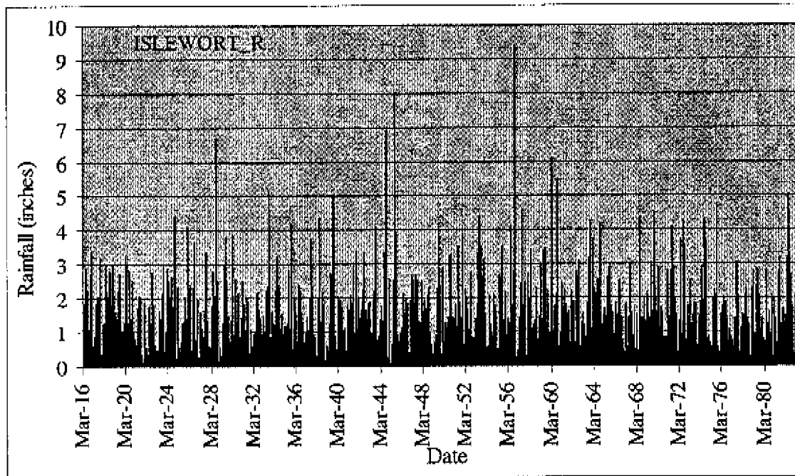
Figure A6. Historical daily rainfall data at station ISLEWORT_R (few records are cumulative values of more than one day).
