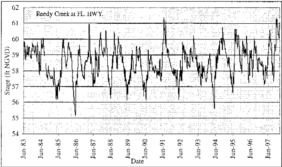
Figure C9-1. Historical daily stage at Reedy Creek at FL. HWY.
