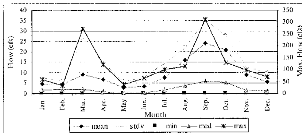
Figure 5b. Pre-67 flow monthly statistics at Cypress Creek, Vineland station.
