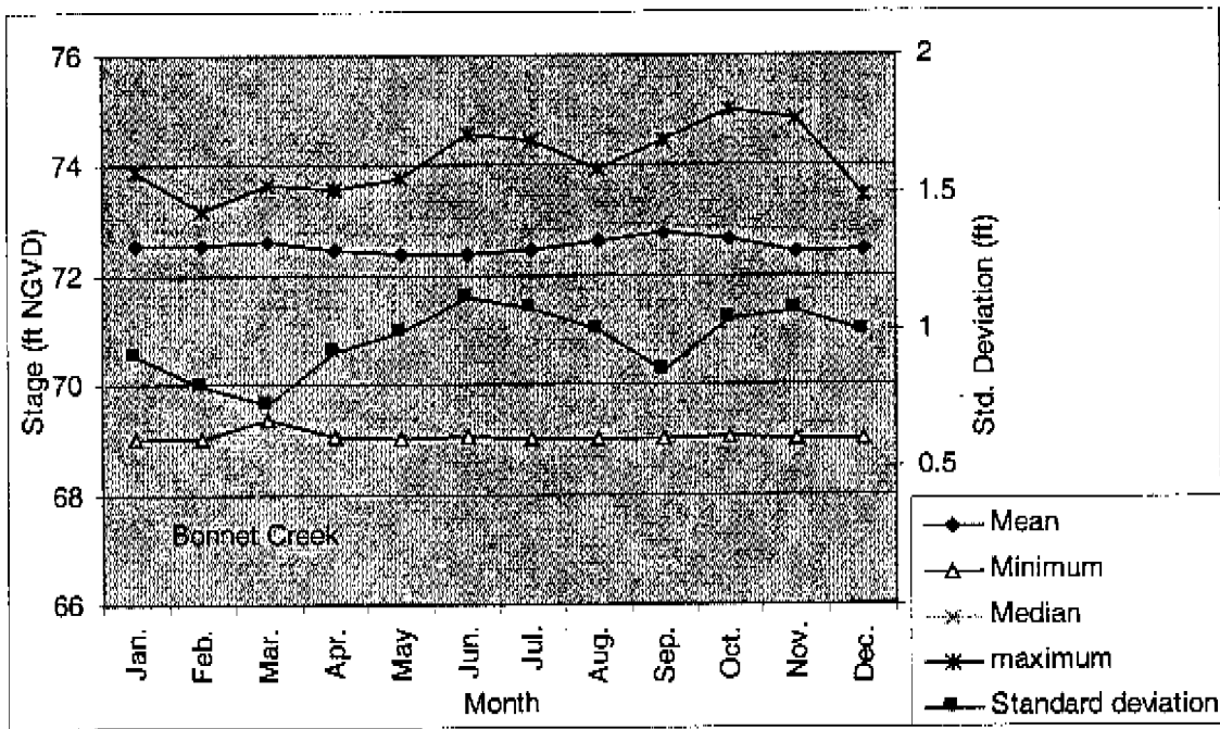
Figure C4-2. Monthly statistics for stage data at Bonnet Creek.
