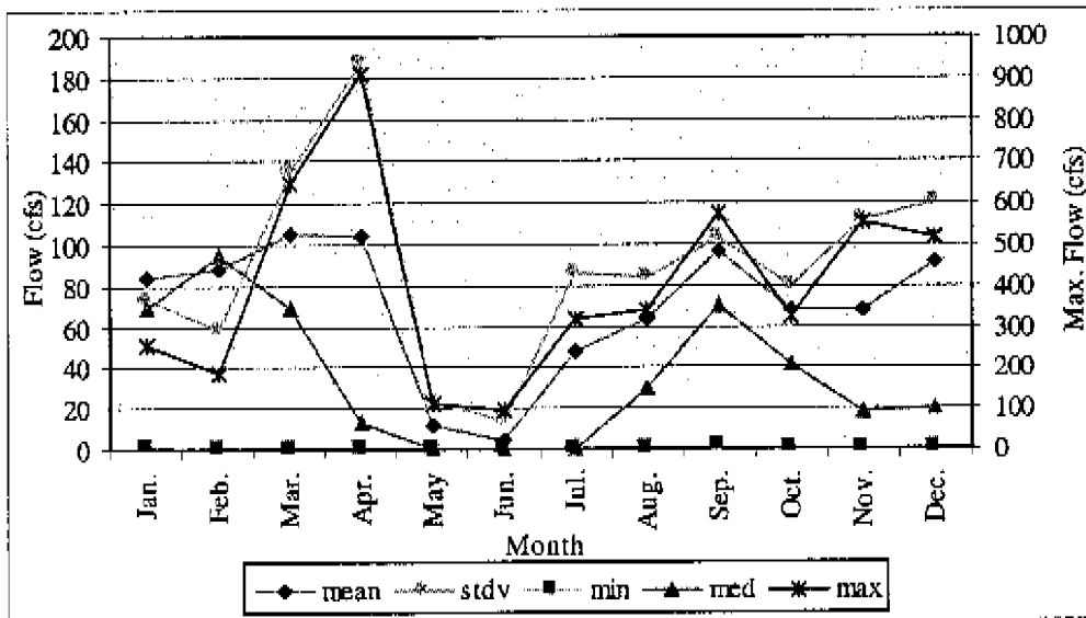
Figure 12b. Flow monthly statistics at Reedy Creek, Florida Highway station.
