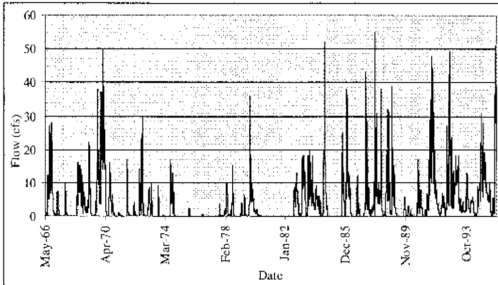
Figure 7a. Preferred flow data at Whittenthorpe Creek, Vinland station.
