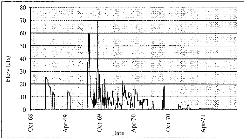
Figure 3a. Preferred flow data at Bay Lake outlet station.
