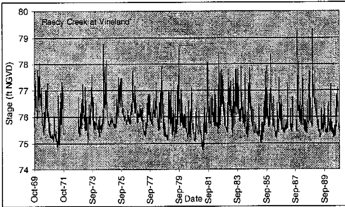
Figure C6-1. Historical daily stage at Reedy Creek at Vineland.
