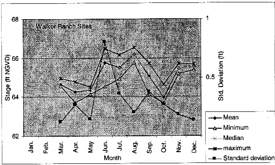
Figure C12-2. Monthly statistics for stage data at Walker Ranch sites.
