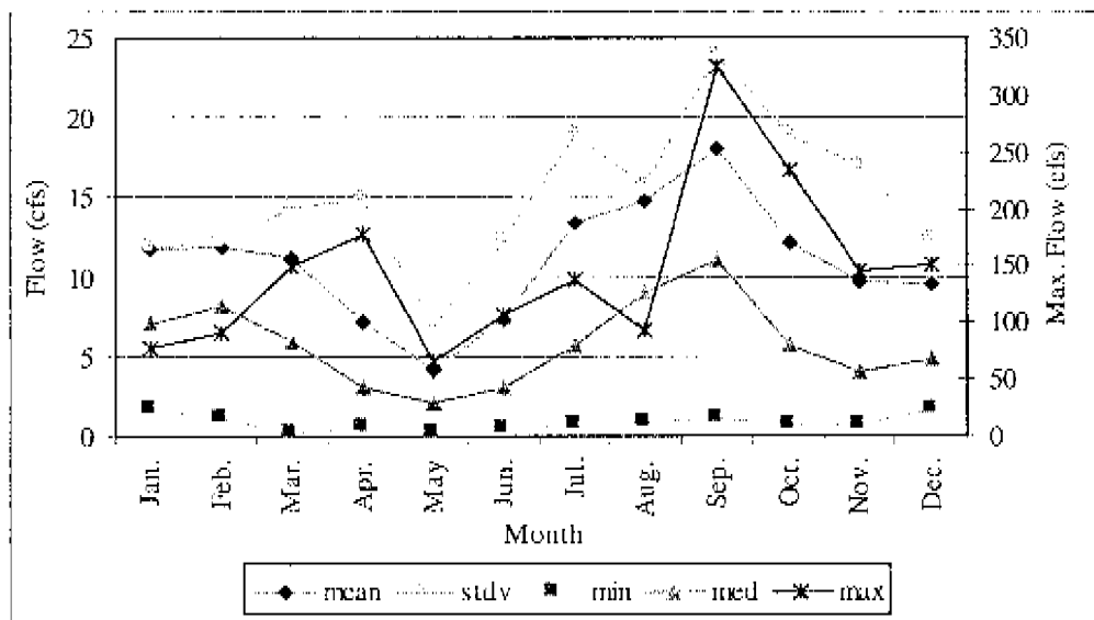
Figure 9b. Flow monthly statistics at Davenport, Loughman station.
