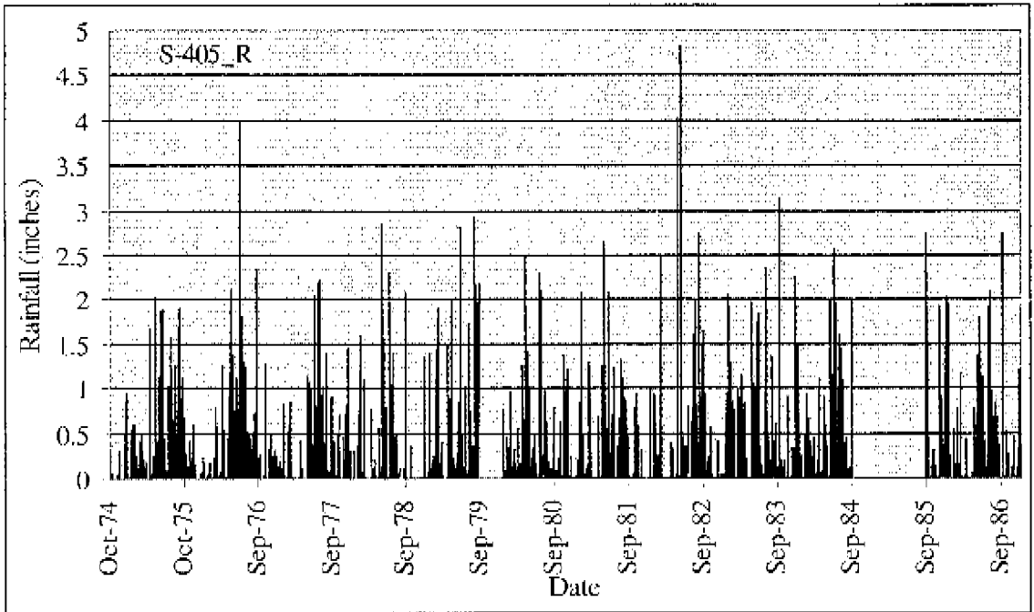
Figure A3. Historical daily rainfall data at station S-405_R (few records are cumulative values of more than one day)
