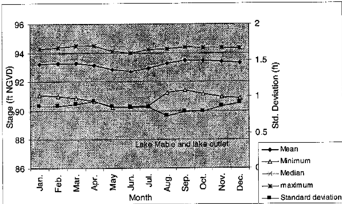
Figure C2-2. Monthly statistics for stage data at Lake Mable.
