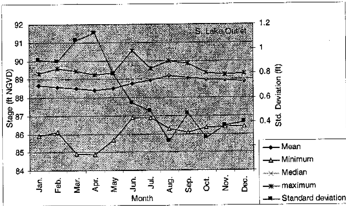
Figure C10-2. Monthly statistics for stage data at South Lake outlet.
