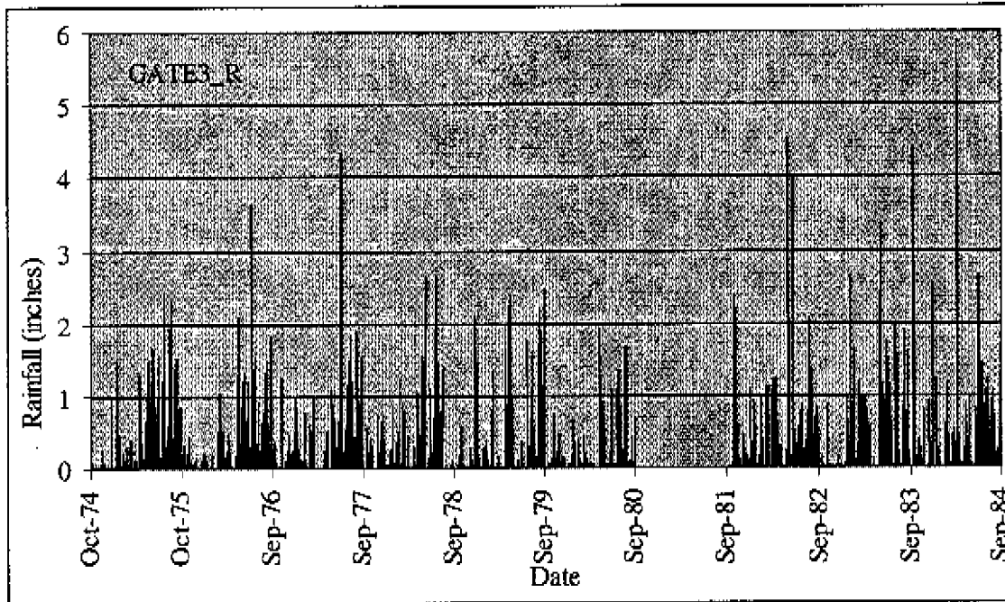
Figure A1. Historical daily rainfall data at station GATE3_R (few records are cumulative values of more than one day)
