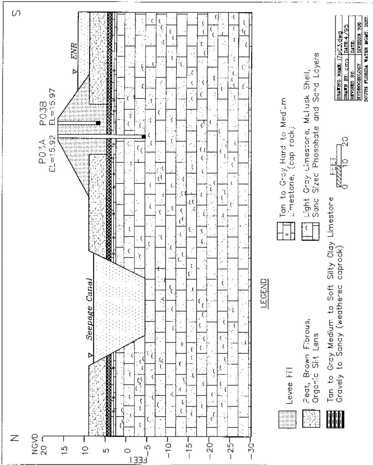
Figure A-3. Cross Section for Wells P-03A and P-03B Located on the Perimeter
