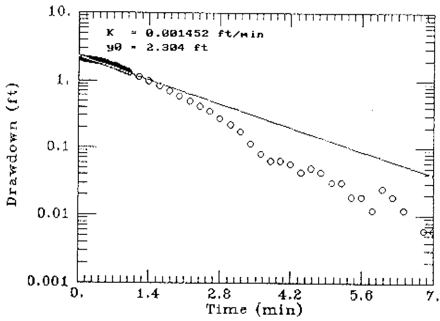
Figure D-11. Analyses of Slug Test for P05A
