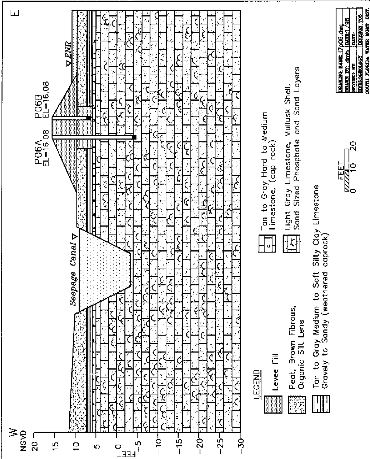
Figure A-6. Cross Section for Wells P-06A and P-06B Located on the Perimeter Levee
