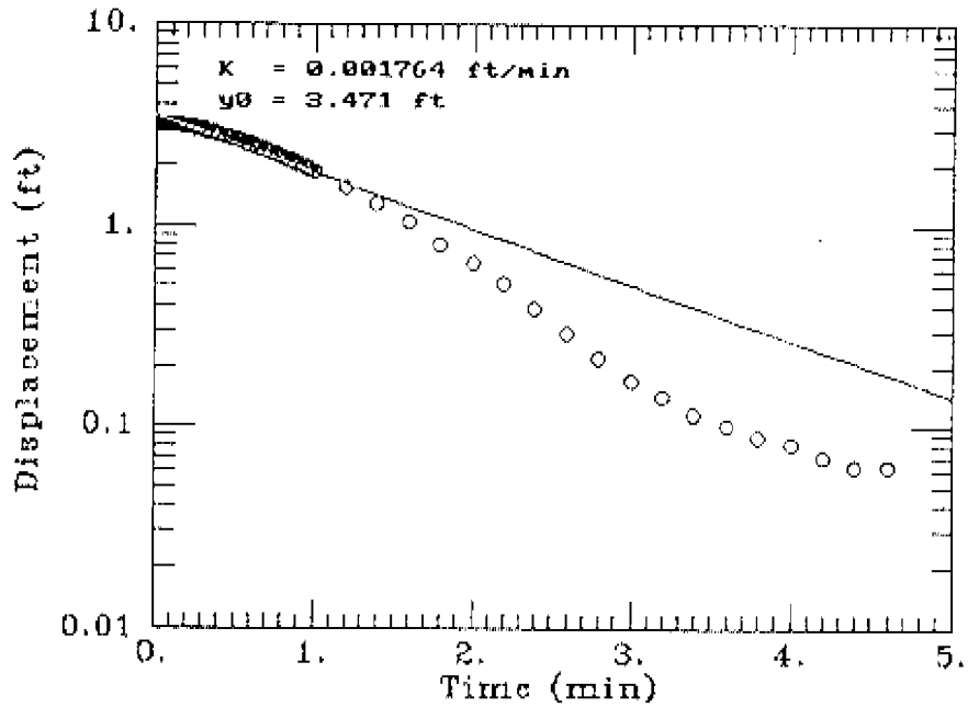
Figure D-17. Analyses of Slug Test for P10A
