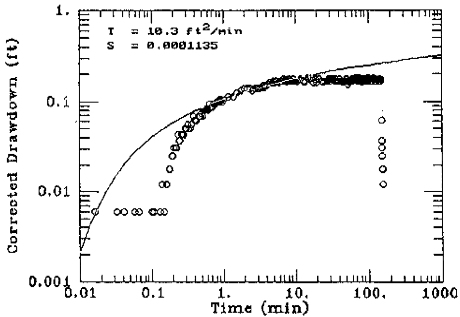
Figure D-4. Analyses of Aquifer Performance Test for P14B (Cooper-Jacob Method)
