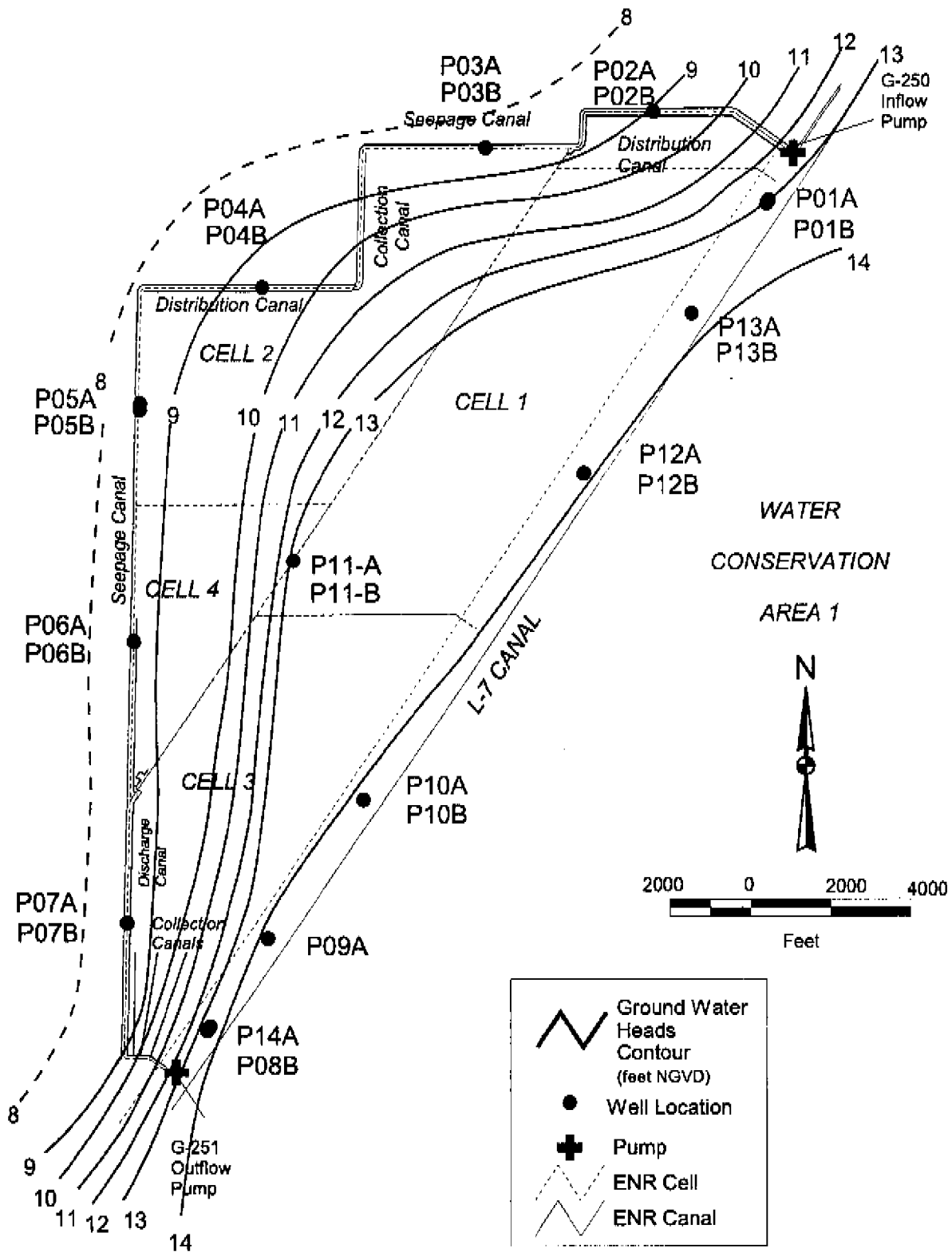
Figure 7. Altitude of the Water Table in the Surficial Aquifer, October 1995.
