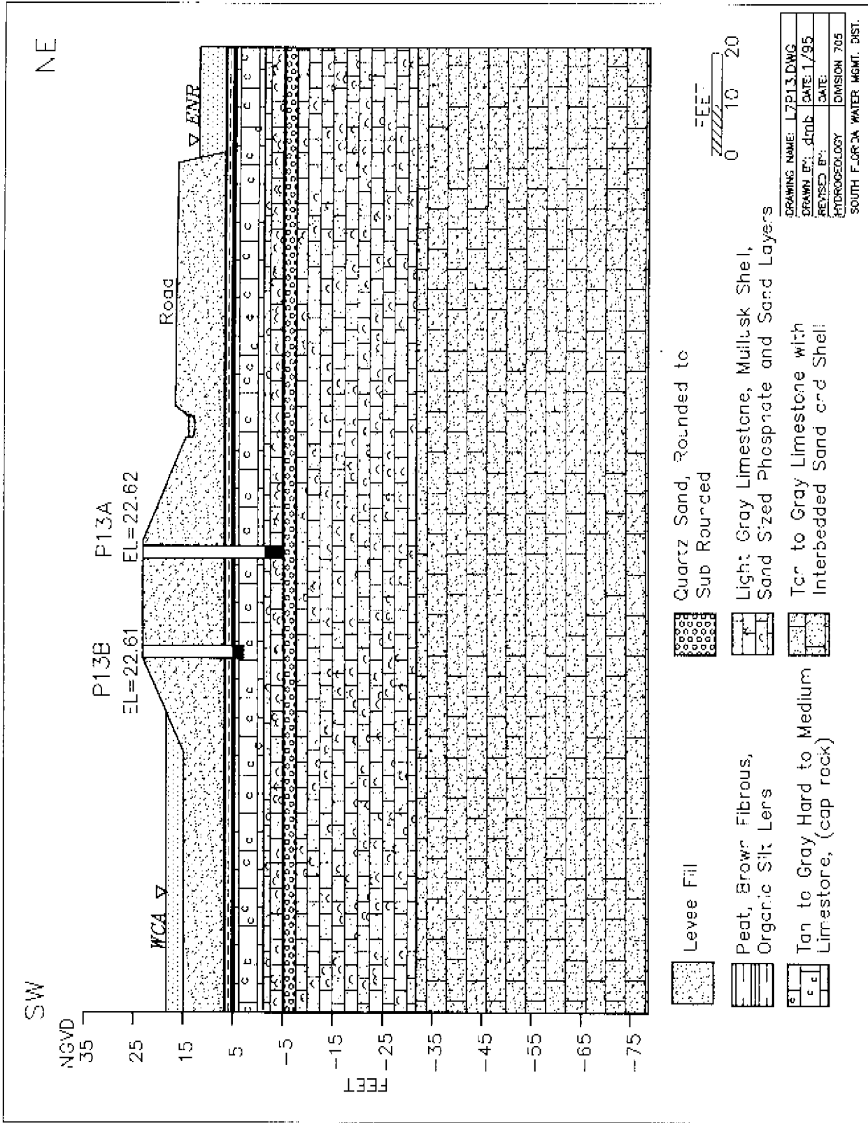
Figure A-11. Cross Section for Wells P-13A and P-13B Located on the L-7 Levee
