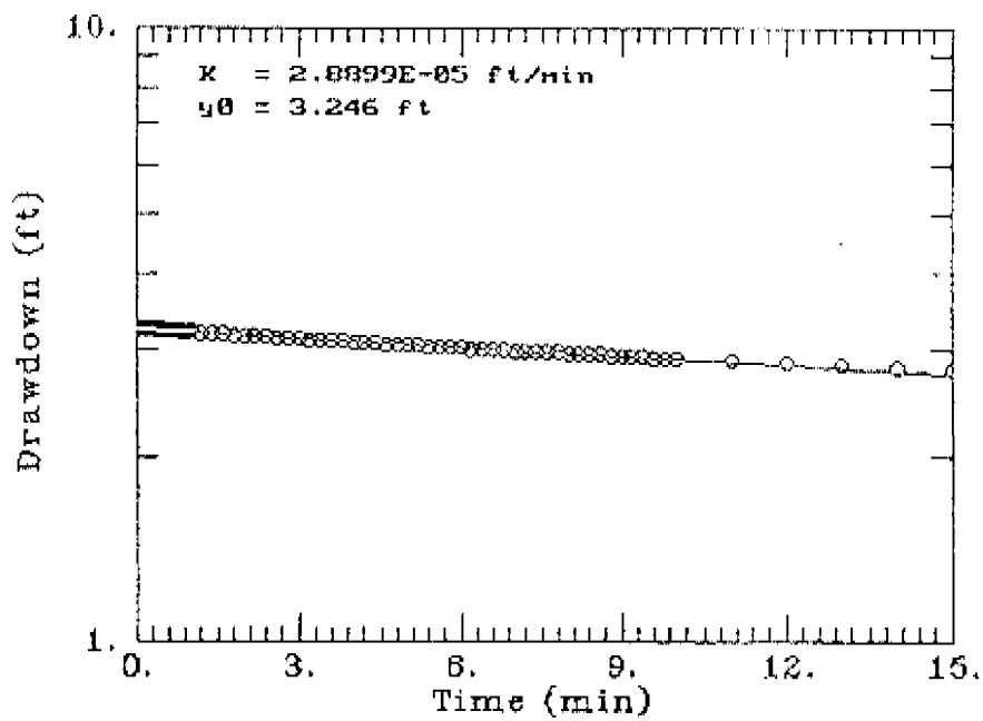
Figure D-5. Analyses of Slug Test for PO2A
