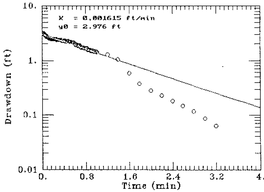
Figure D-13. Analyses of Slug Test for P06A
