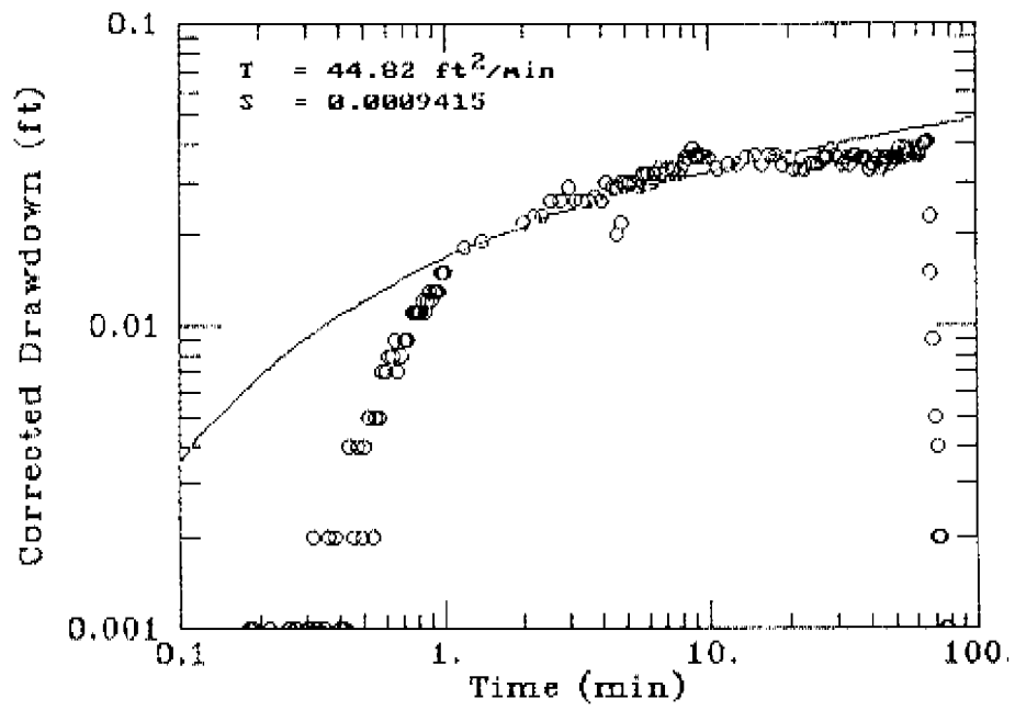
Figure D-1. Analyses of Aquifer Performance Test for PO1B (Theis Method)
