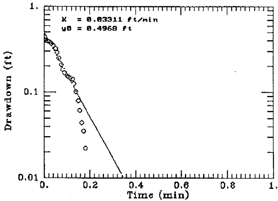
Figure D-16. Analyses of Slug Test for P07B
