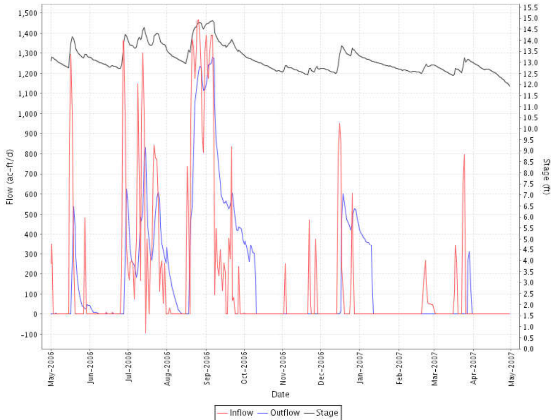
Figure 8. Inflow, outflow, and stage for STA-2, Cell 1.
