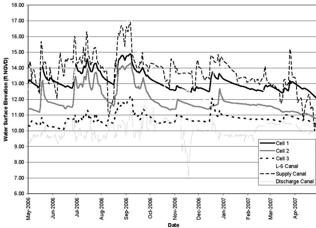
Figure 7. Stage in STA-2, Cells 1, 2, and 3 and surrounding areas.
