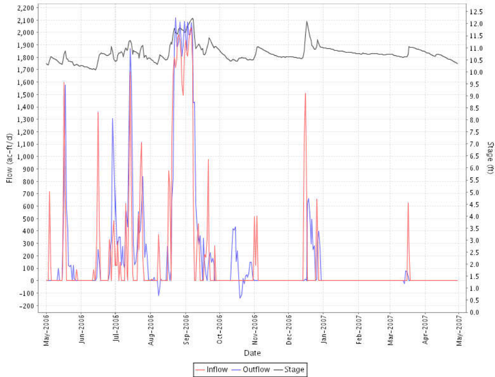
Figure 14. Inflow, outflow, and stage for STA-2, Cell 3.
