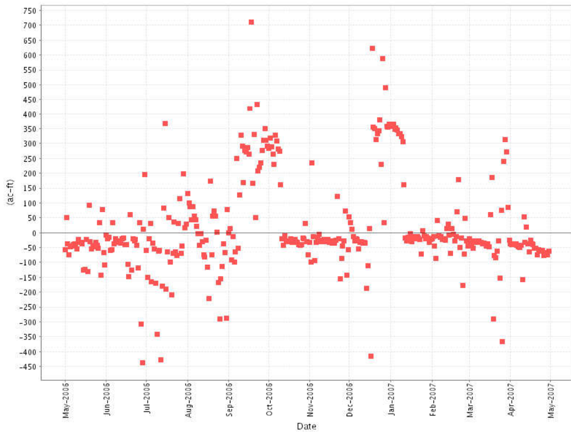
Figure 5. Daily water budget residuals for STA-2, Cell 1.
