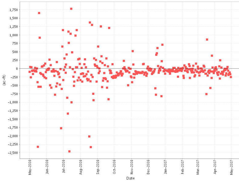
Figure 15. Daily water budget residuals for STA-2.
