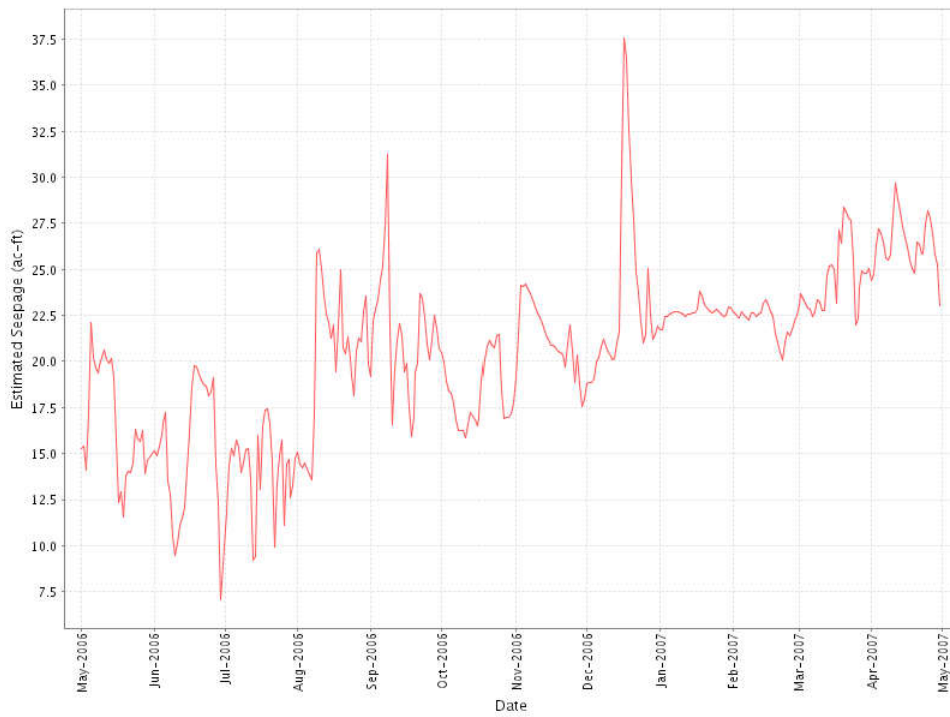
Figure 13. Estimated seepage for STA-2, Cell 3.
