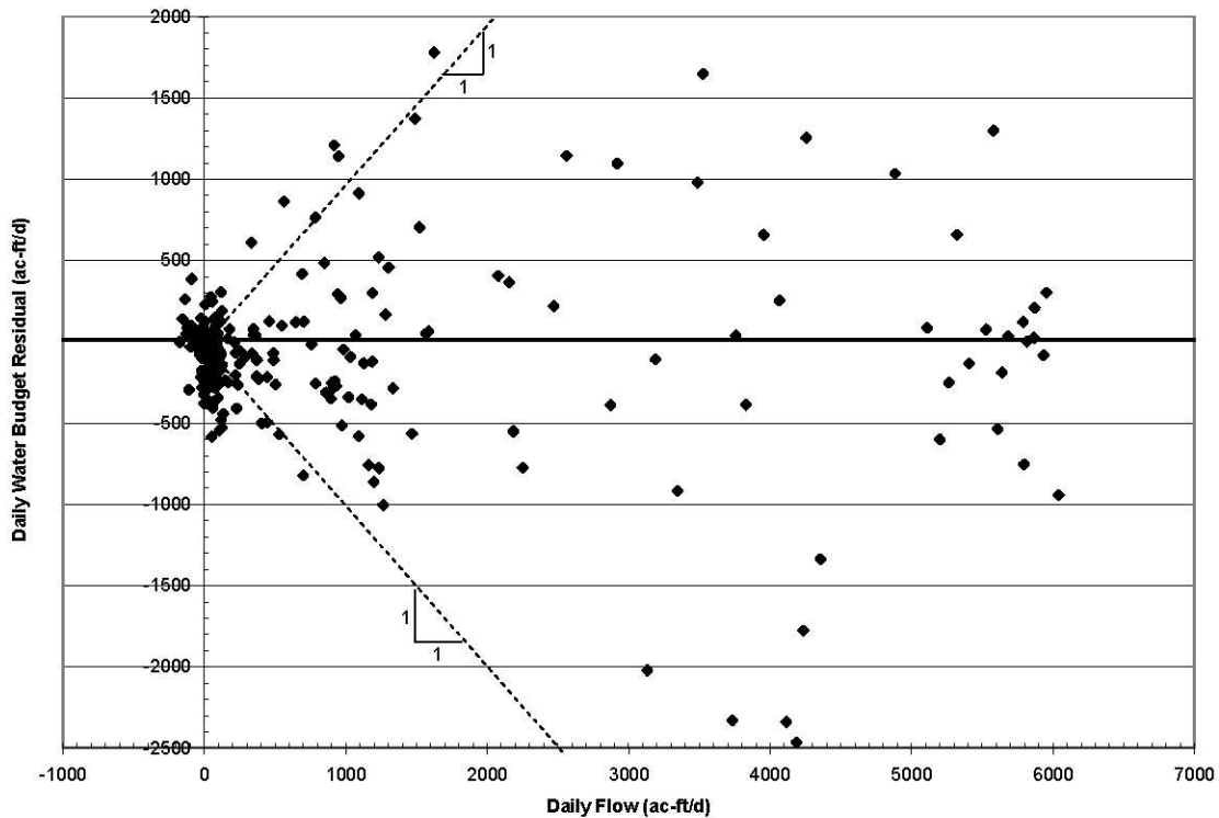
Figure 18. STA-2 water budget residual versus flow.
