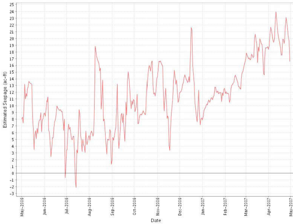
Figure 16. Estimated seepage for STA-2.
