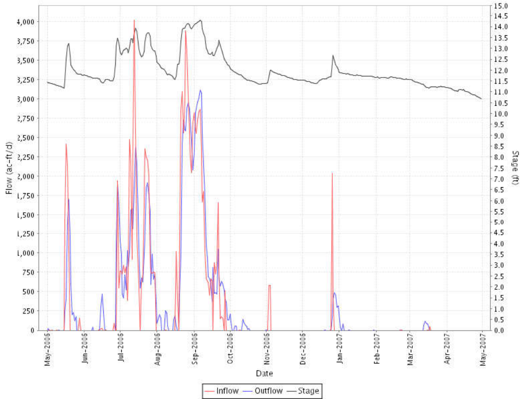
Figure 11. Inflow, outflow, and stage for STA-2, Cell 2.
