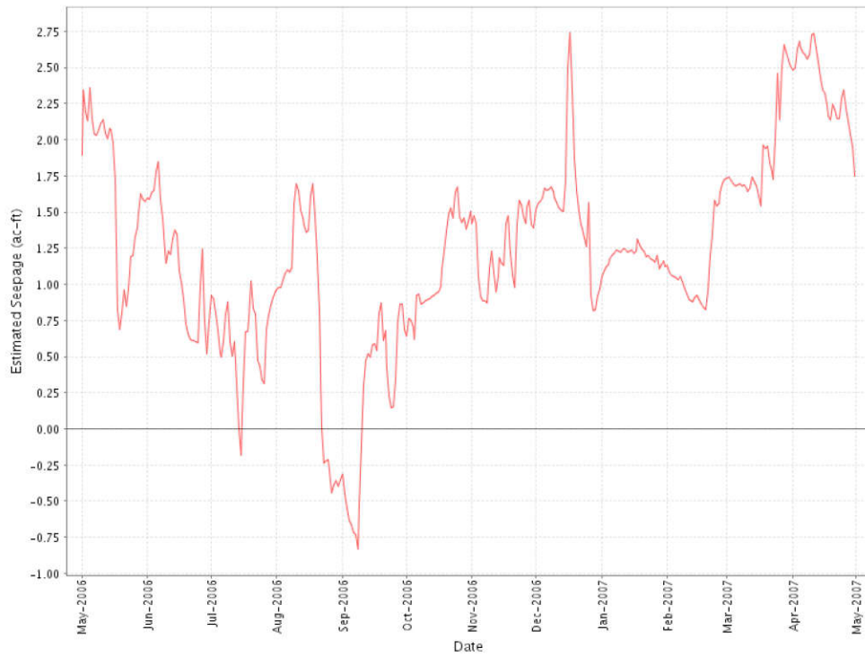
Figure 6. Estimated seepage for STA-2, Cell 1.
