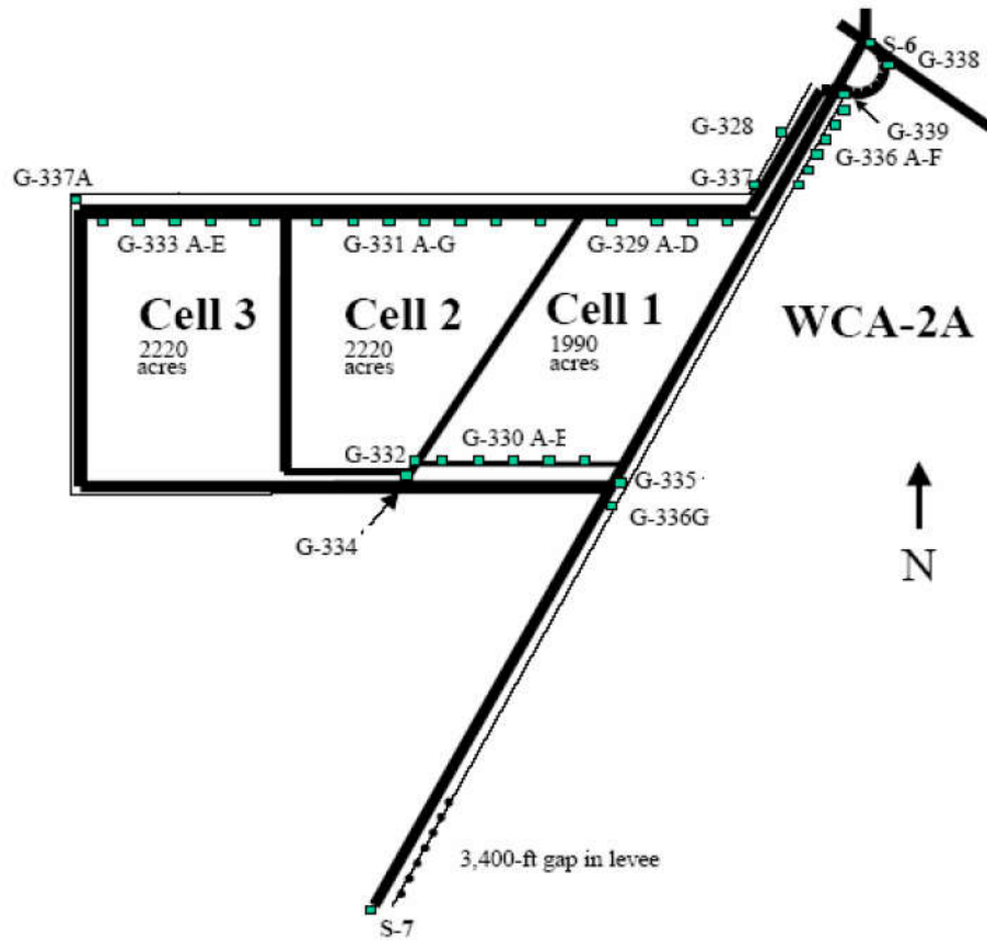
Figure 2. Schematic diagram of STA-2.
