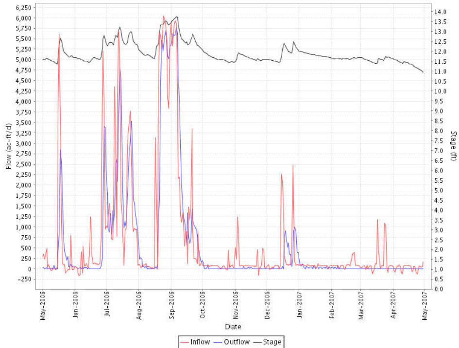
Figure 17. Inflow, outflow, and stage for STA-2.
