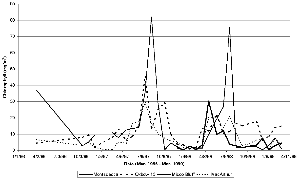
Figure 9-2. Chlorophyll a in remnant river runs of Pool C.
