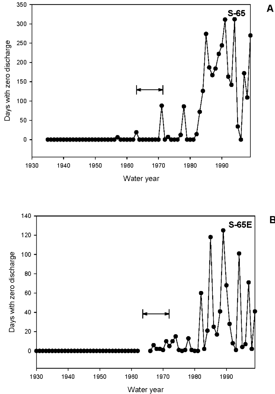
Figure 1-1. Number of days each water year that mean daily discharge was 0 cfs at S-65 (A) and S-65E (B). Double-headed arrows indicate the time interval when channelization occurred.
