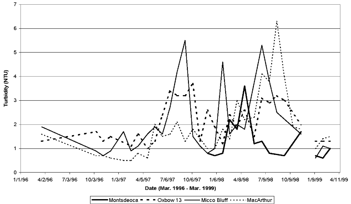
Figure 9-1. Turbidity in remnant river runs of Pool C.
