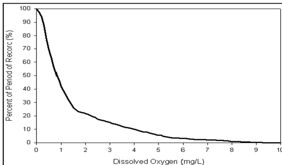
Figure 8-3. Percent of period of record (July 1997–June 1999) that Dissolved oxygen (DO) within remnant river channels exceeded x-axis values. Data are based on mean (average of 96 values per day) daily DO concentrations at two remnant river run stations in Pool C (Oxbow 13 and Montsdeoca Run). Dissolved Oxygen readings were taken at a depth of 1.0 m at each station.
