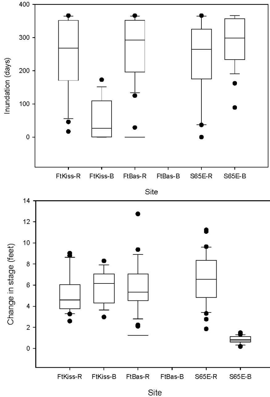
Figure 3-1. Box plots for inundation (number of days that stage exceeds the average ground elevation in a water year) and the change in stage per water year. Sites were Fort Kissimmee during the reference period (FtKiss-R) and baseline (FtKiss-B) periods, Fort Basinger during reference (FtBas-R) and baseline (FtBas-B) periods, and S-65E during reference (S65E-R) and baseline (S65E-B) periods. A box plot was not constructed for Fort Basinger during the baseline period because the single water year of data during the baseline period was insufficient.
