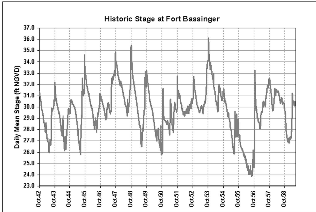
Figure 4-3. Historic daily surface water levels at Fort Bassinger.
