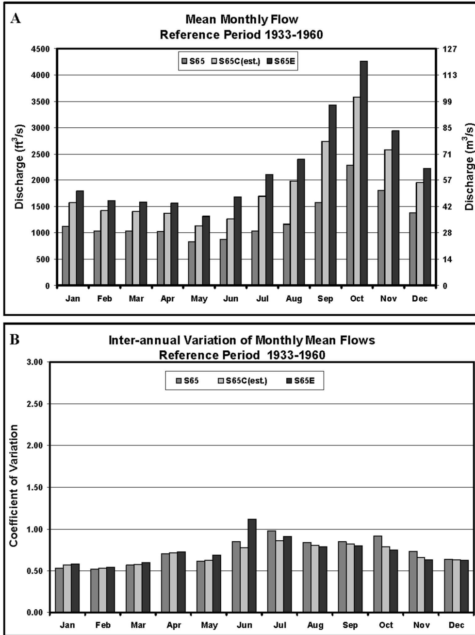
Figure 2-2. (A) Historic mean monthly flows along the Kissimmee River. S-65 represents flows at the outlet of Lake Kissimmee. S-65E represents flows near Lake Okeechobee. S-65C (est.) represents estimated flow conditions for the lower portion of the first phase of restoration. (B) Historic year-to-year variation of monthly mean flows along the Kissimmee River. S-65 represents flows at the outlet of Lake Kissimmee. S-65E represents flows near Lake Okeechobee. S-65C (est.) represents estimated flow conditions for the lower portion of the first phase of restoration.
