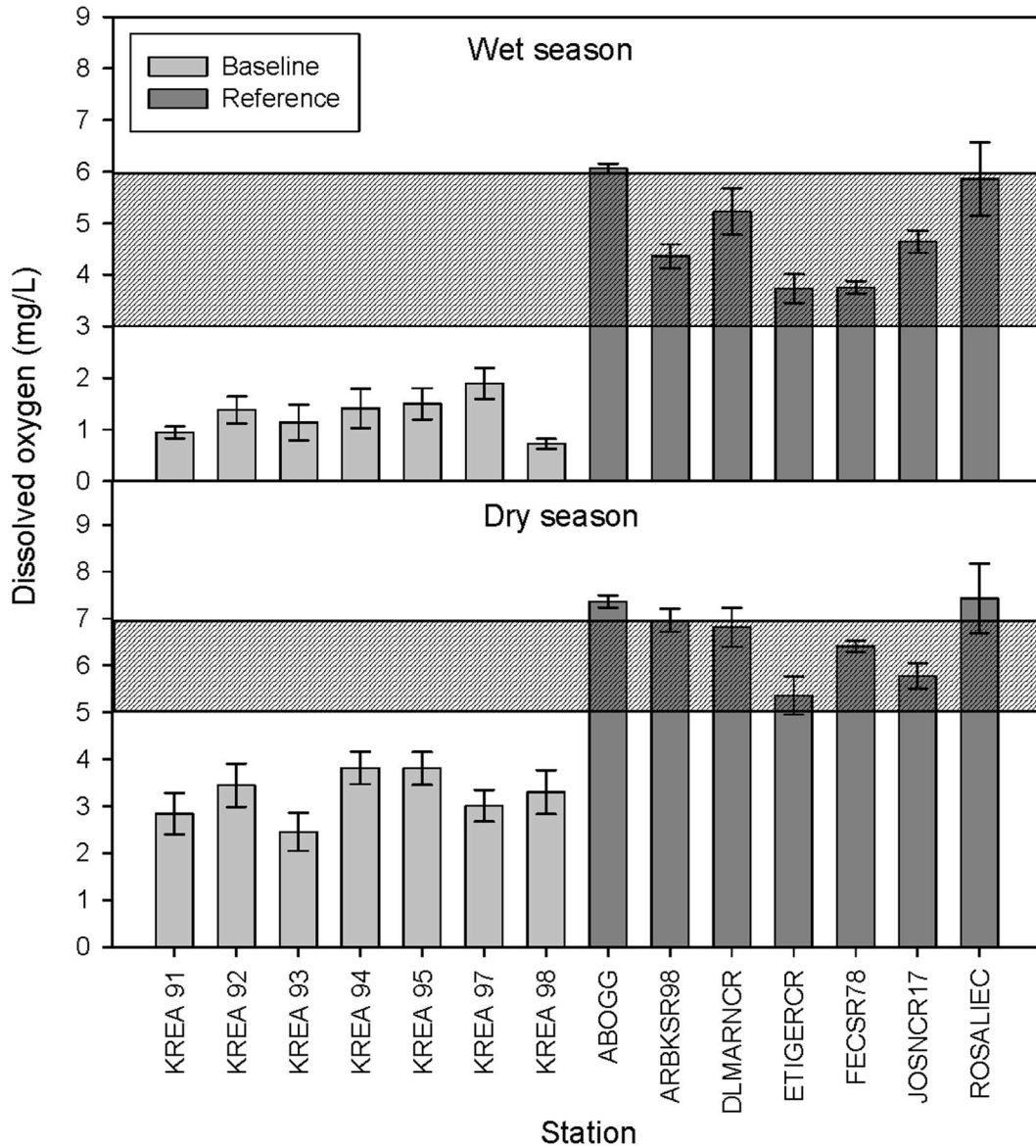
Figure 8-1. Mean ( \pm standard error of the mean) dissolved oxygen (DO) concentrations in free-flowing, blackwater, south Florida streams and remnant runs of the channelized Kissimmee River during the wet (June–November) and dry (December–May) season. Cross-hatched area represents expected range of DO concentrations in the Kissimmee River after restoration.
