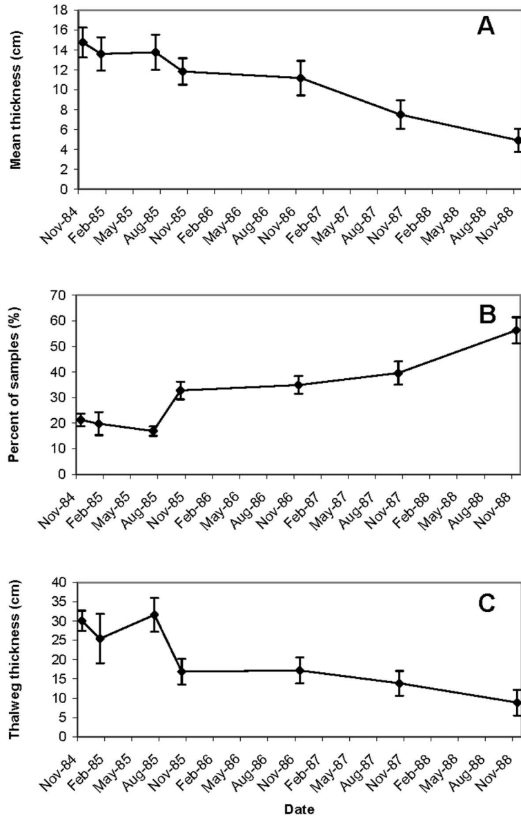
Figure 6-1. Mean values ( \pm standard error) for (A) mean thickness of substrate-overlying deposits, (B) percent of samples without substrate-overlying deposits, and (C) the thickness of substrate-overlying deposits at the thalweg during the Kissimmee River Demonstration Project. The first sample date is prior to the weirs being installed and combines data from November 1984 for R3, March 1985 for R2, and July 1985 for R1.
