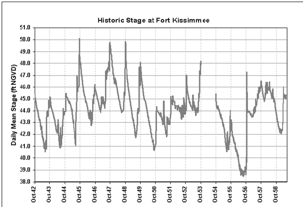
Figure 4-2. Historic daily surface water levels at Fort Kissimmee.
