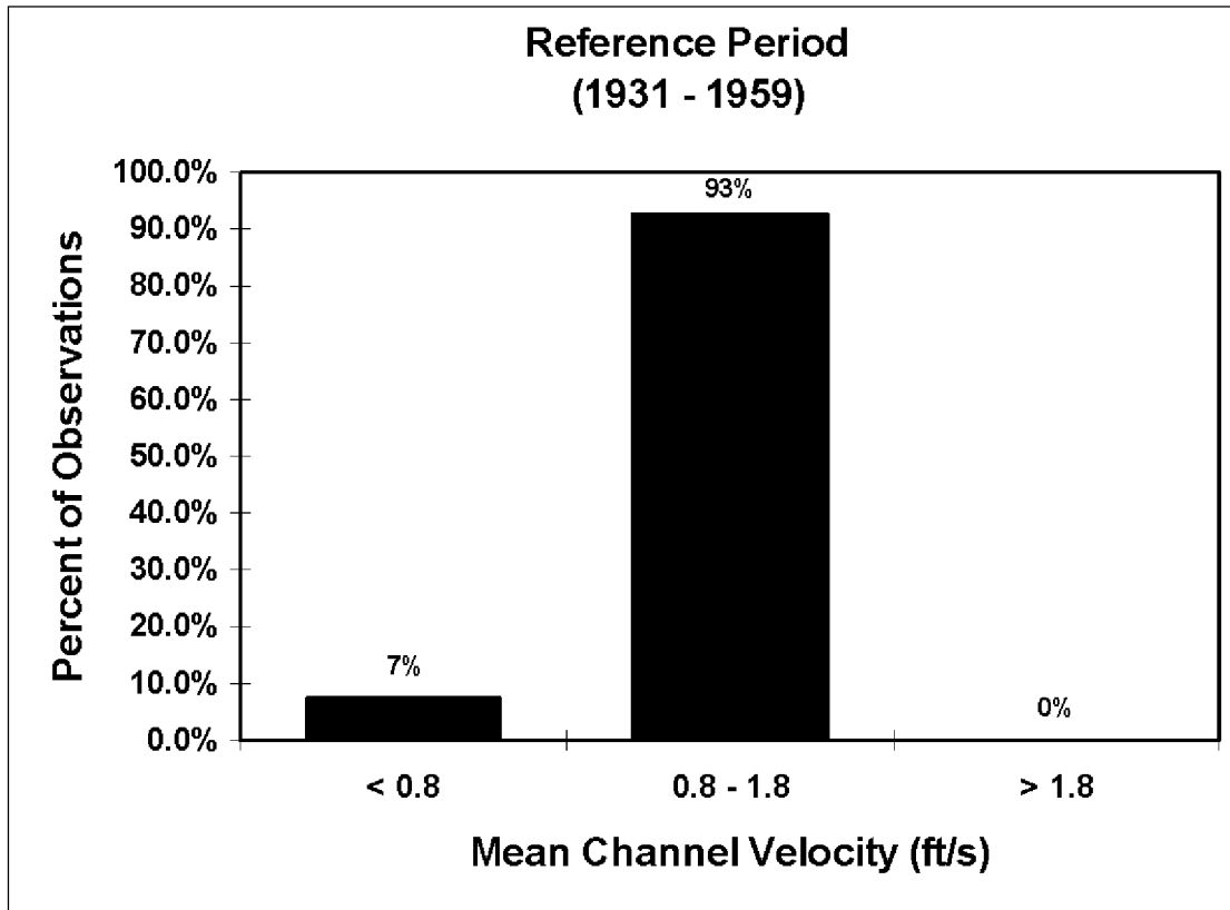
Figure 5-1. Frequency distribution of mean channel velocities near Fort Bassinger (n=24) and downstream of Lake Kissimmee (n=155). Data were collected during stream gauging events and are not from continuous monitoring.
