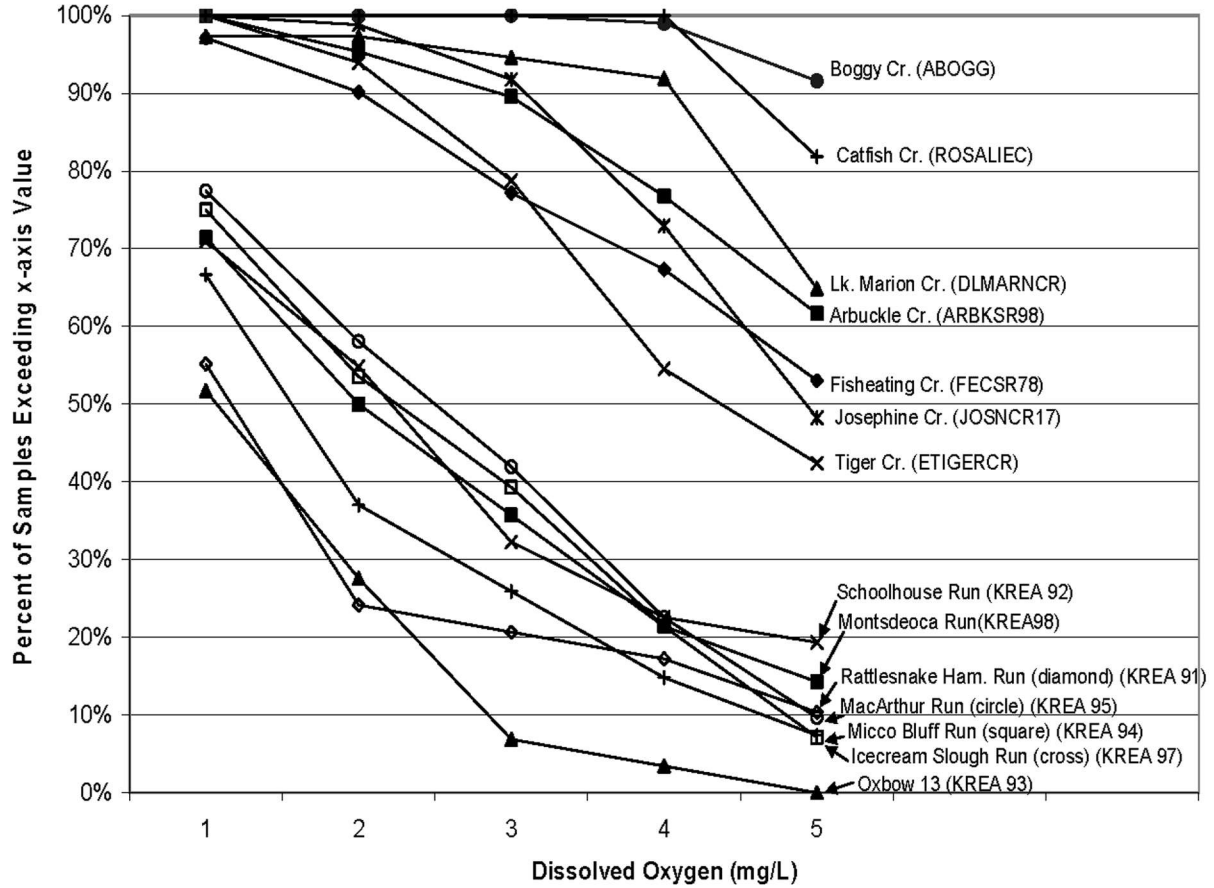
Figure 8-2. Dissolved Oxygen concentrations at 0.5 m depth in south Florida reference streams and remnant runs of the channelized Kissimmee River.
