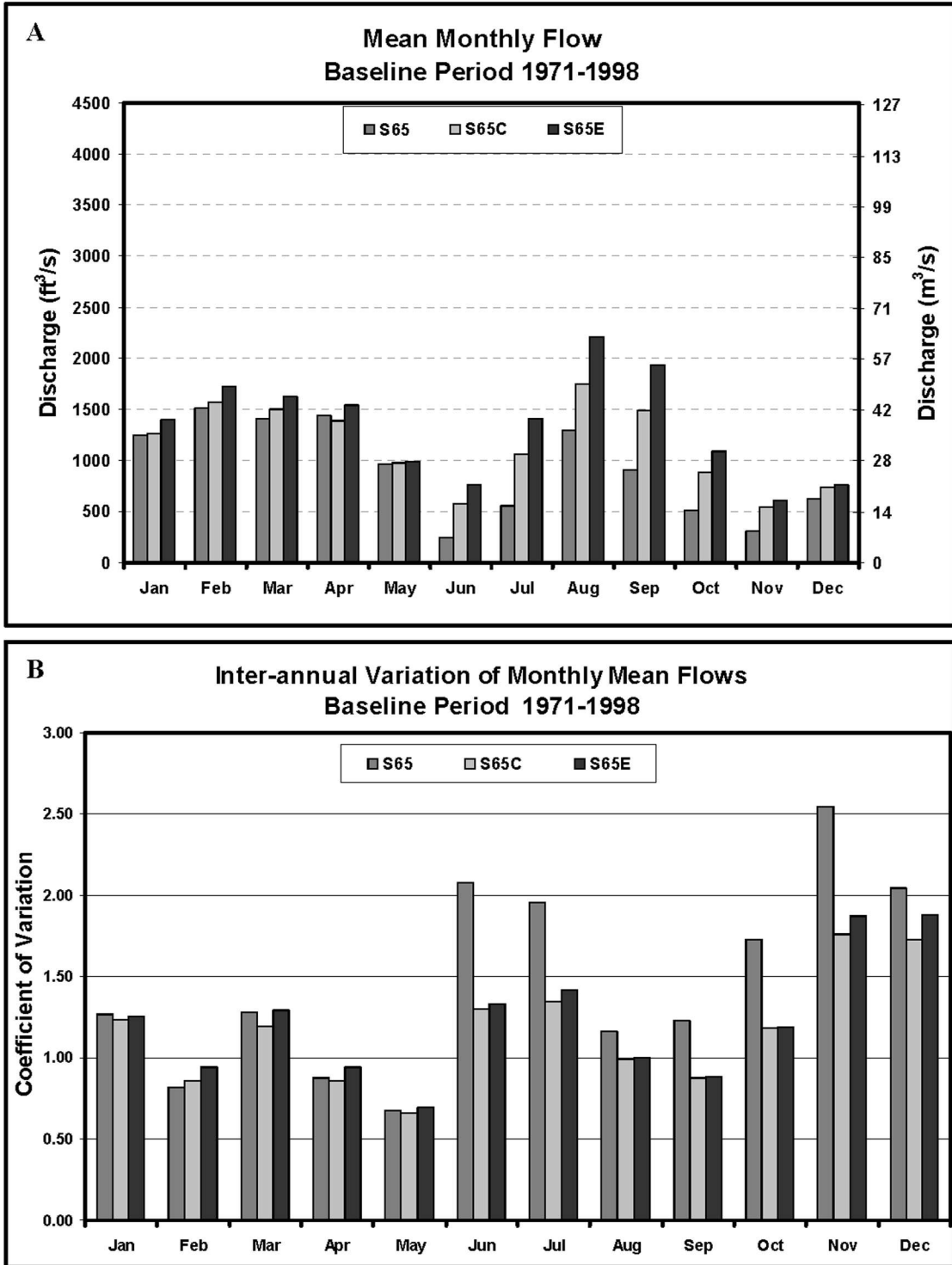
Figure 2-1. (A) Baseline mean monthly flows along the channelized Kissimmee River. (B) Baseline year-to-year variation of monthly mean flows along the channelized Kissimmee River.
