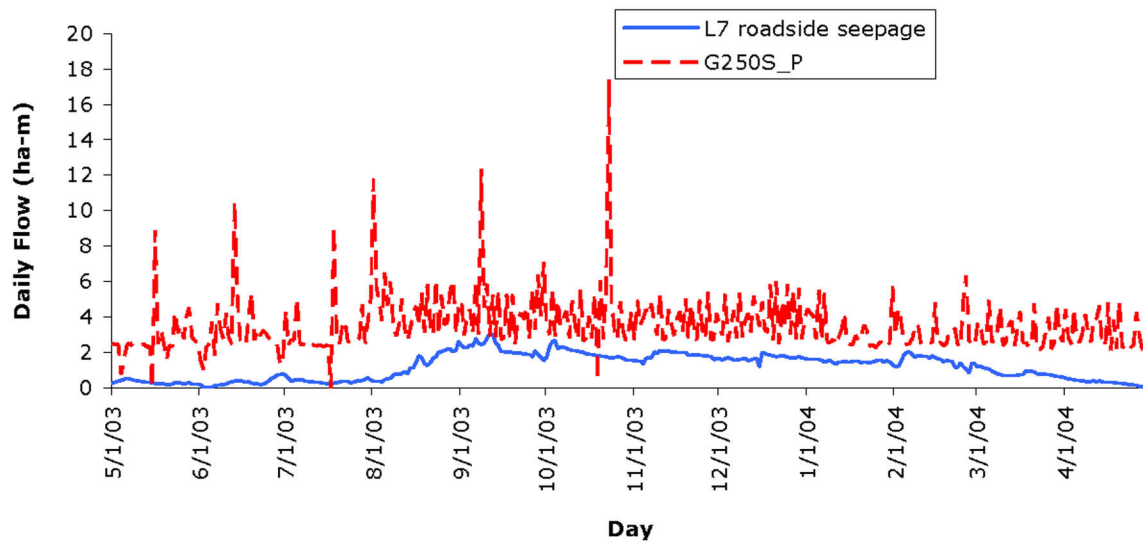
Figure 5. Daily pumping rates of the seepage/recirculation pump and seepage flow through L-7 levee roadside seepage collection culverts in STA-1W.
