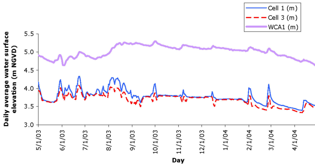
Figure 6. Daily mean water levels in Cells 1 and 3 of STA-1W and Water Conservation Area 1.
