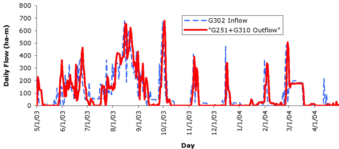
Figure 4. Daily STA-1W inflows and outflows.
