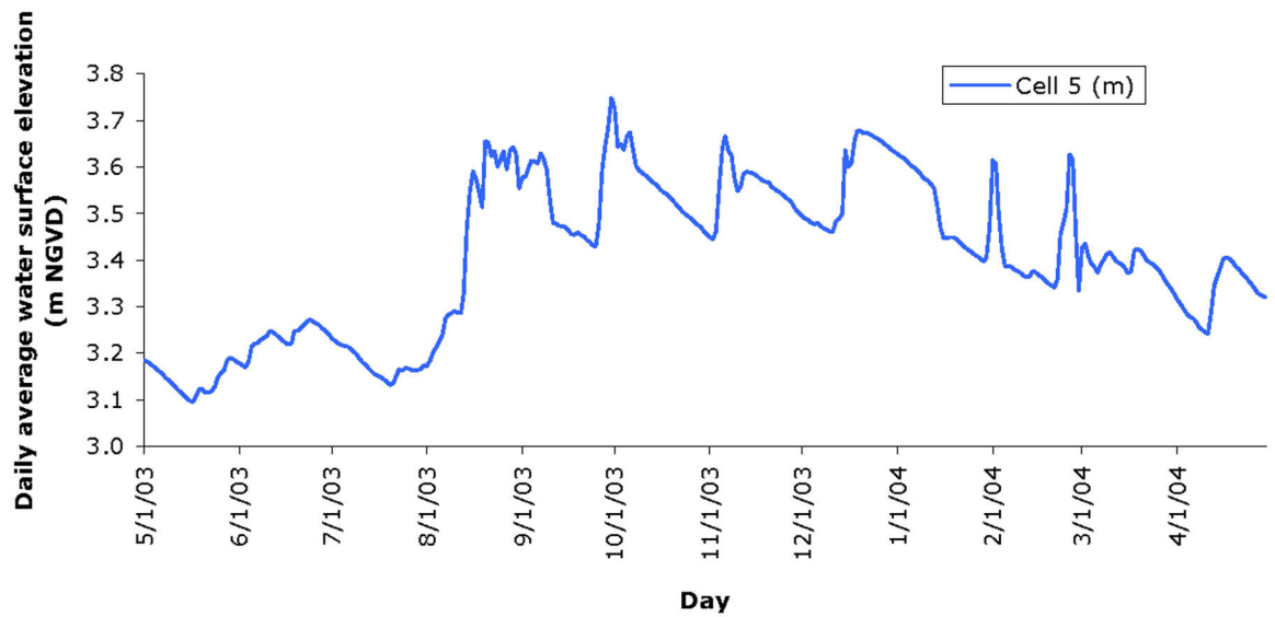
Figure 8. Daily mean water level in Cell 5 of STA-1W.
