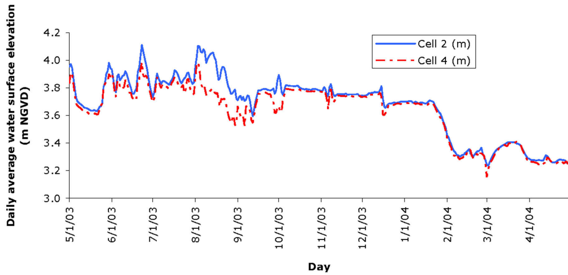
Figure 7. Daily mean water level in Cells 2 and 4 of STA-1W.
