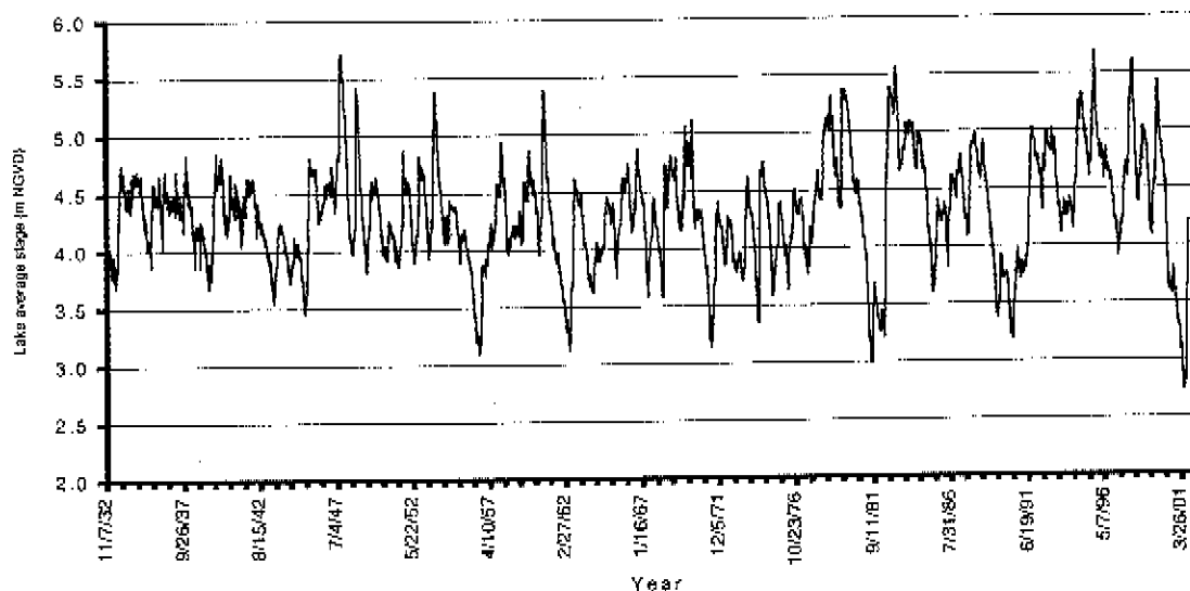
Figure 9. Average daily water level for Lake Okeechobee.
