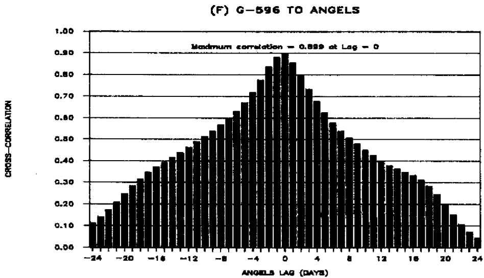
Figure 37. Cross-correlations Between G-596, G-1502, G-3273, and Angel's Well for the Period June, 1985 through May, 1986
