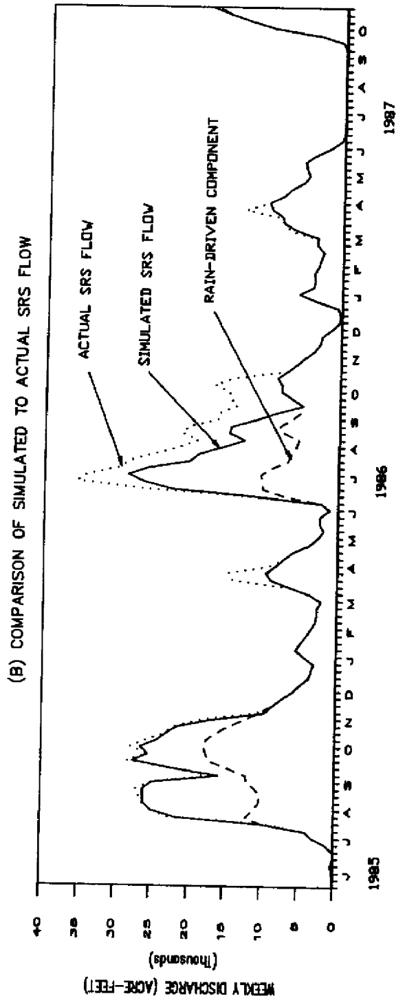
Figure 19. WCA 3A Water Levels and SRS Flow: Simulated Assuming the IAP Had Not Been in Effect
