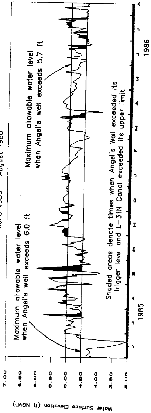
Figure 11. Comparison of Angel's Well and L-31N Water Levels North of S-331
