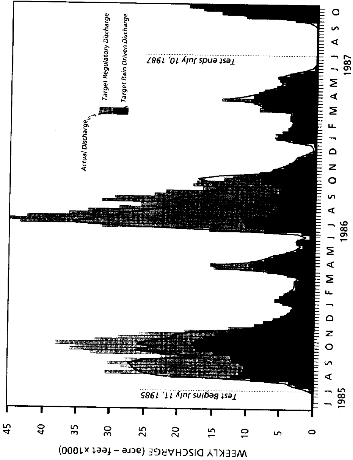
Figure 7. Comparison of Target and Actual Discharge to Shark River Slough
