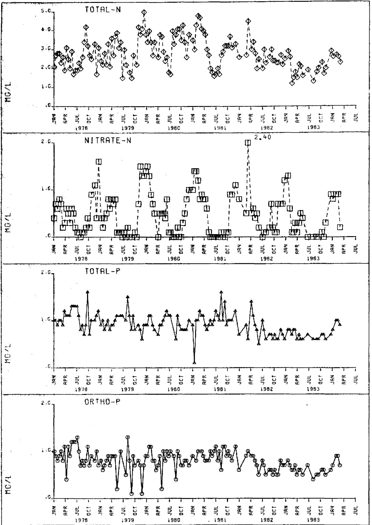
FIGURE S191 AT LAKE OKEECHOBEE
