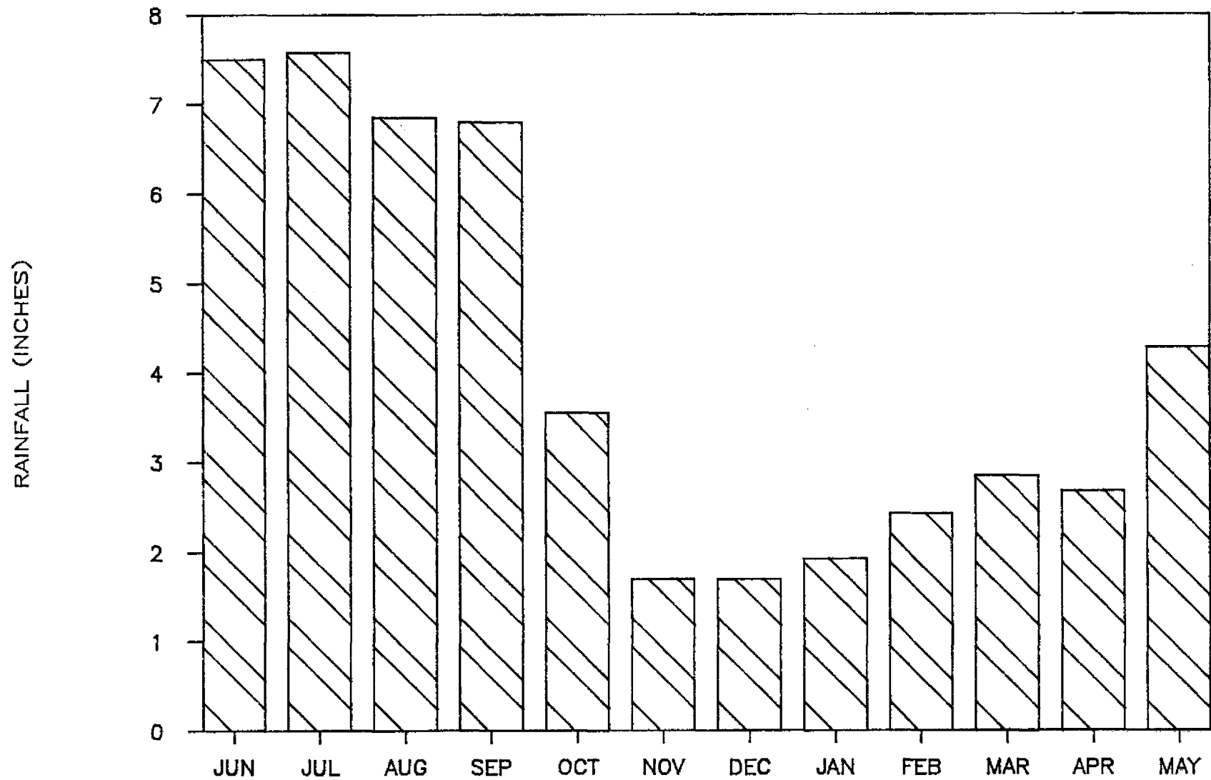
FIGURE 13 UPPER KISS.—KISS.—FEC BASIN
