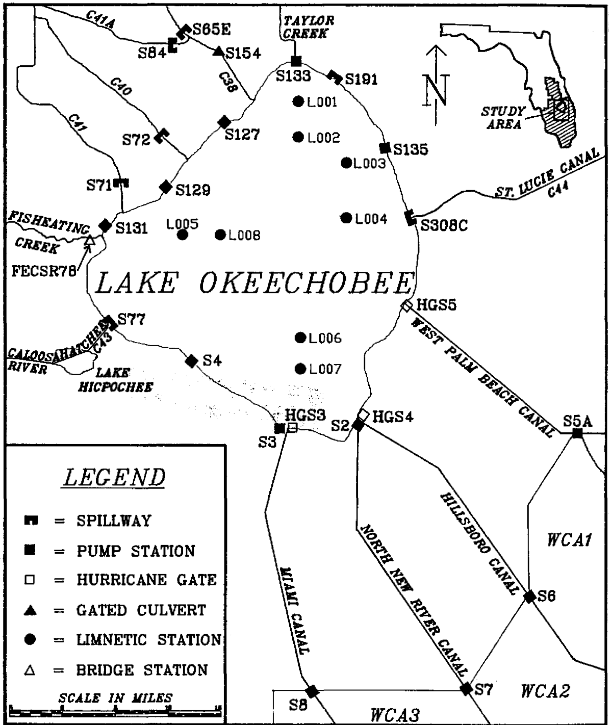
Figure 34. Lake Okeechobee Water Quality Management Plan Sampling Stations.
