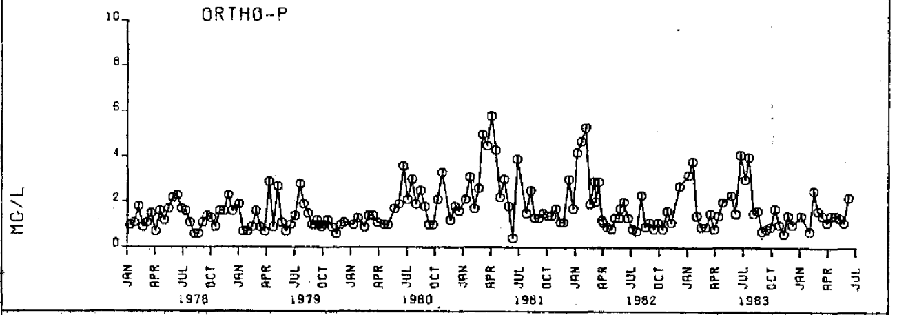
FIGURE NUBBIN SLOUGH STATION 14
