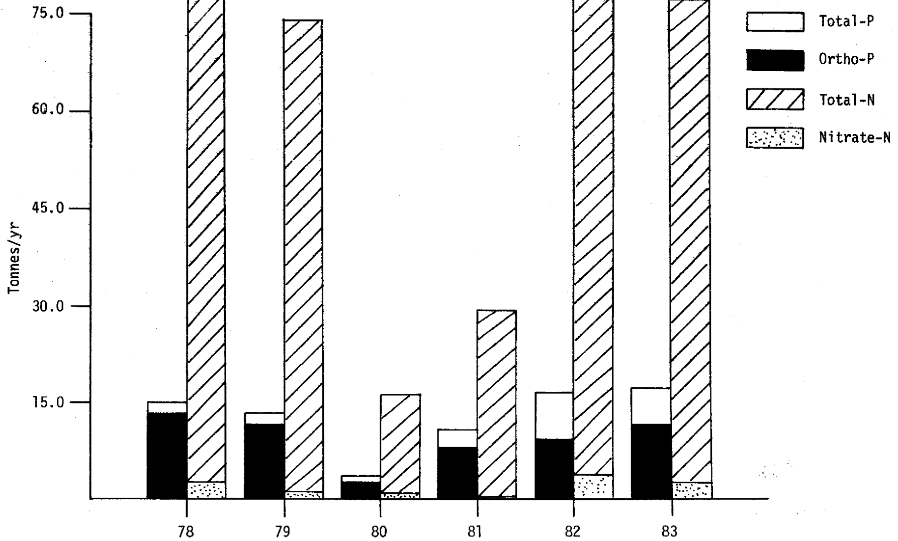
FIGURE 22. Williamson Ditch Annual Nutrient Loads 1978-1983
