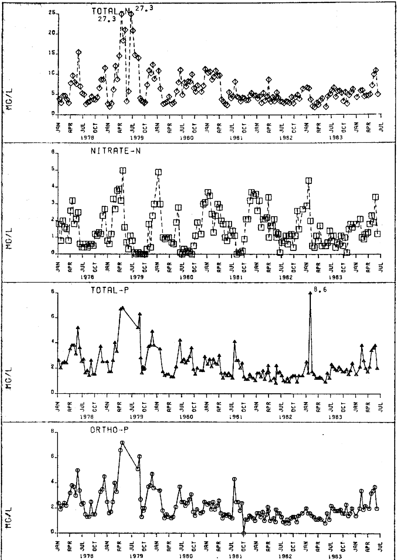
FIGURE MOSQUITO CREEK STATION 13
