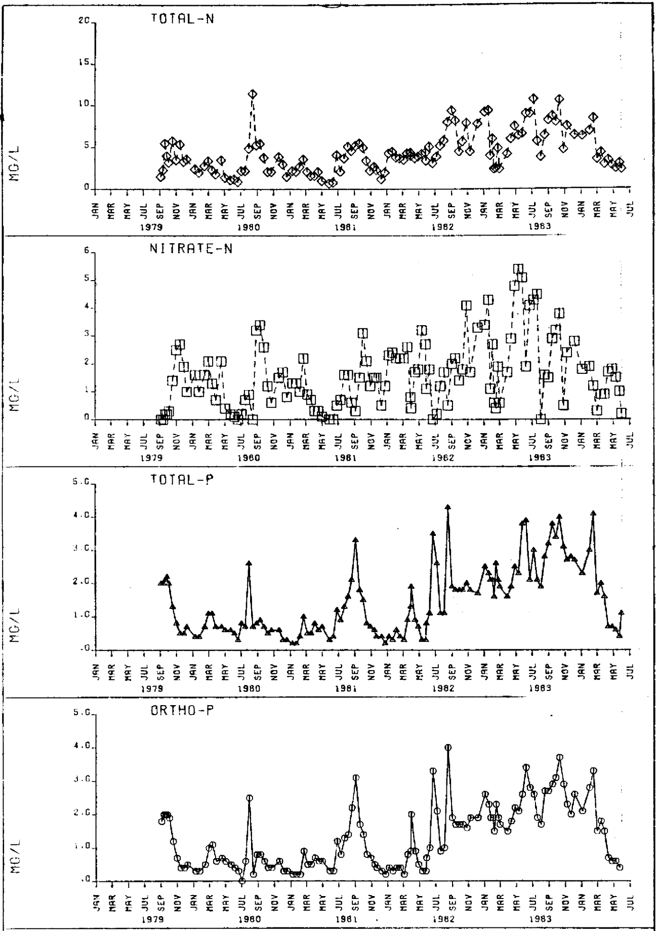
FIGURE LITTLE BIMINI STATION O2
