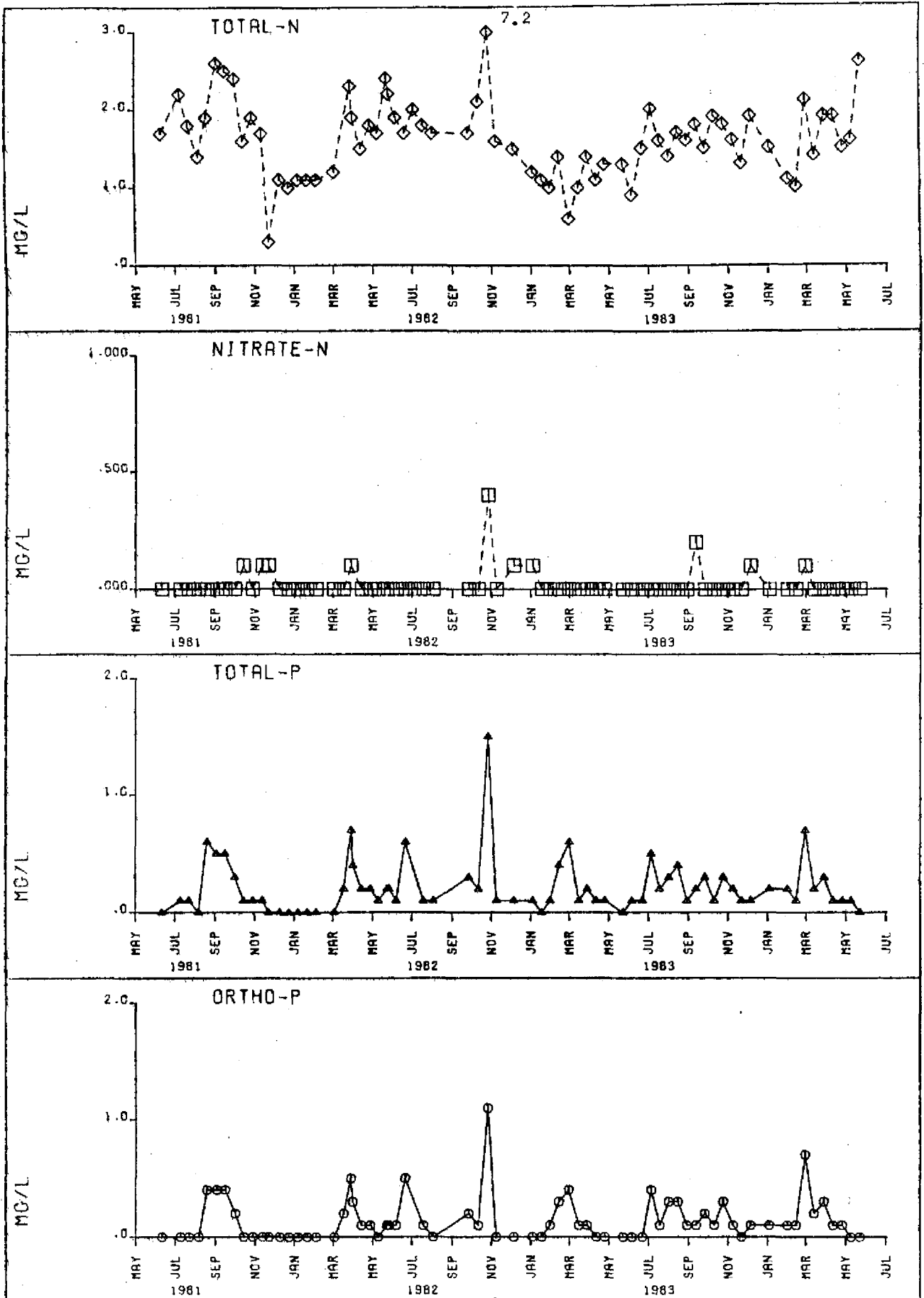
FIGURE LETTUCE CREEK STATION 40
