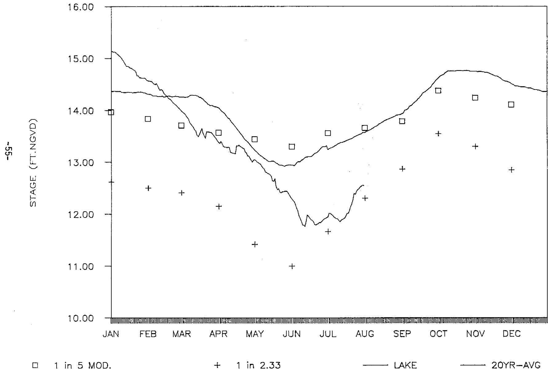
FIGURE 33. LAKE OKEECHOBEE OPERATIONAL LIMITS
