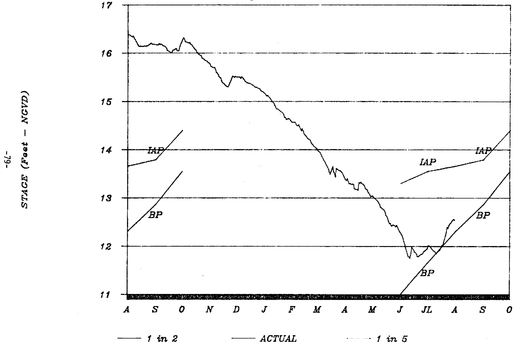
FIGURE 36. LAKE OKEECHOBEE STAGES
