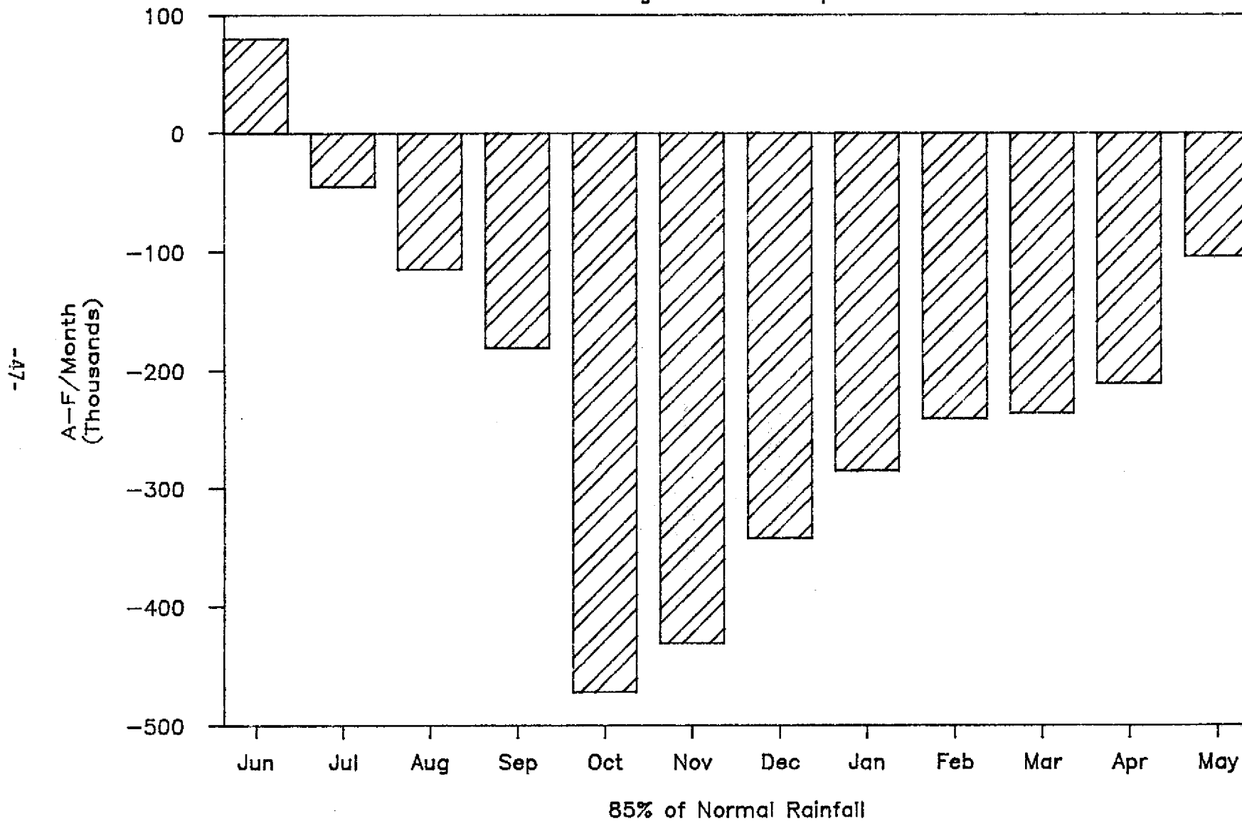
FIGURE 28. Lake Okeechobee Change in Storage (Backsummed)
