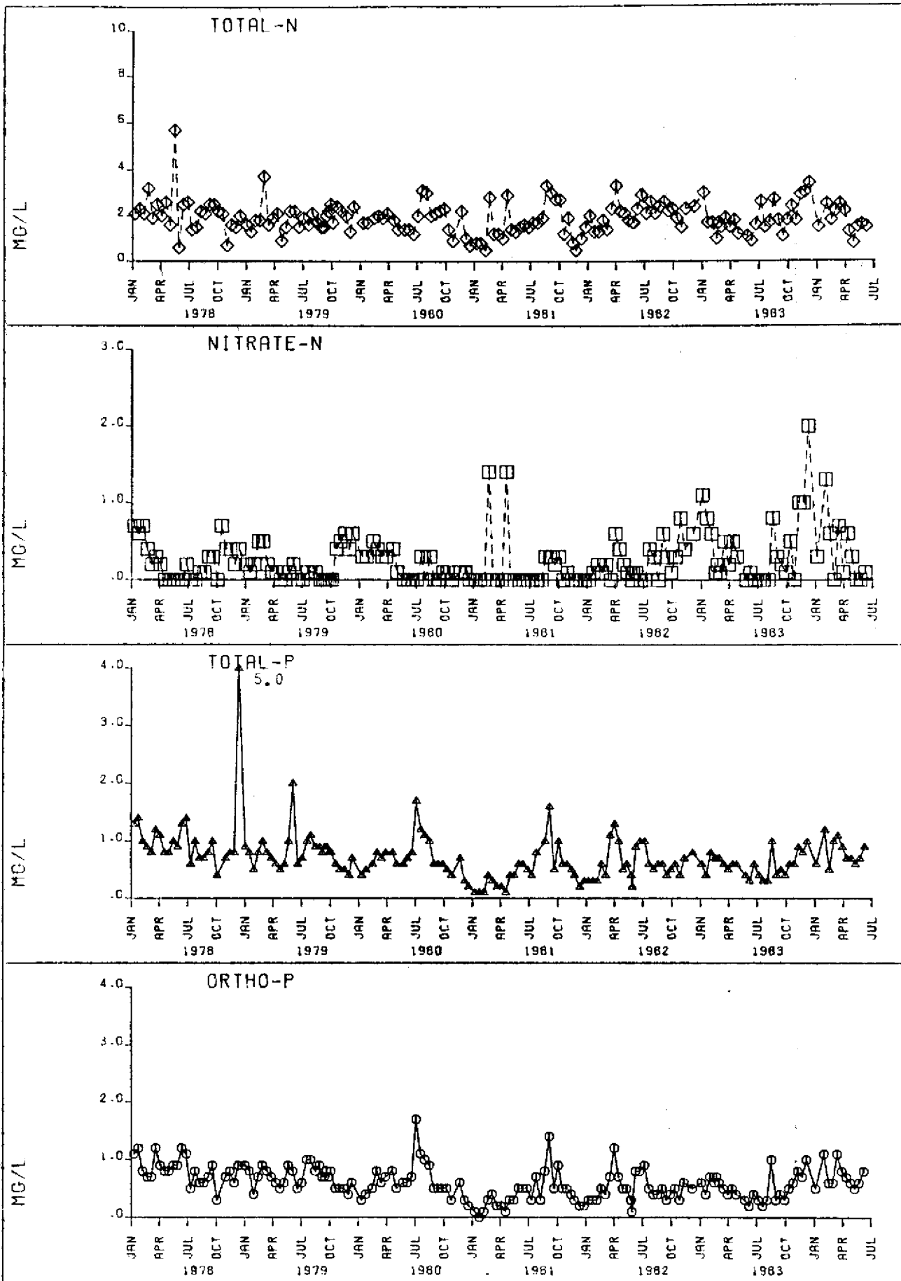
FIGURE UPPER TAYLOR CREEK STATION 11
