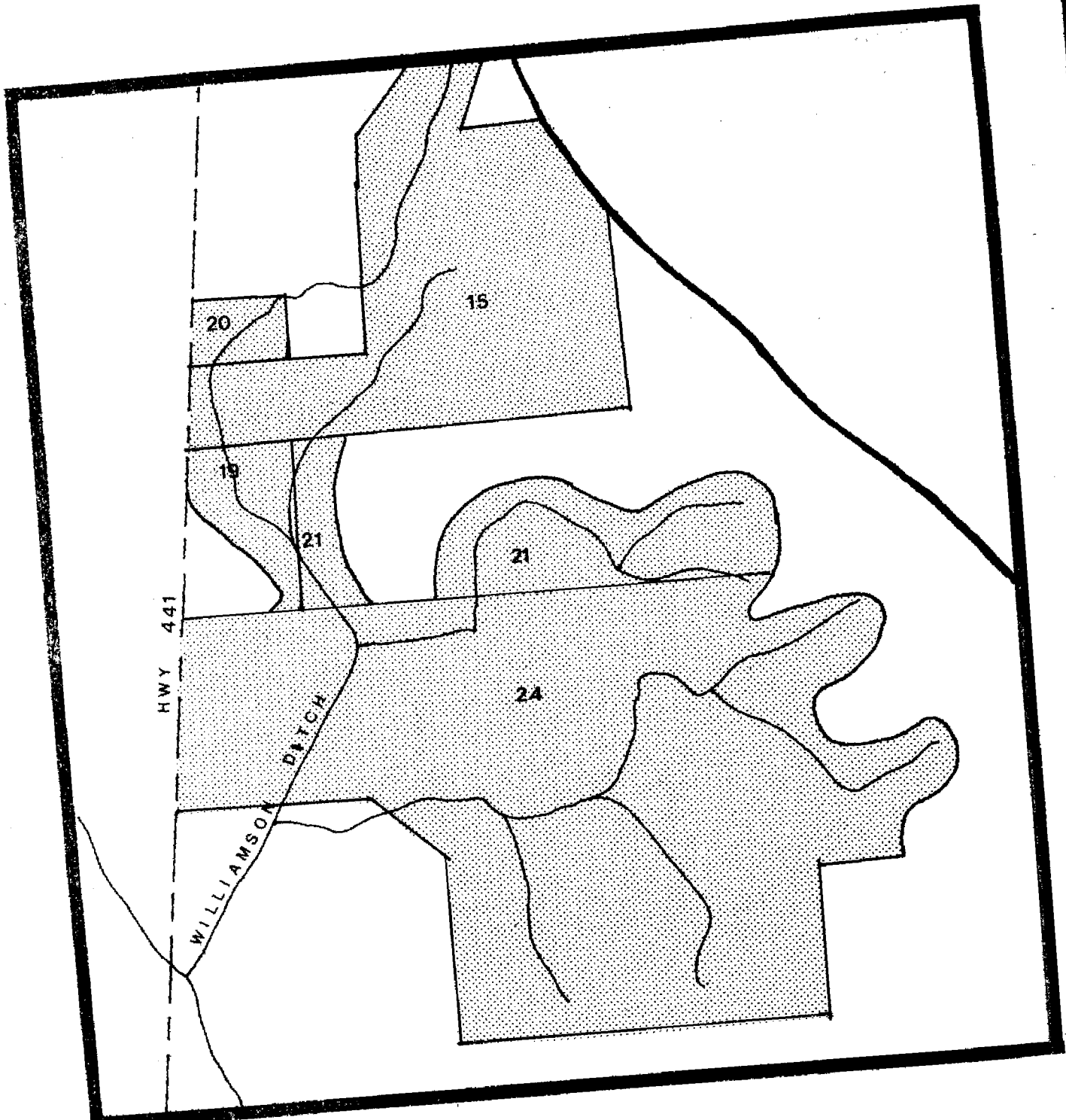
FIGURE 14. WILLIAMSON DITCH SUB-WATERSHED CRITICAL AREA CONTRACTED
