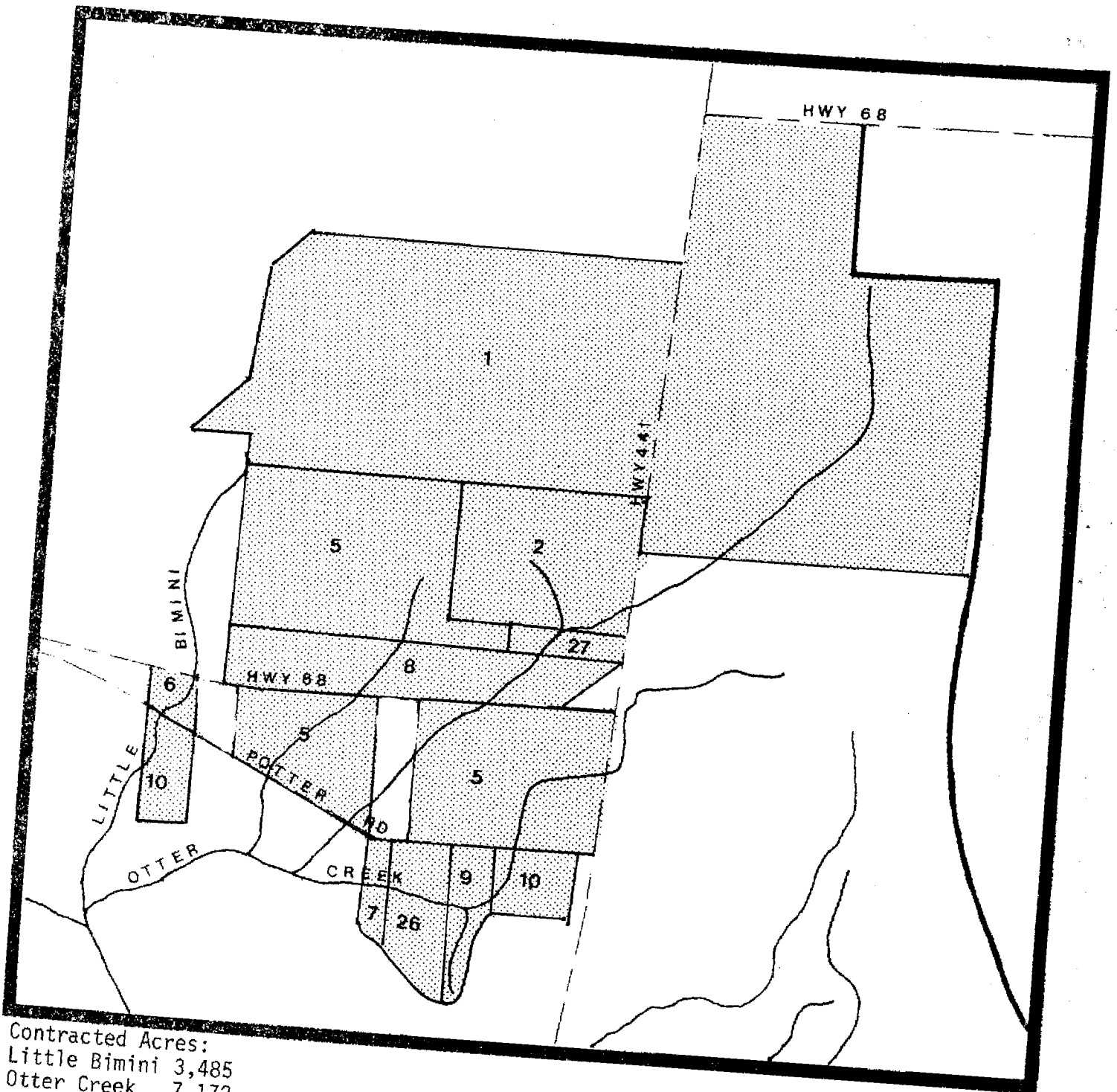
FIGURE 12. LITTLE BIMINI AND OTTER CREEK SUB-WATERSHEDS CRITICAL AREA CONTRACTED
