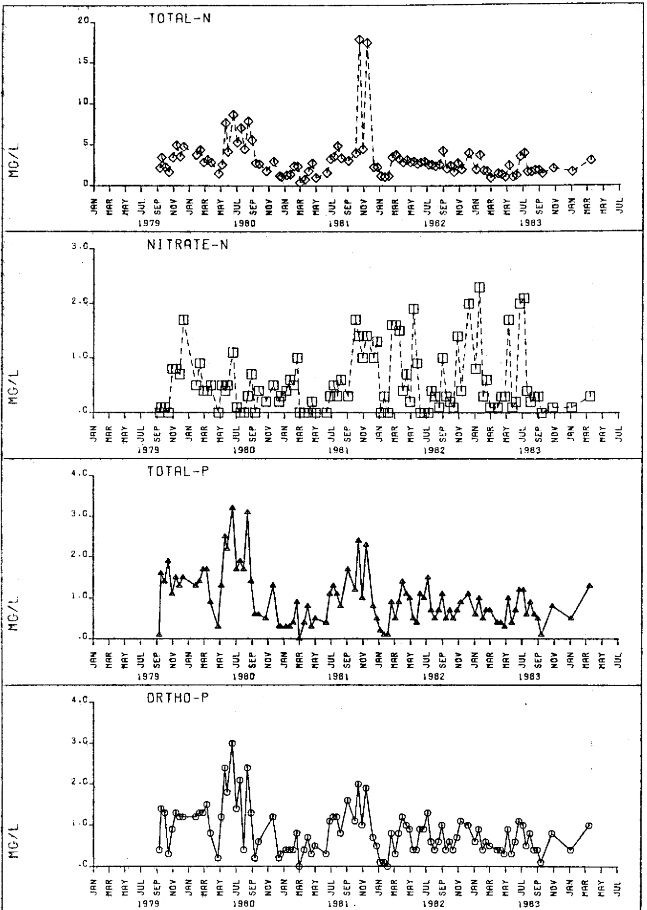
FIGURE HEADWATERS CONFLUENCE STATION 18
