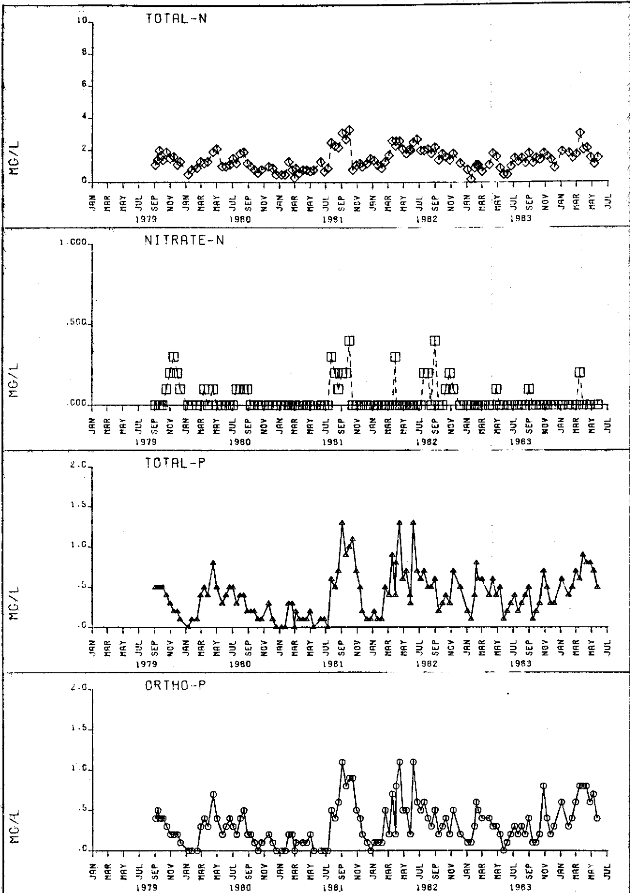
FIGURE N.W. TAYLOR CREEK STATION 01
