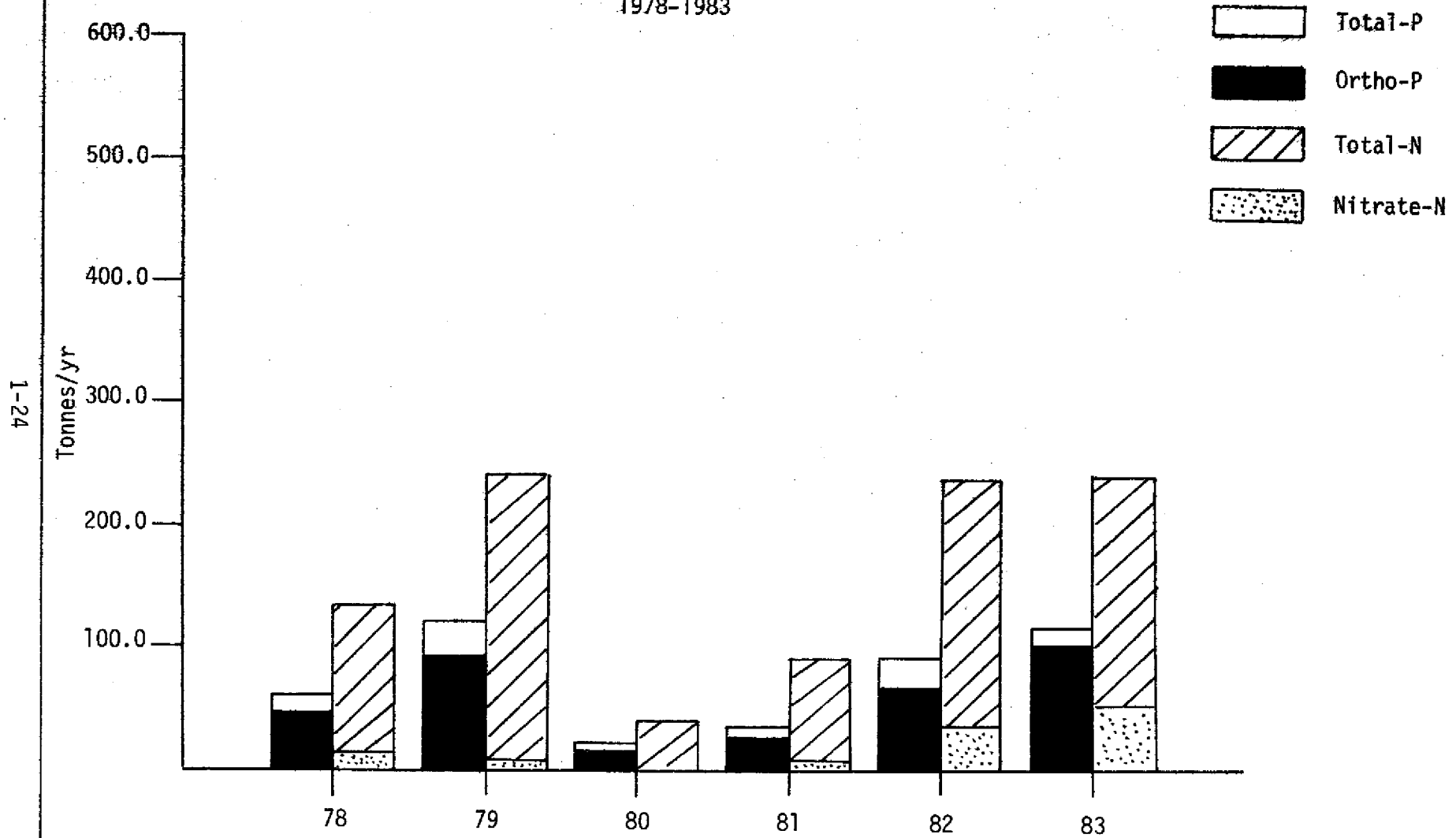
FIGURE 24. Upper Taylor Creek Annual Nutrient Loads 1978-1983
