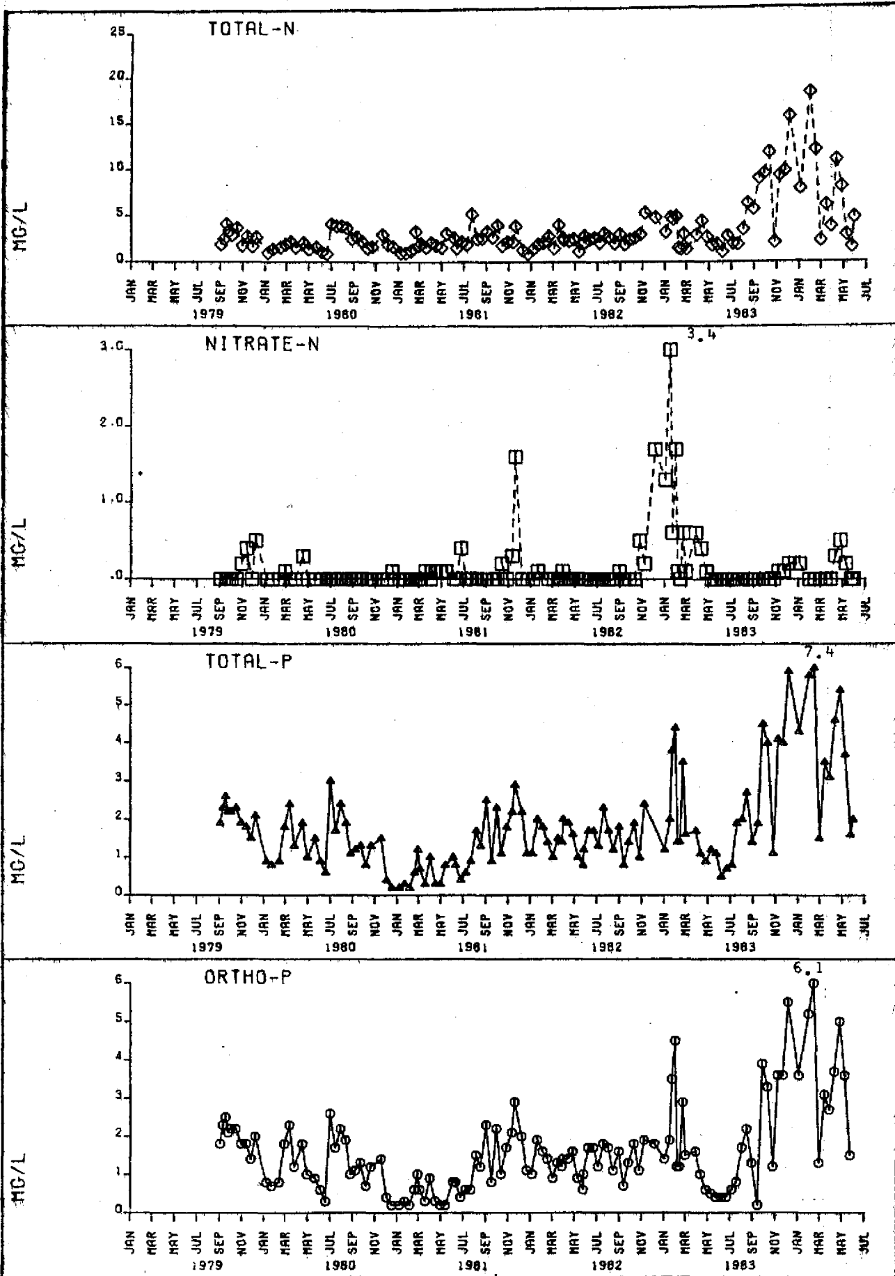
FIGURE OTTER CREEK STATION 03
