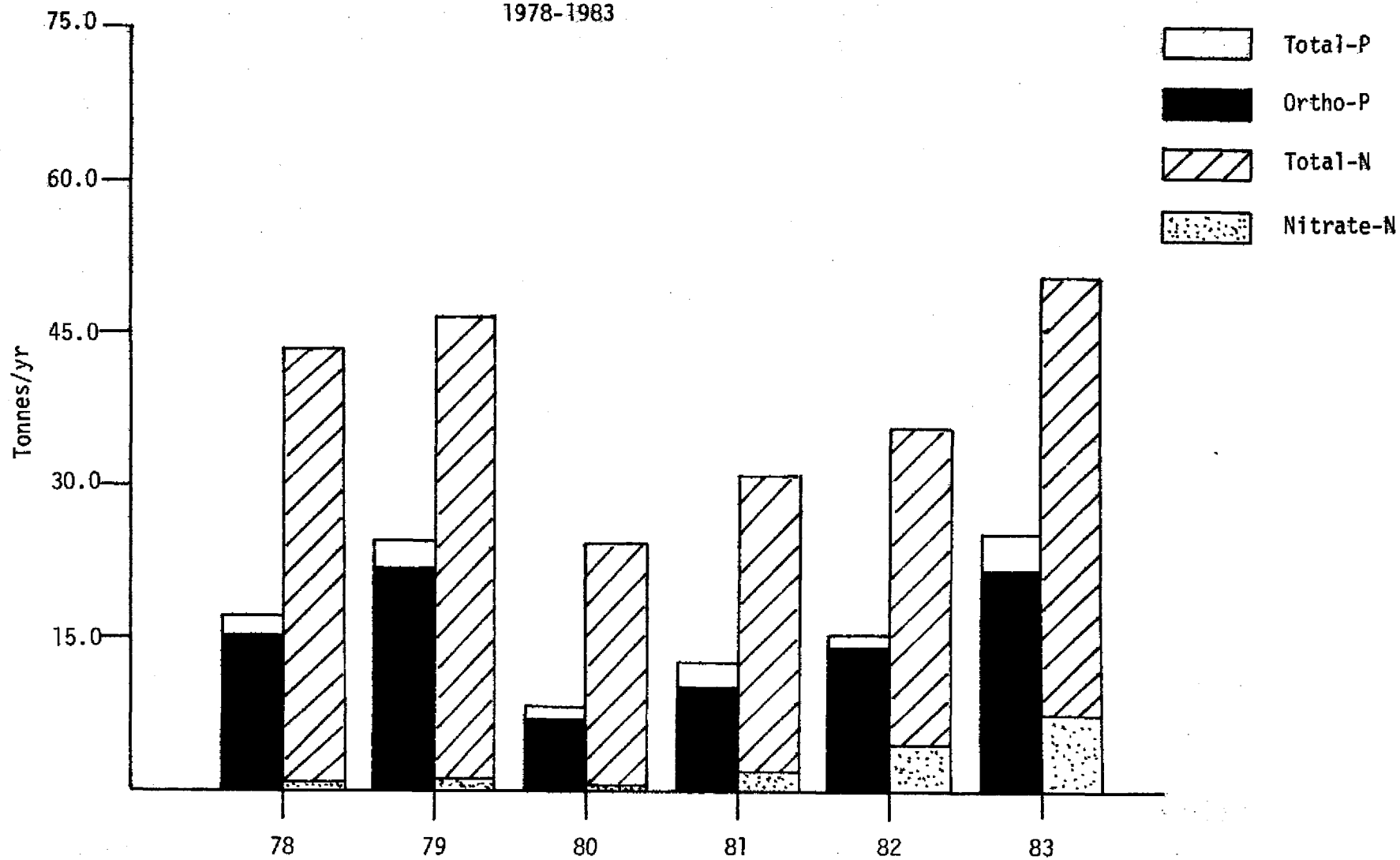
FIGURE 19. Otter Creek Annual Nutrient Loads 1978-1983
