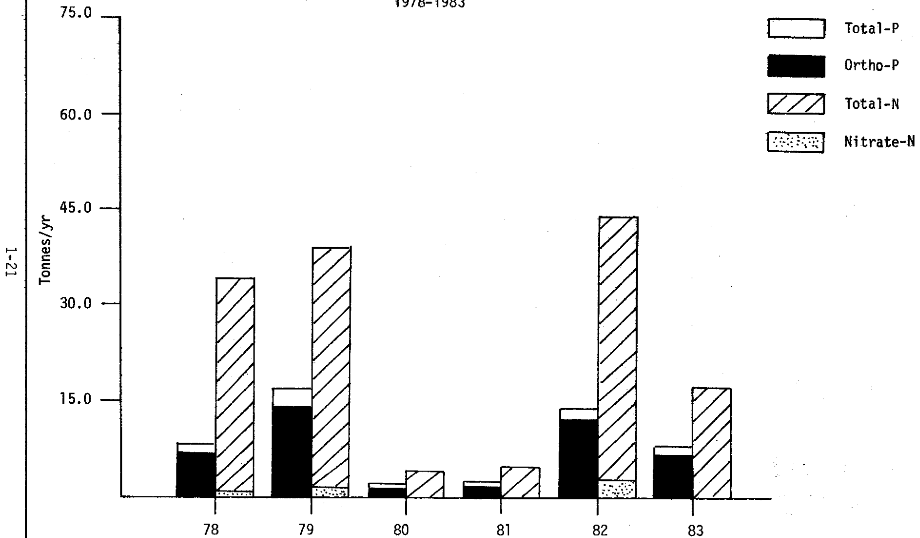
FIGURE 21. N. W. Taylor Creek Annual Nutrient Loads 1978-1983
