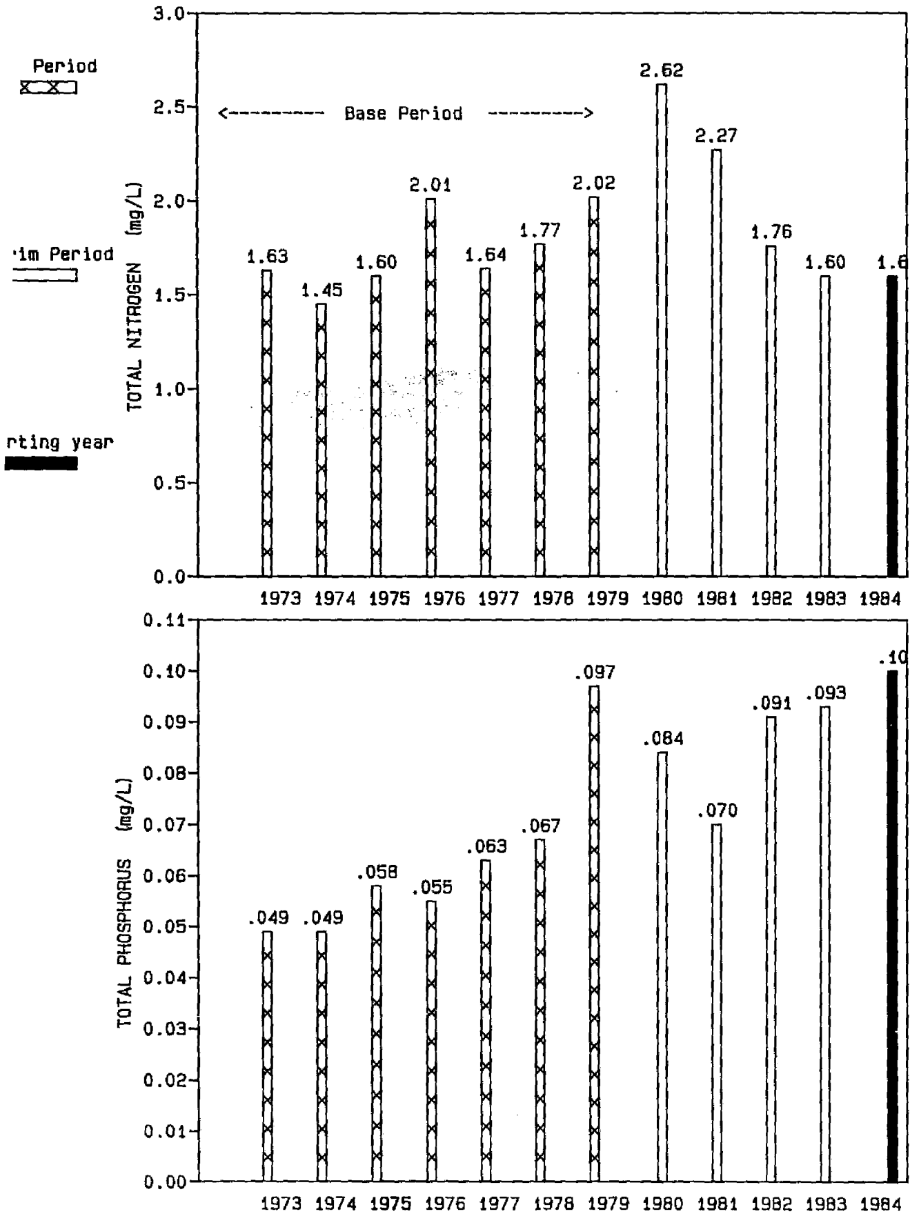
FIGURE 35. MEAN ANNUAL LAKE OKEECHOBEE TOTAL N AND TOTAL P CONCENTRATIONS
