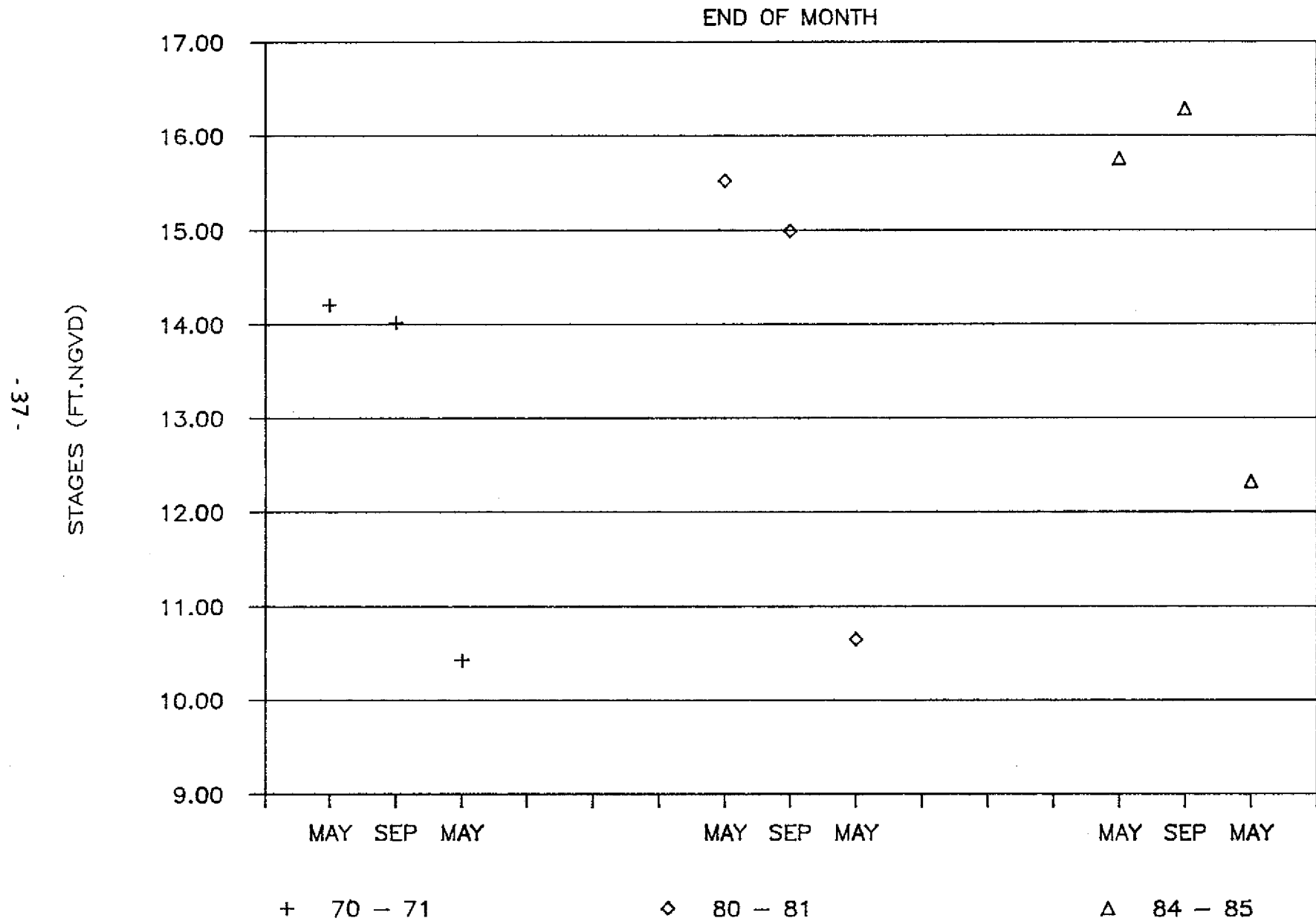
Figure 22 LAKE OKEECHOBEE HISTORICAL STAGES
