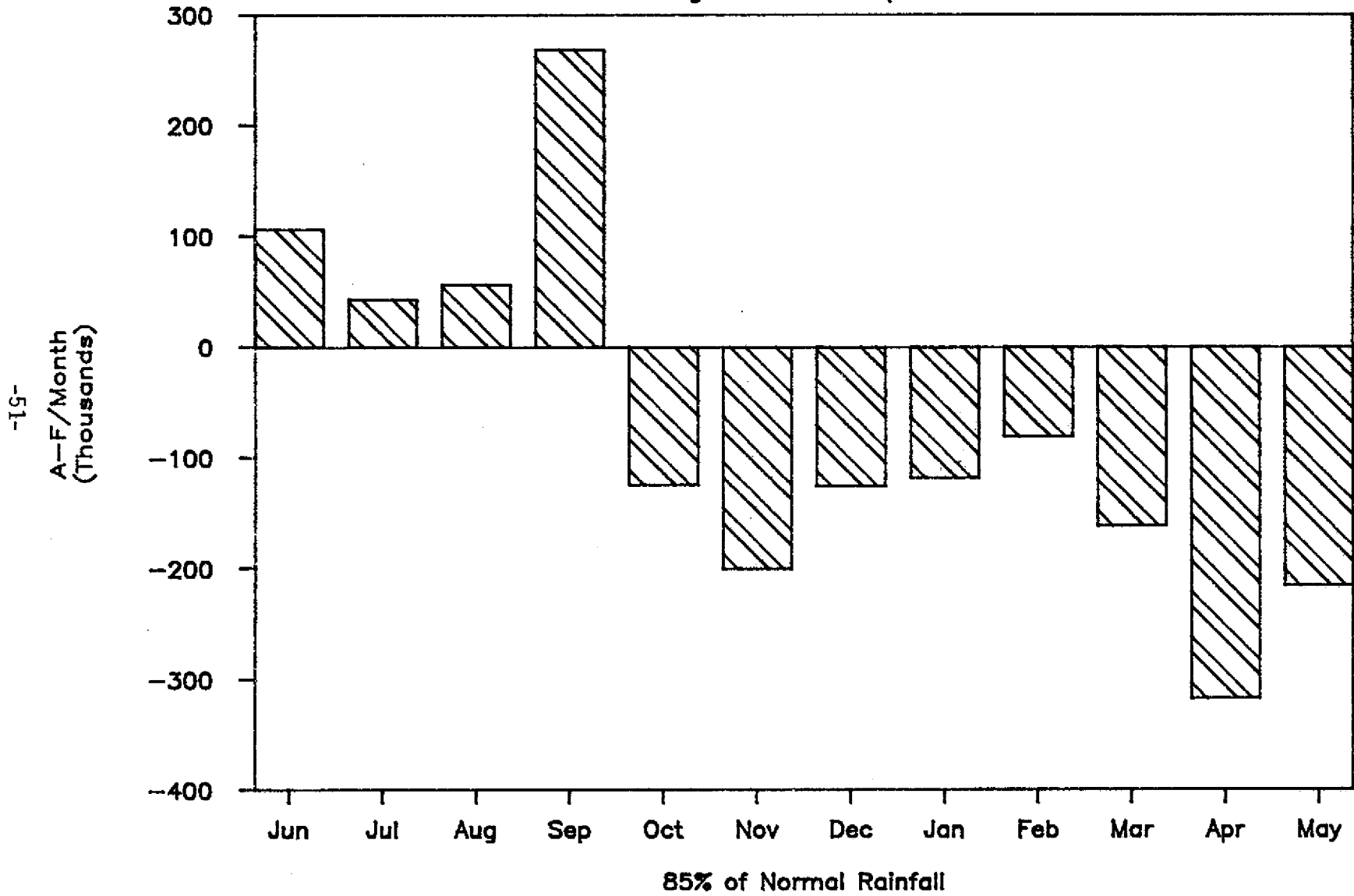
FIGURE 30. Lake Okeechobee Required Storage Including Water Use Requirements
