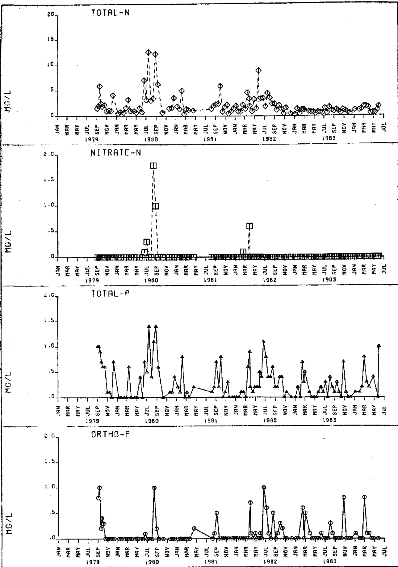
FIGURE EAST OTTER CREEK STATION 19
