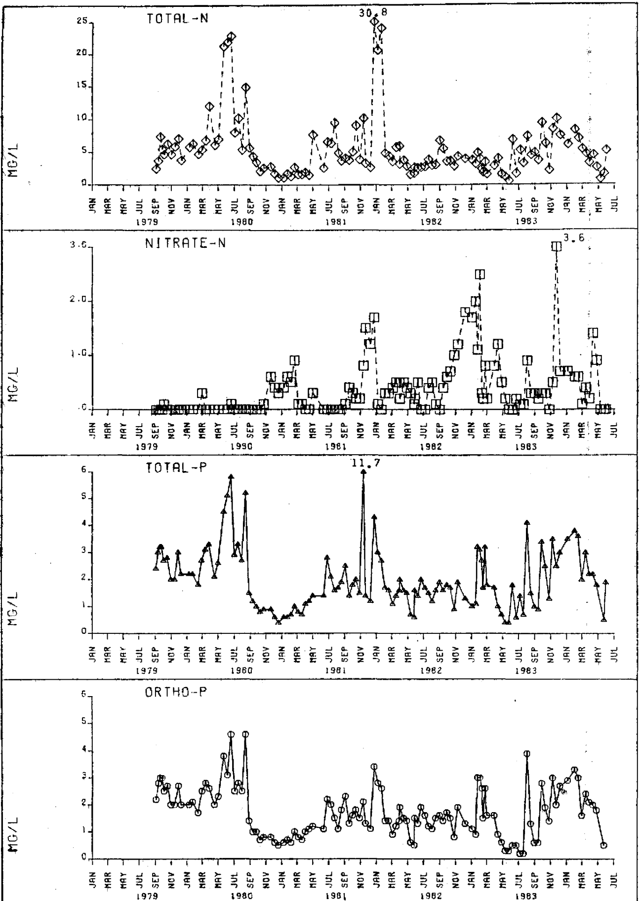
FIGURE OTTER CREEK STATION 06
