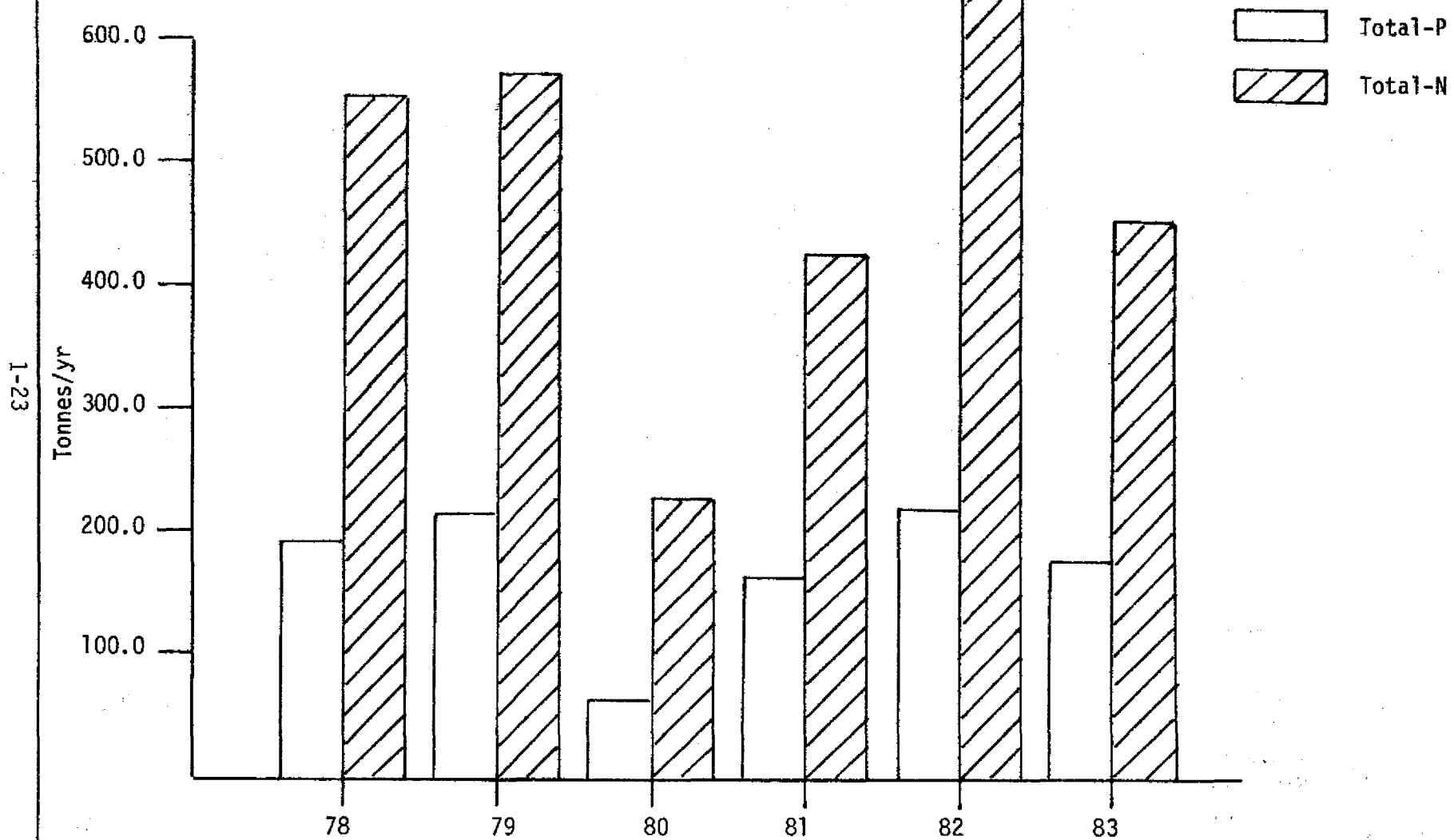
FIGURE 23. S-191 at Lake Okeechobee Annual Nutrient Loads 1978-1983
