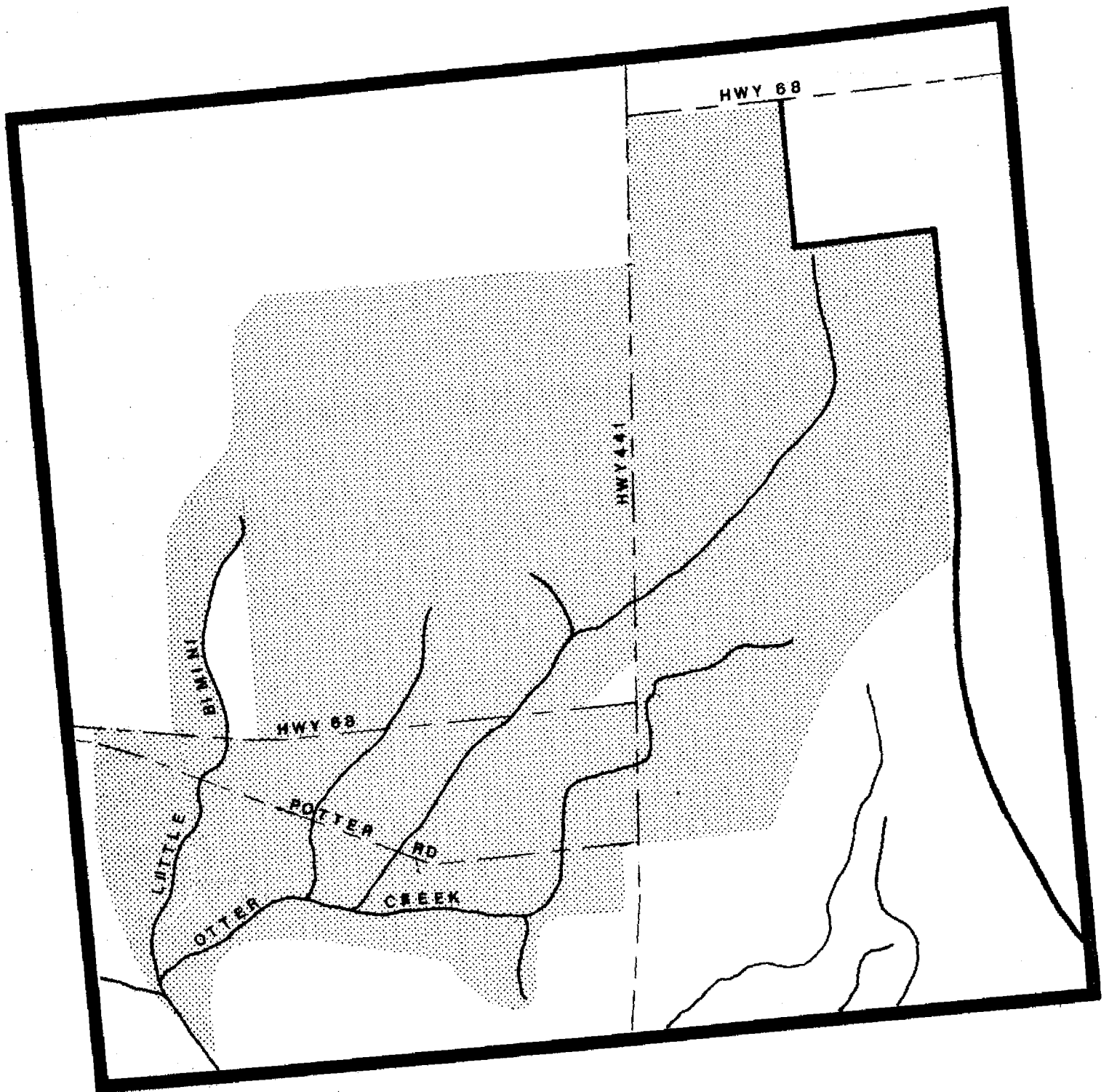
FIGURE 5. CRITICAL AREA IN LITTLE BIMINI AND OTTER CREEK SUB-WATERSHEDS
