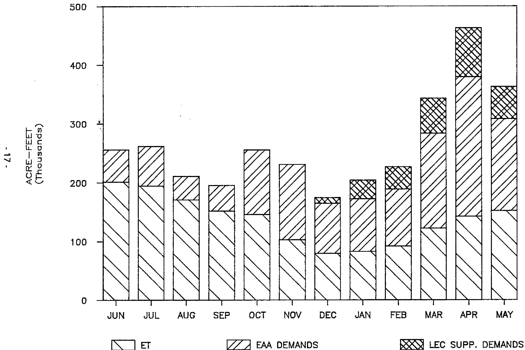
Figure 10 LAKE OKEECHOBEE PROJECTED WATER BUDGET
