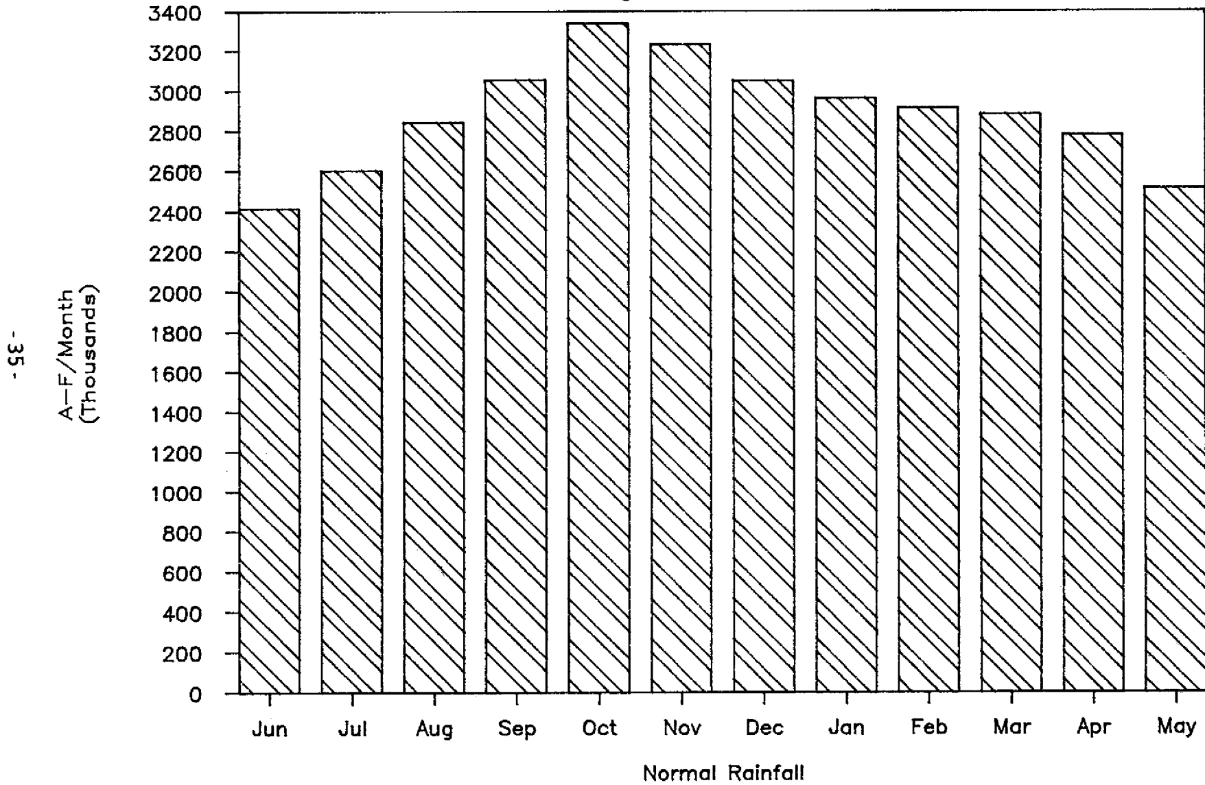
Figure 20 Lake Okeechobee Required Storage (Backsummed)
