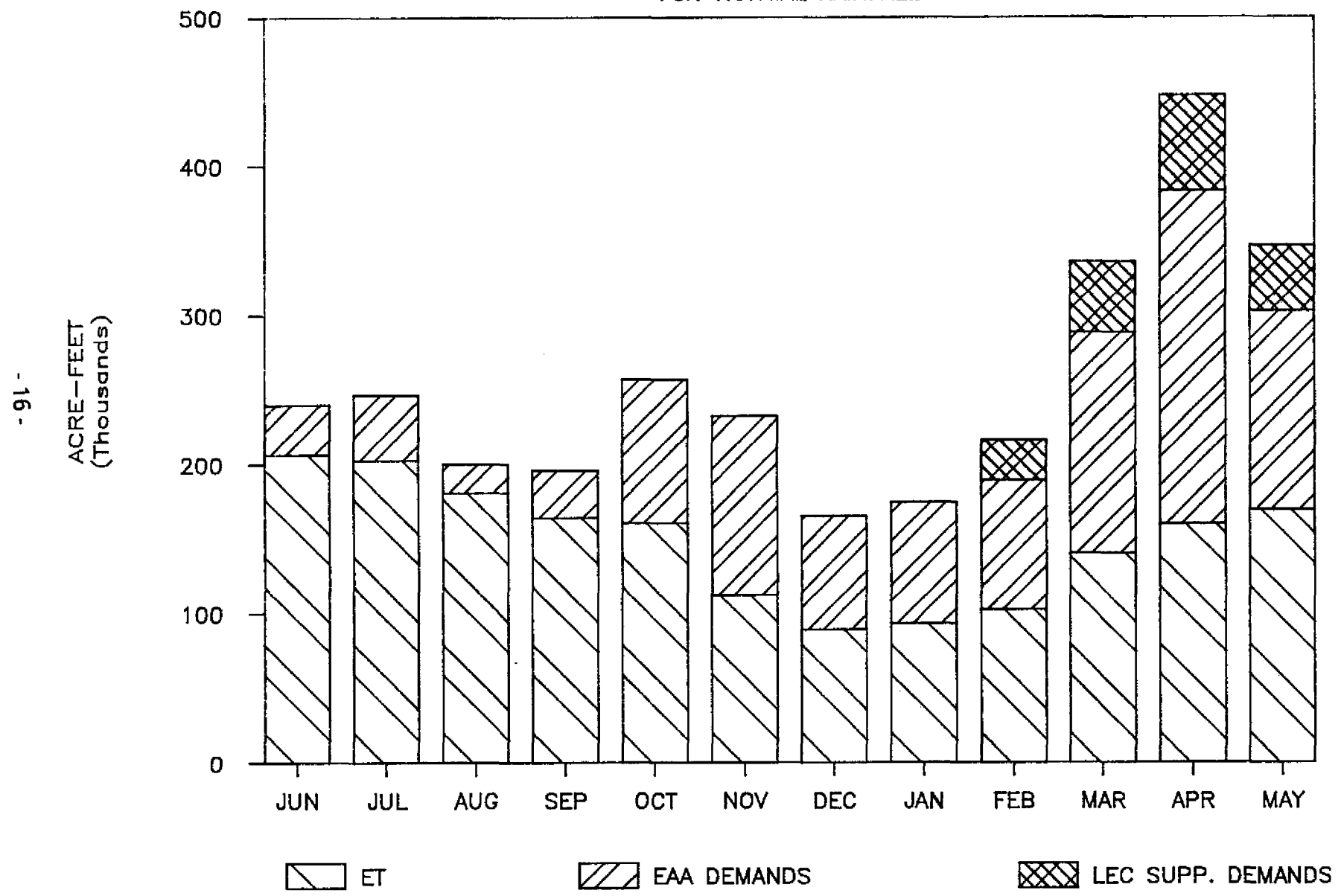
Figure 9 LAKE OKEECHOBEE PROJECTED WATER BUDGET
