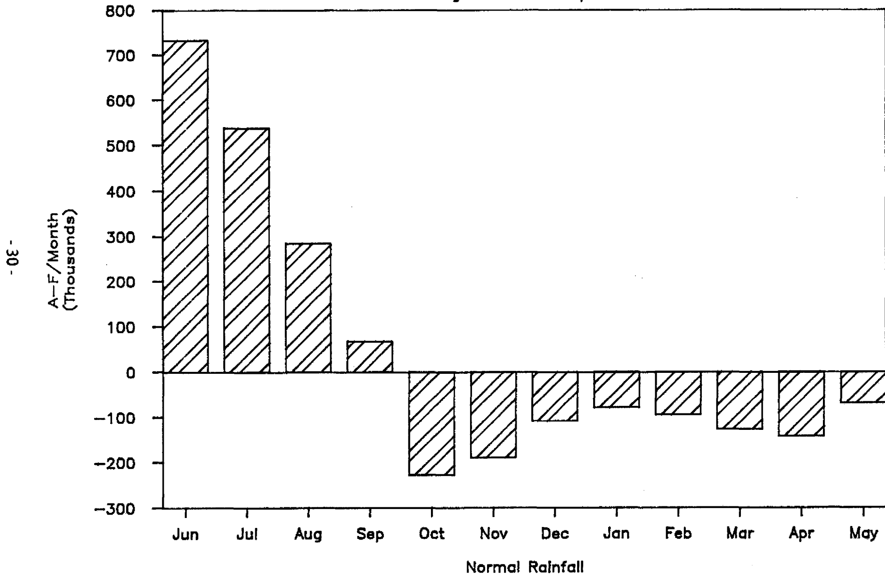
Figure 17 Lake Okeechobee Change in Storage (Backsummed)
