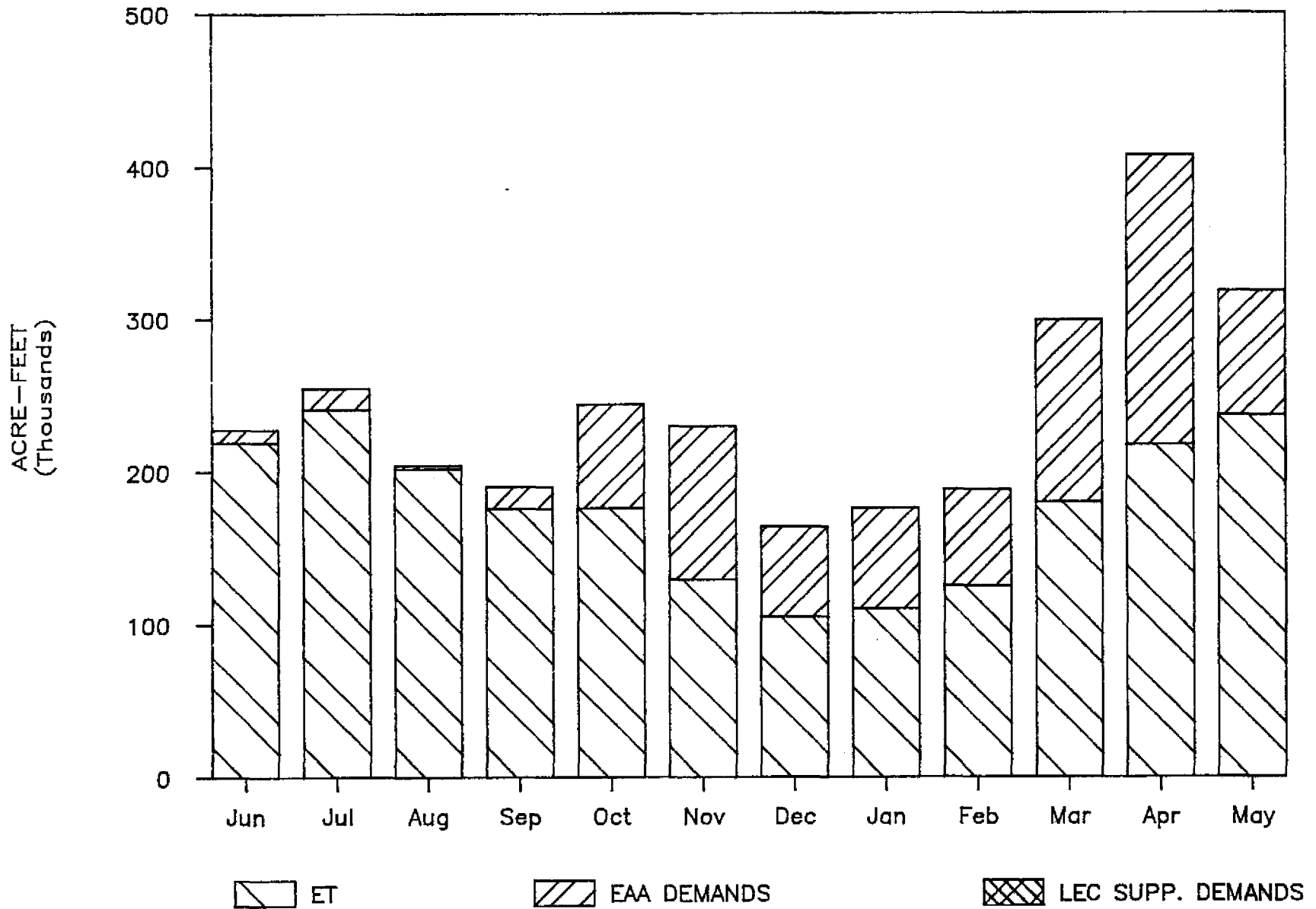
Figure 7 LAKE OKEECHOBEE PROJECTED WATER BUDGET
