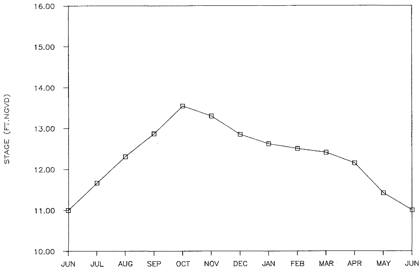
Figure 23 LAKE OKEECHOBEE OPERATIONAL LIMITS
