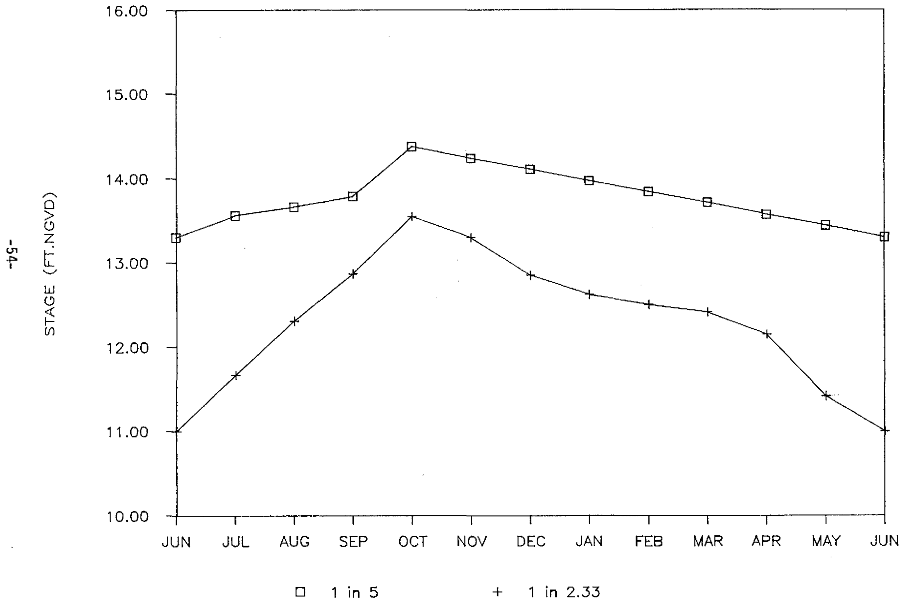
FIGURE 32. LAKE OKEECHOBEE OPERATIONAL LIMITS
