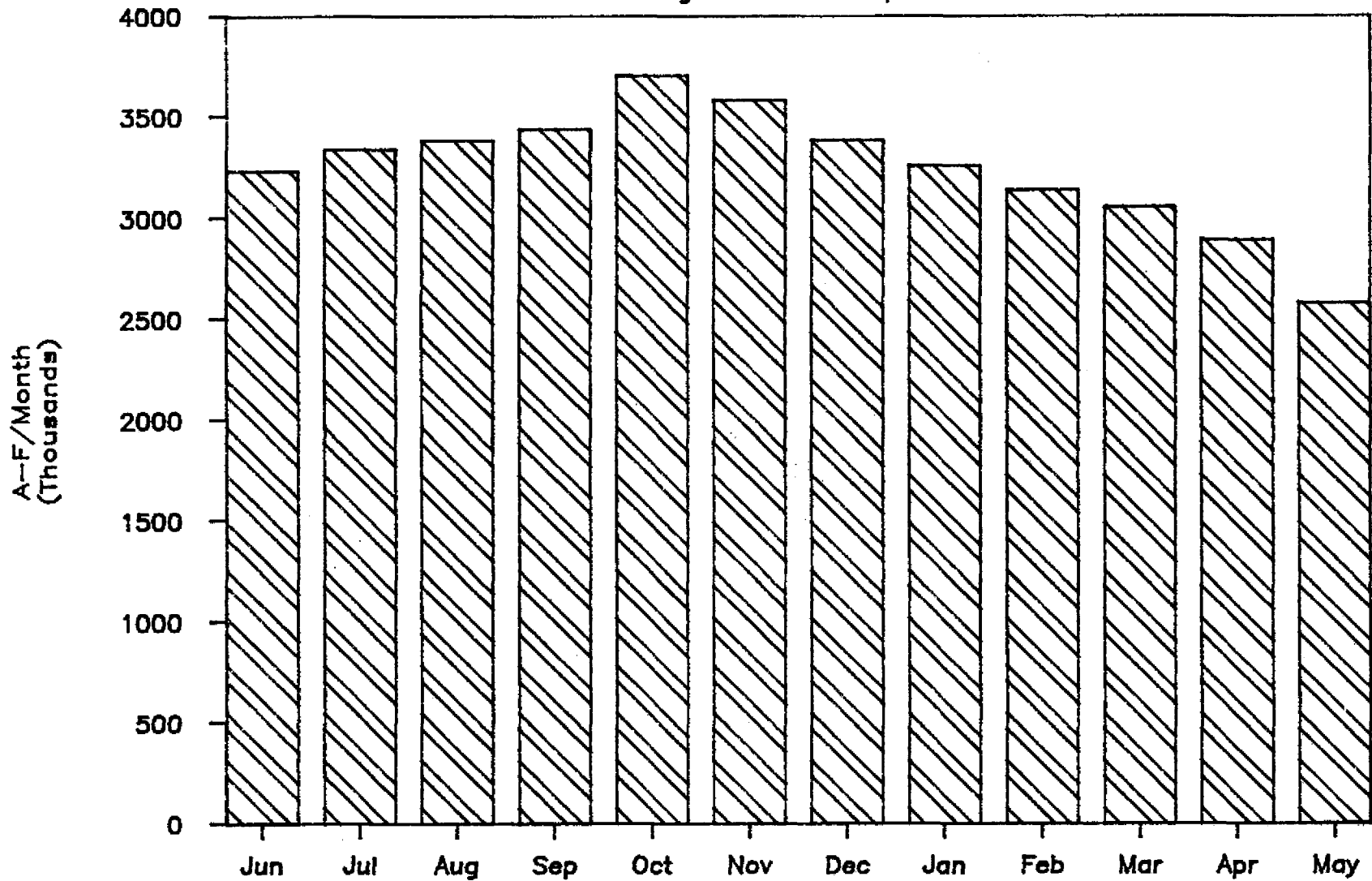
FIGURE 31. Lake Okeechobee Required Storage (Backsummed)
