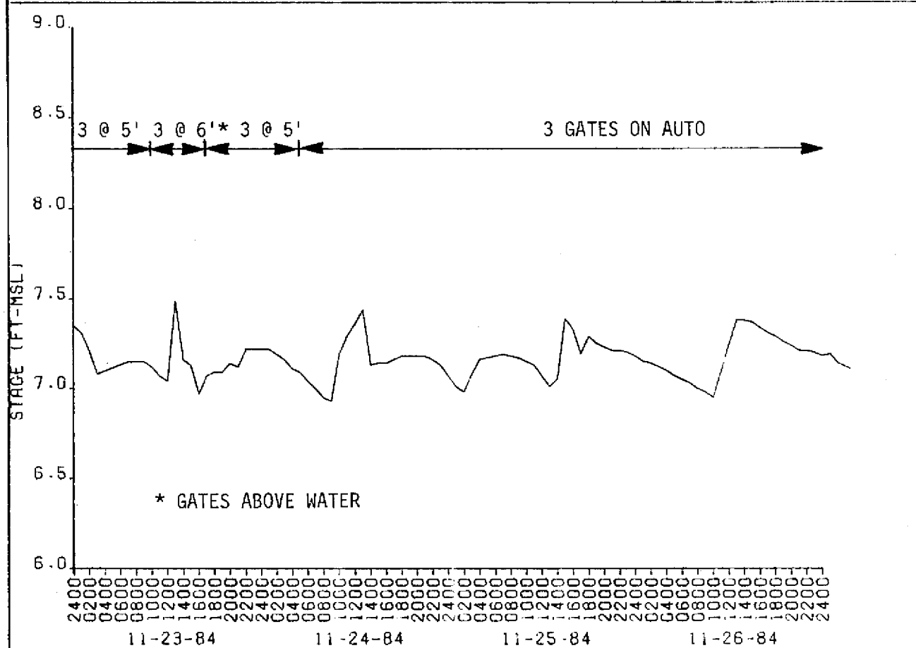
FIG. 8 HOURLY STAGE READINGS AT S-155HW
