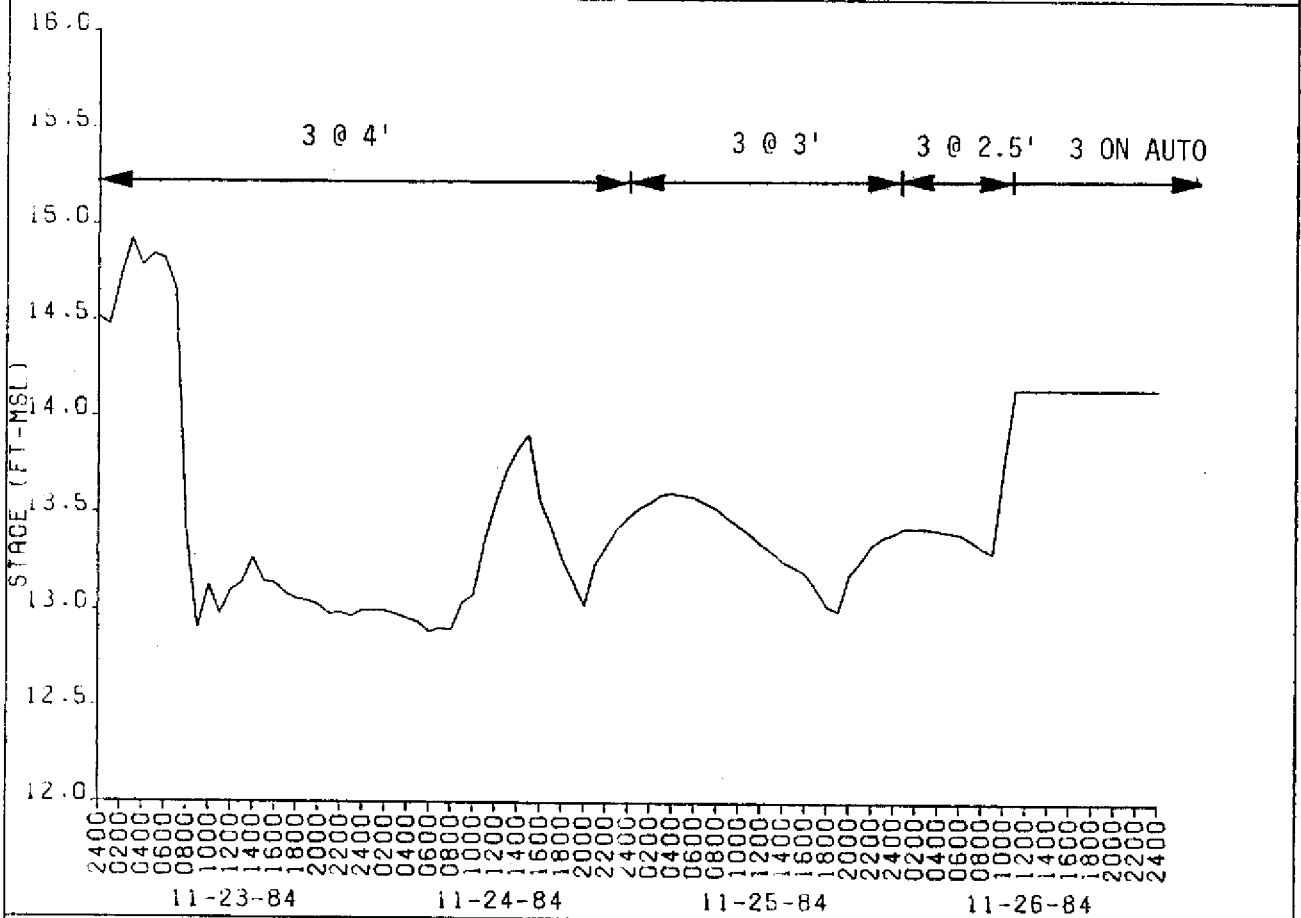
FIG. 11 HOURLY STAGE READINGS AT S-46HW
