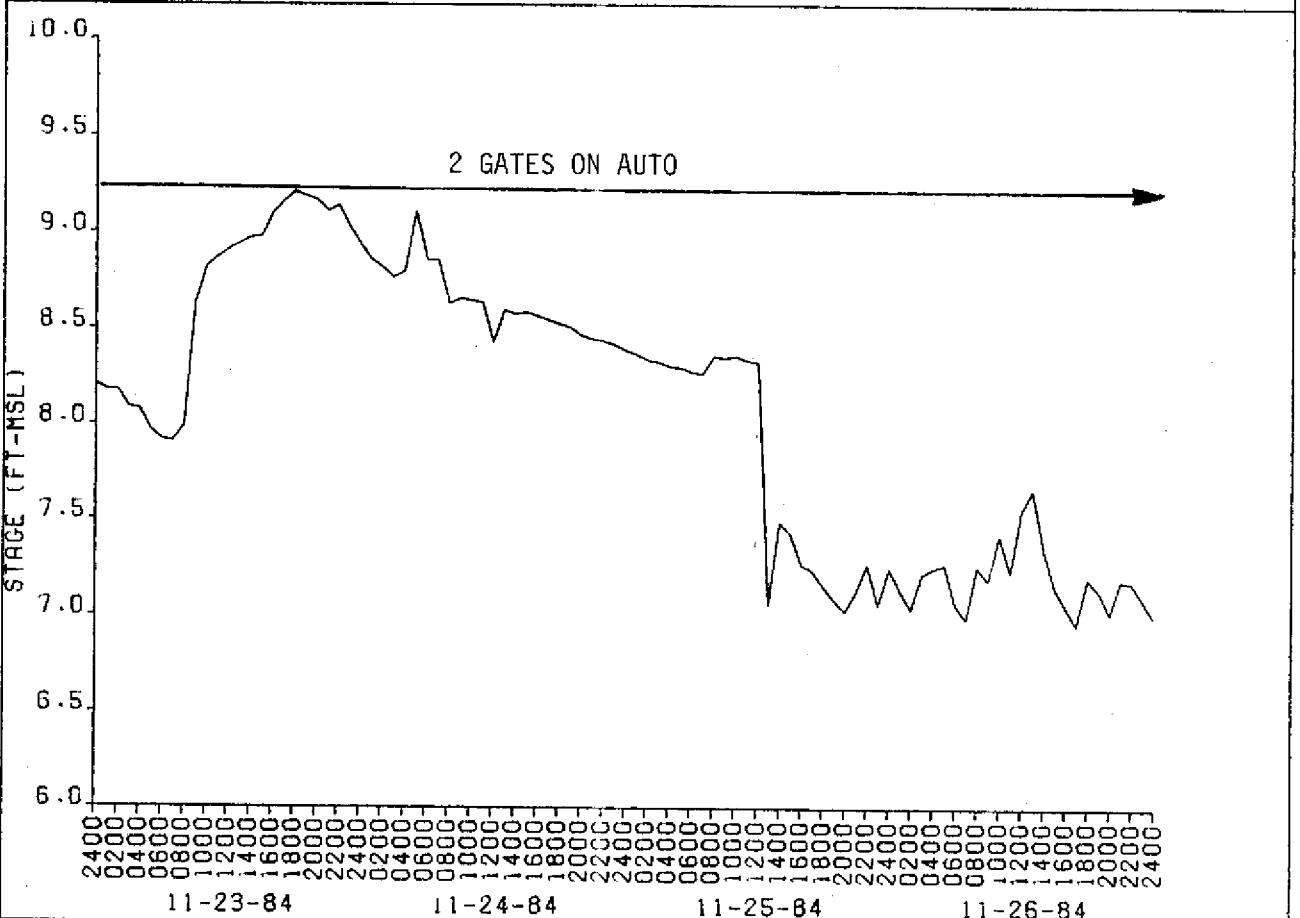
FIG. 10 HOURLY STAGE READINGS AT S-44HW
