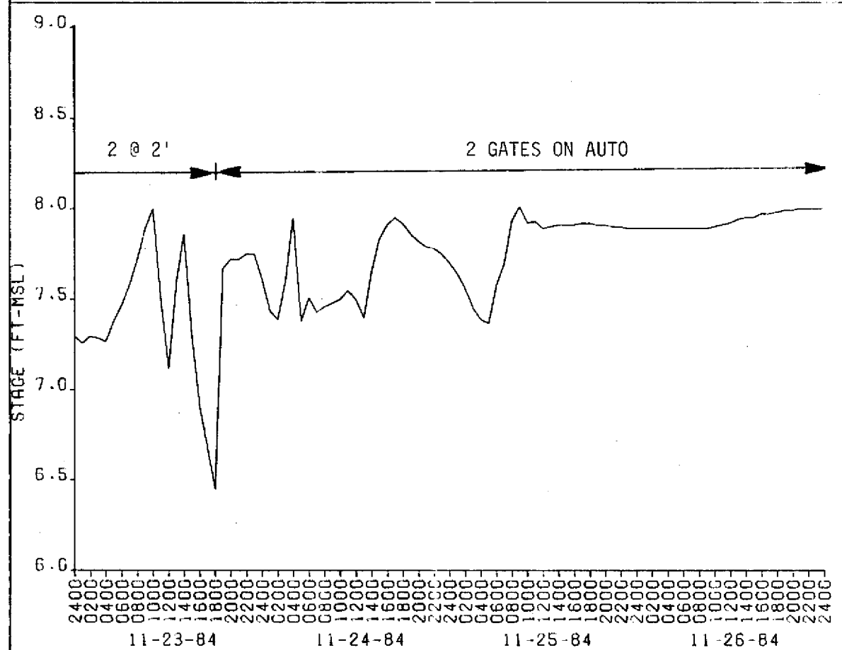
FIG. 9 HOURLY STAGE READINGS AT S-41HW
