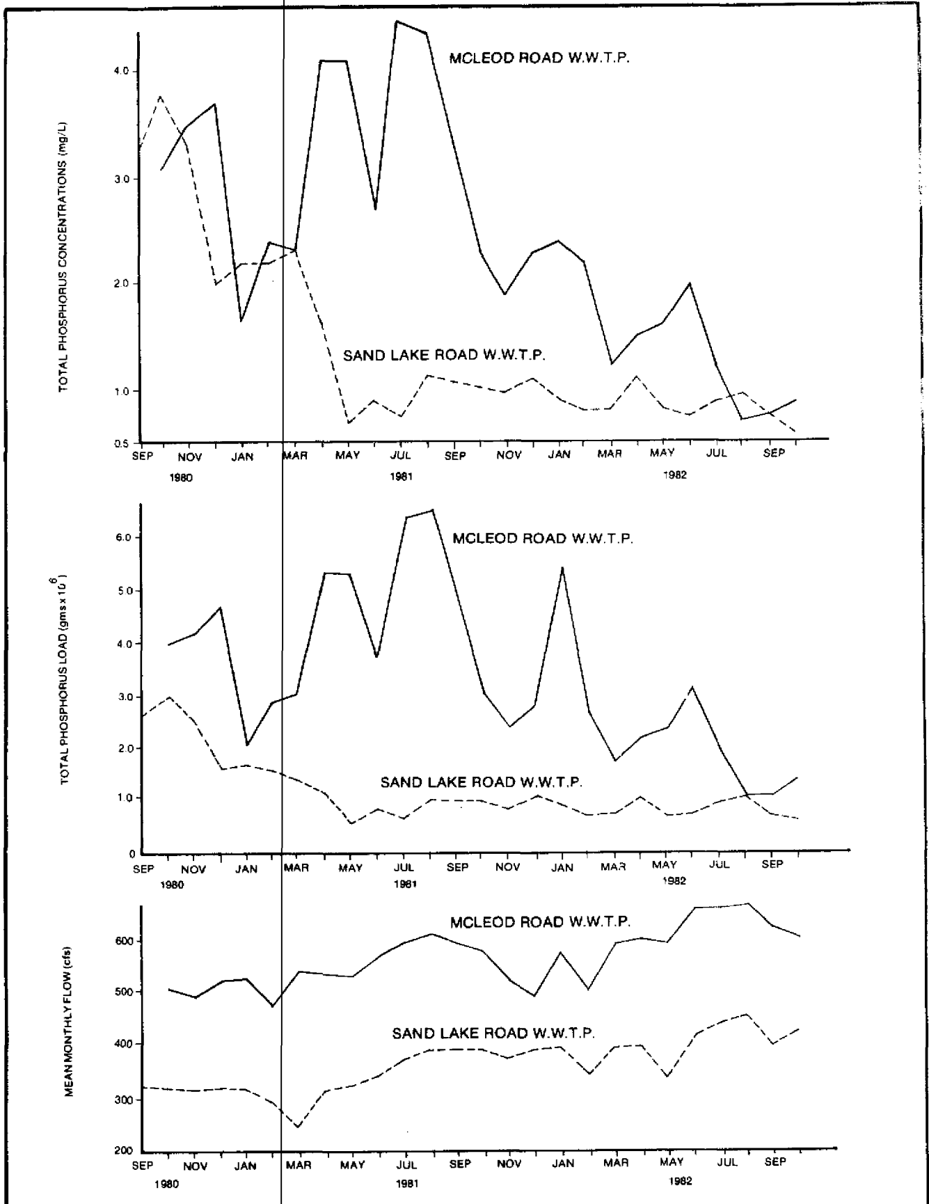
Fig. 8 MCLEOD ROAD AND SAND LAKE ROAD WASTE WATER TREATMENT PLANT PHOSPHORUS AND AVERAGE DISCHARGE DATA.
