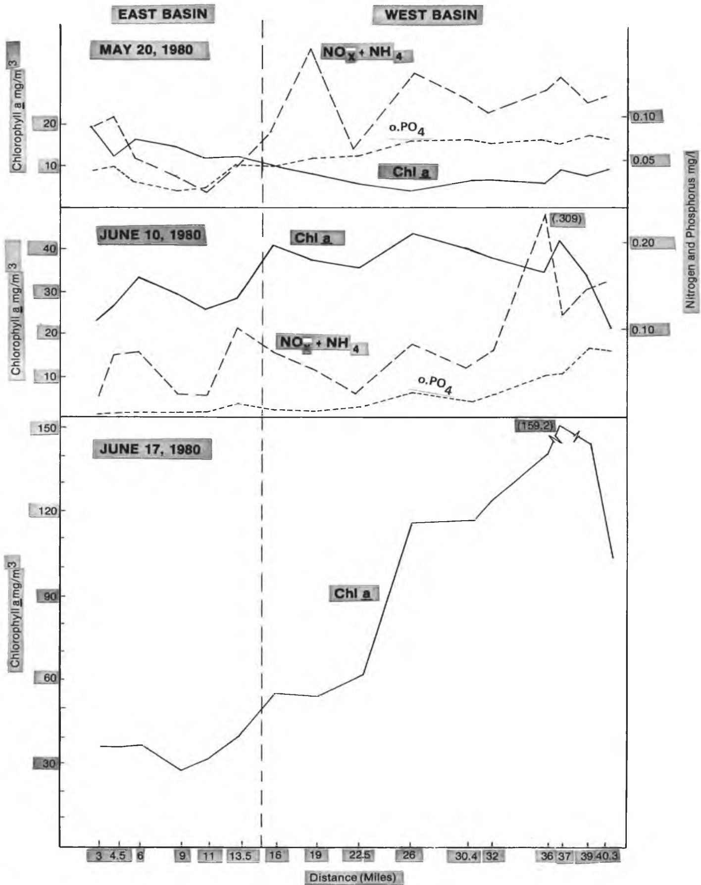
Figure 42 CHLOROPHYLL A AND INORGANIC NUTRIENT LEVEL ALONG C-43 PRIOR TO AND DURING A NUISANCE ALGAL BLOOM, 1980
