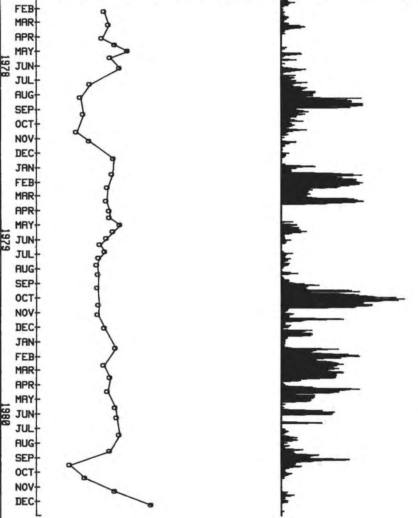
CHLORIDE CONCENTRATION AND DAILY DISCHARGE AT S-79 (CR-40.3)
