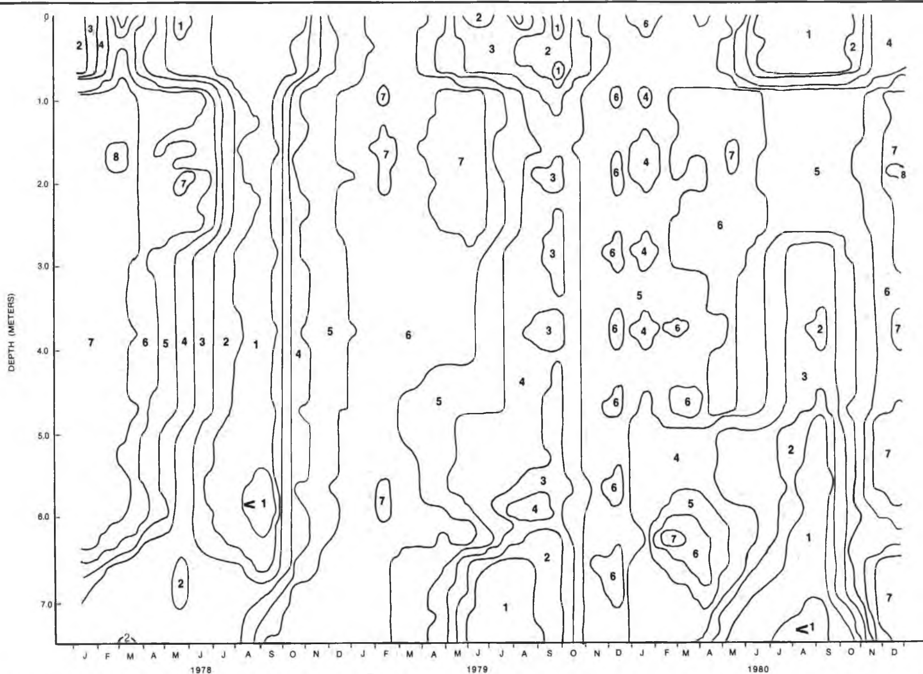
Figure 33 DEPTH-TIME DIAGRAM OF ISOPLETHS OF DISSOLVED OXYGEN CONCENTRATION IN MILLIGRAMS·LITER -1 AT STATION CR-06.0 EAST BASIN 1978-1980
