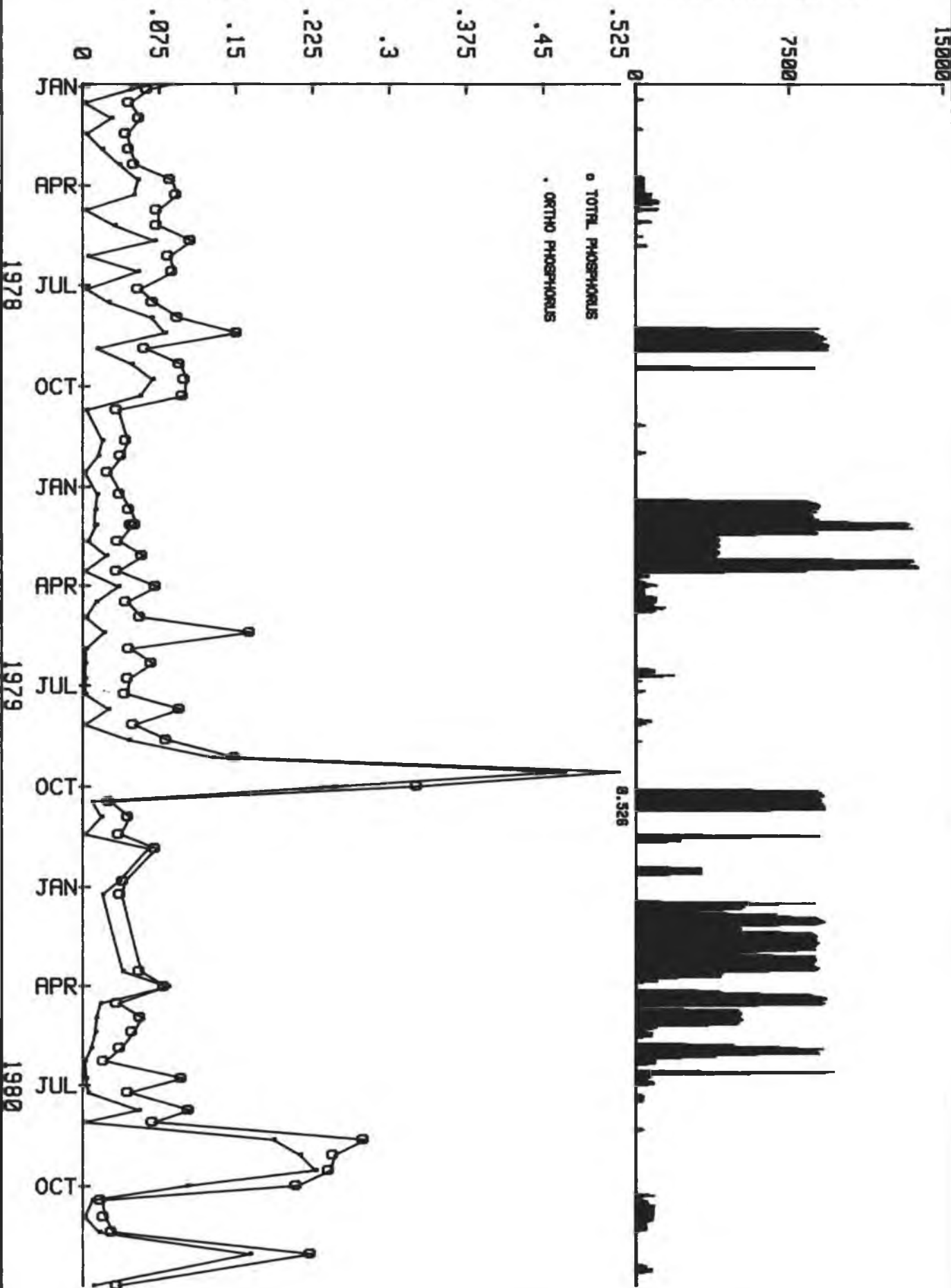
Figure 17 PHOSPHORUS CONCENTRATIONS AND DAILY DISCHARGE AT S-77
