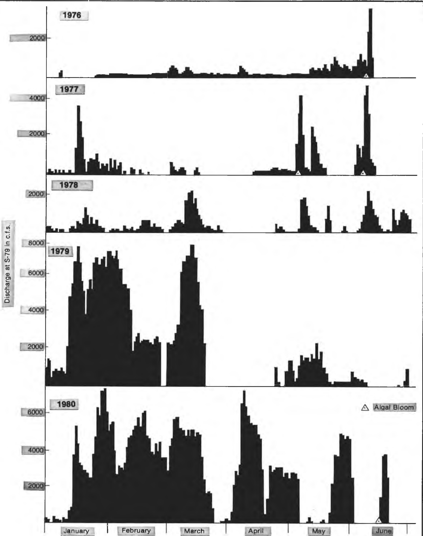
Figure 41 ANTECEDENT WATER FLOW CONDITIONS (AS MEASURED AT S-79) DURING ALGAL BLOOM AND NON-BLOOM YEARS 1976-1980
