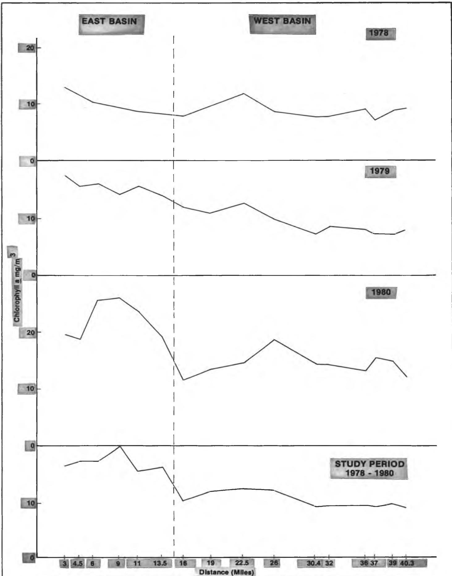
Figure 35 MEAN CHLOROPHYLL A CONCENTRATION VS SAMPLE STATION, 1978-1980
