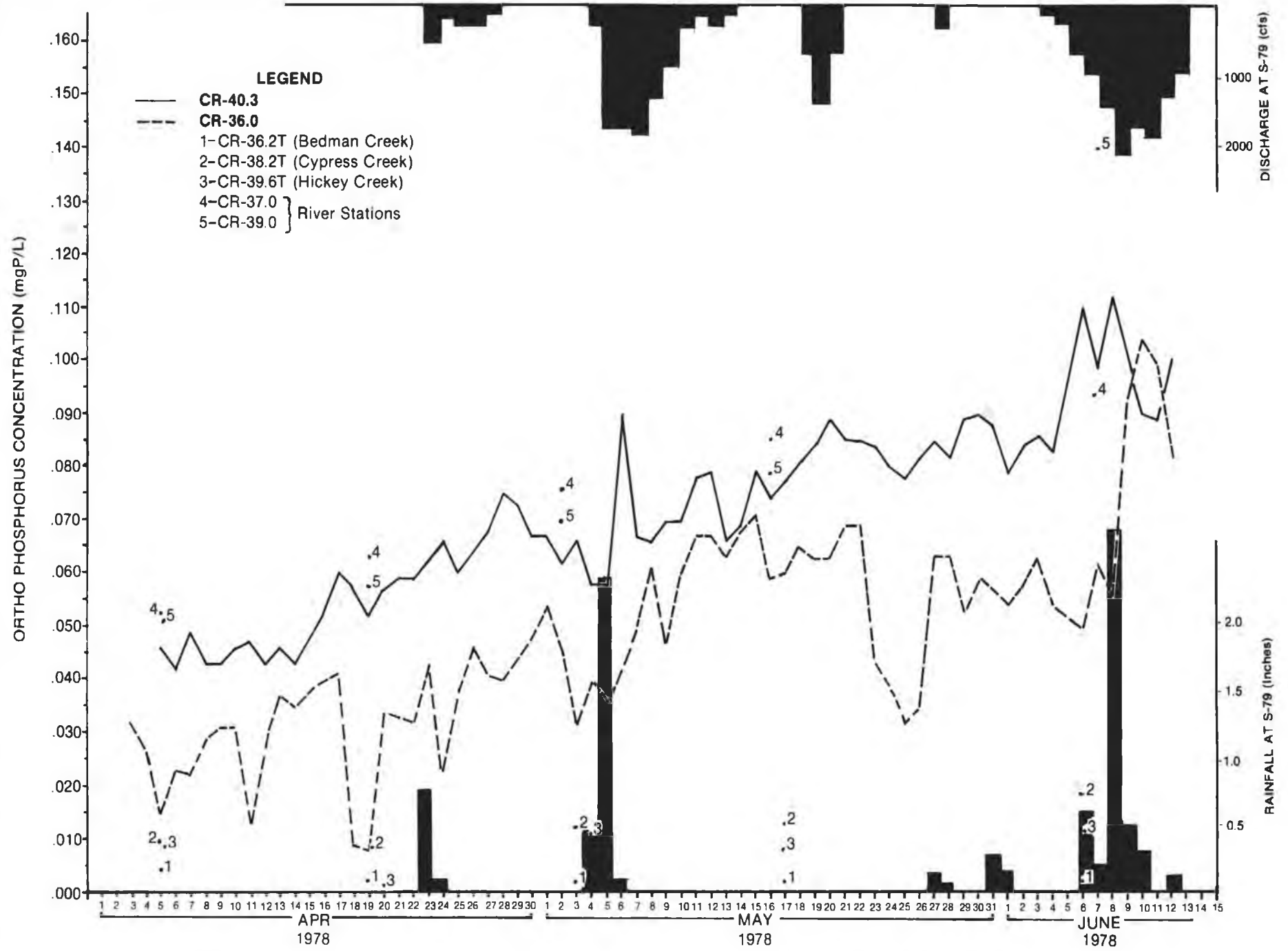
Figure 44 INTENSIVE STUDY ORTHO PHOSPHORUS DATA, 1978
