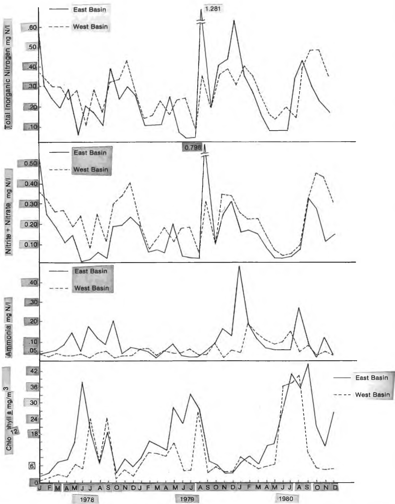
Figure 37B MEAN INORGANIC NITROGEN AND CHLOROPHYLL A CONCENTRATIONS IN THE CALOOSAHATACHEE RIVER DURING ROUTINE SAMPLING TRIPS, 1978 - 1980
