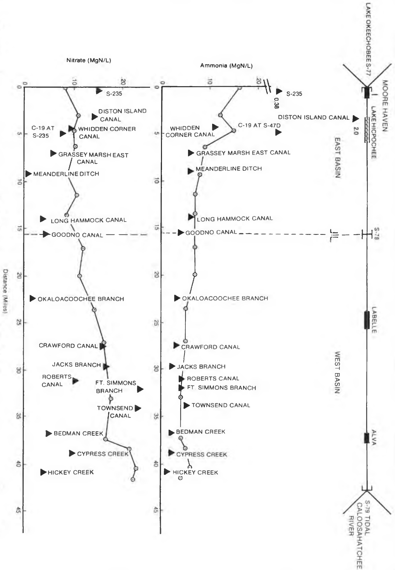
Figure 26 AVERAGE NITRATE AND AMMONIA LEVELS ALONG THE CALOOSAHATCHEE RIVER
