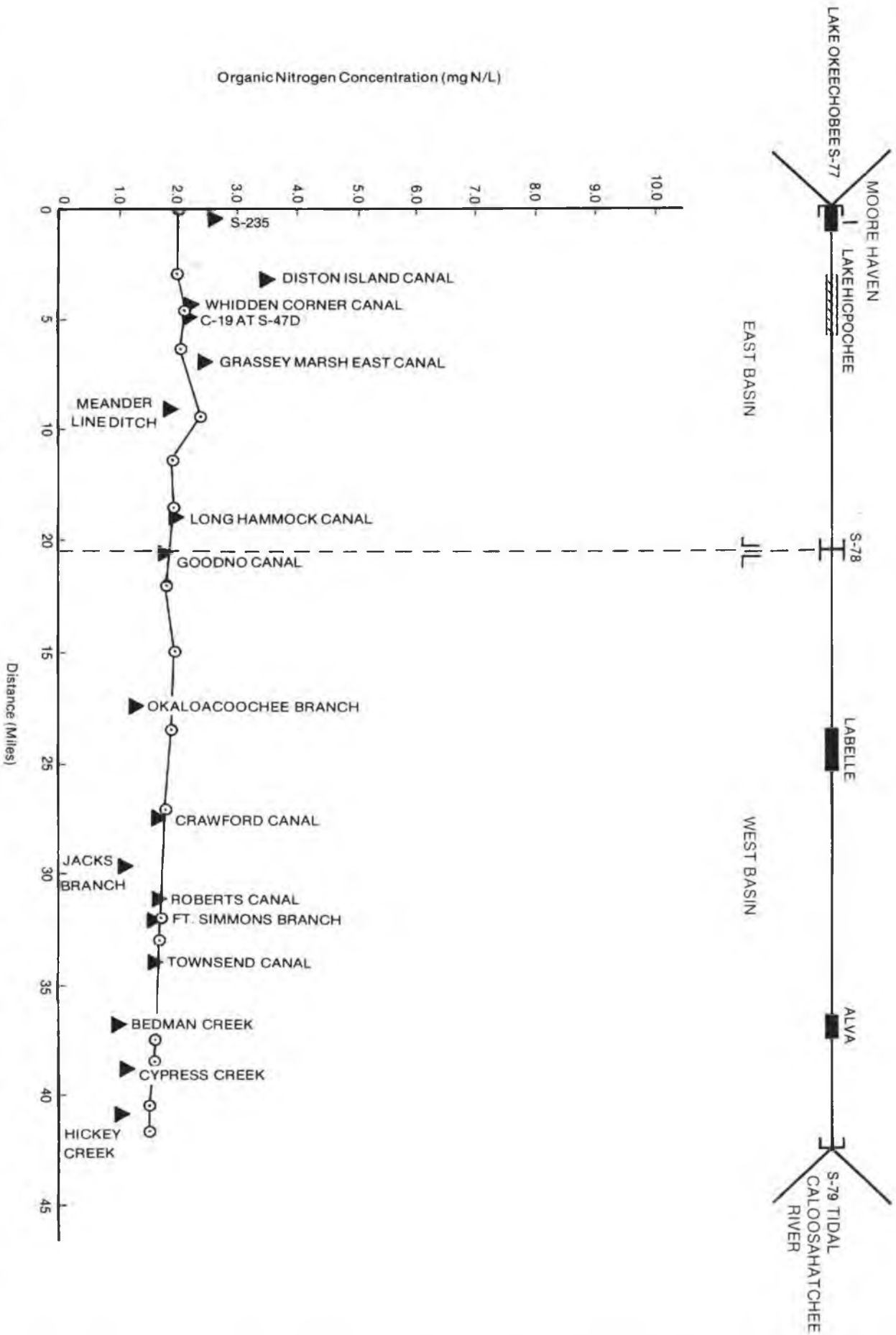
Figure 21 AVERAGE TOTAL ORGANIC NITROGEN ALONG THE CALOOSAHATCHEE RIVER
