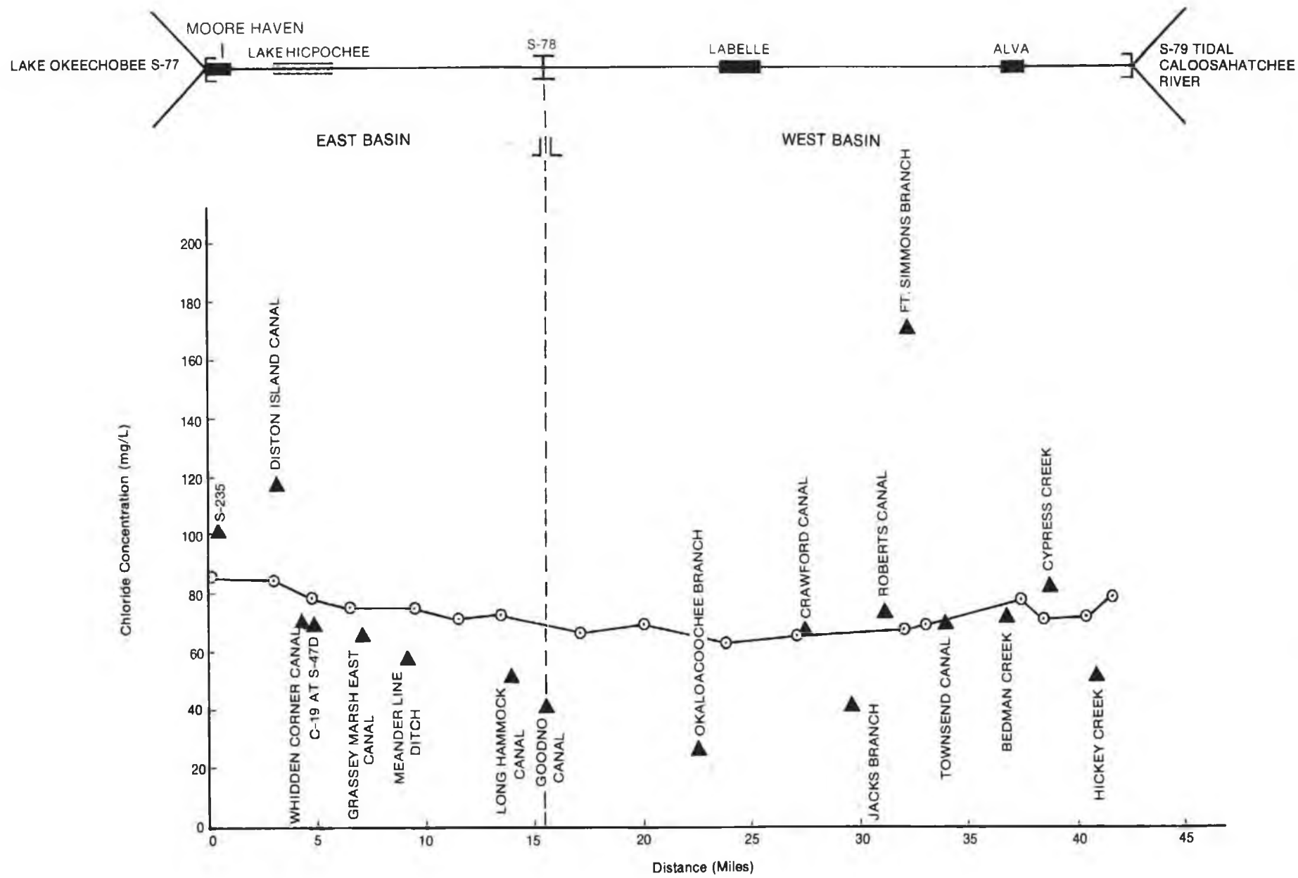
AVERAGE CHLORIDE ALONG THE CALOOSAHATCHEE RIVER
