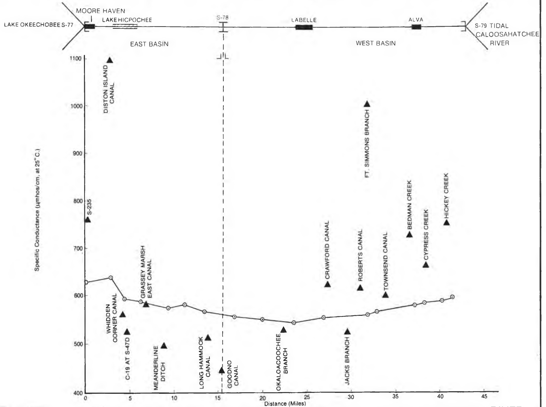
Figure 13 AVERAGE SPECIFIC CONDUCTANCE ALONG THE CALOOSAHATCHEE RIVER
