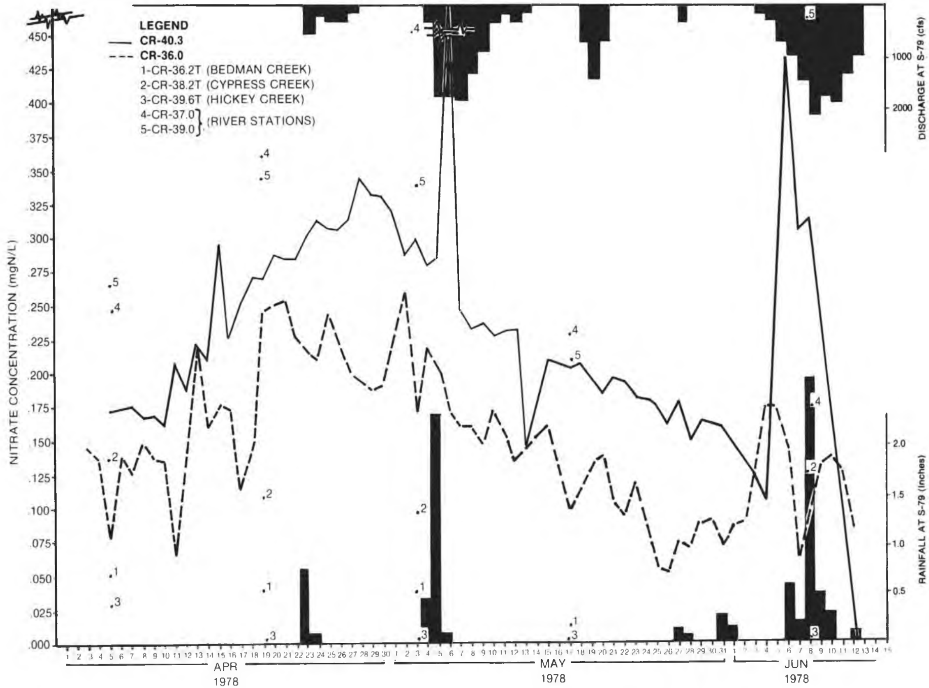
Figure 45 INTENSIVE STUDY NITRATE DATA, 1978
