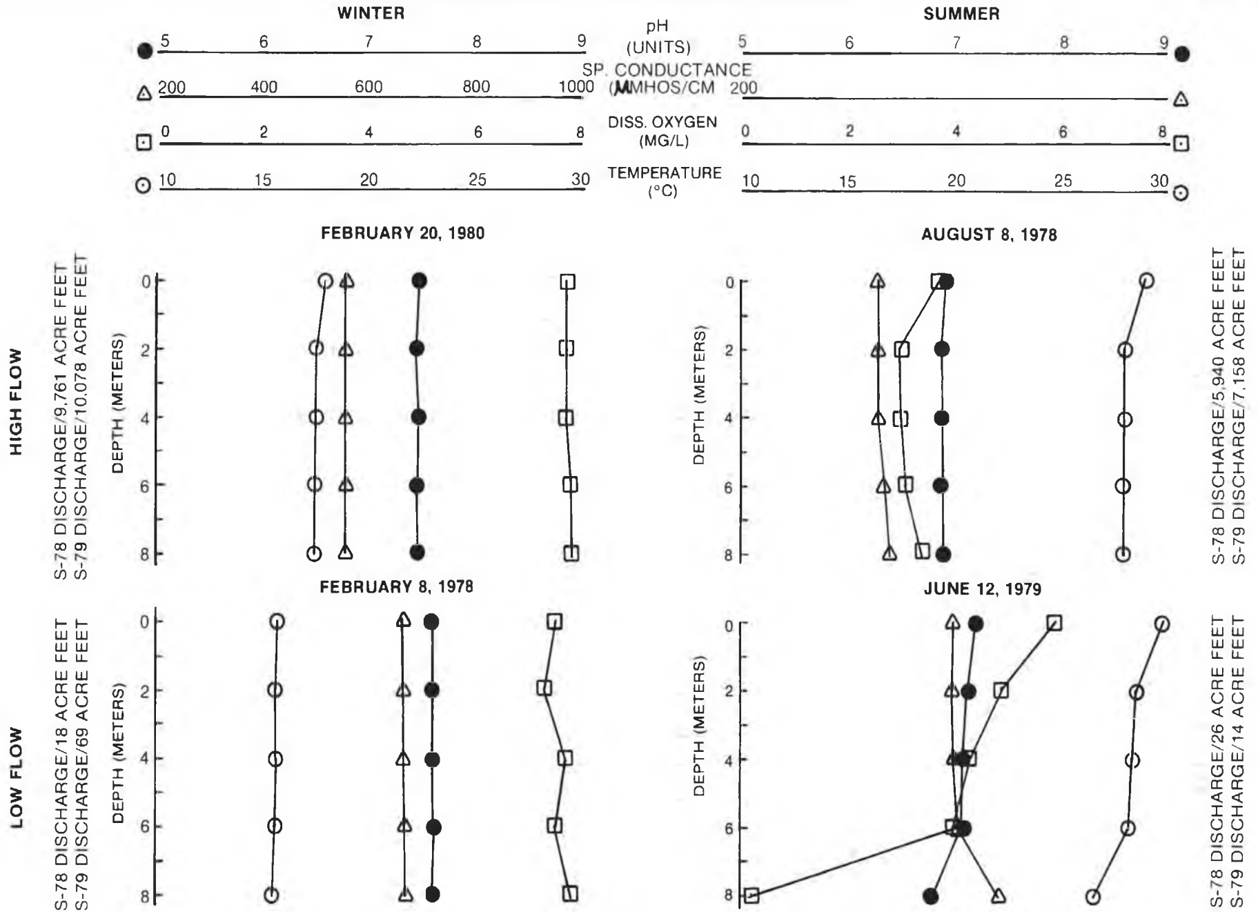
SEASONAL DEPTH PROFILES AT STATION CR-30.4 DURING A HIGH AND LOW FLOW PERIOD
