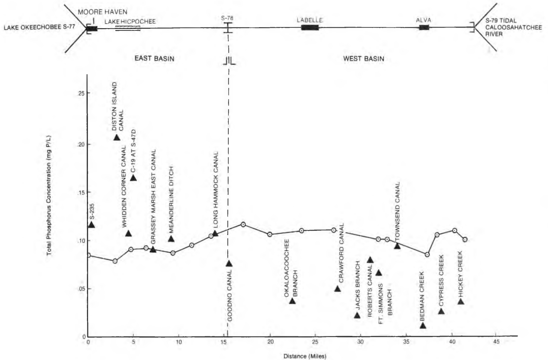
Figure 15 AVERAGE TOTAL PHOSPHORUS ALONG THE CALOOSAHATCHEE RIVER
