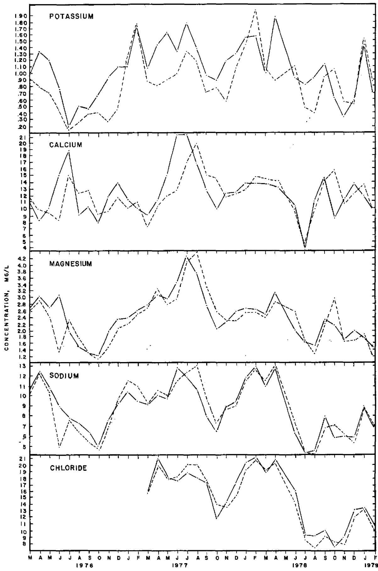
FIG. 6 Monthly average cation and chloride concentrations in inflow (solid line) and outflow (dashed line) water of the flow-thru marsh.
