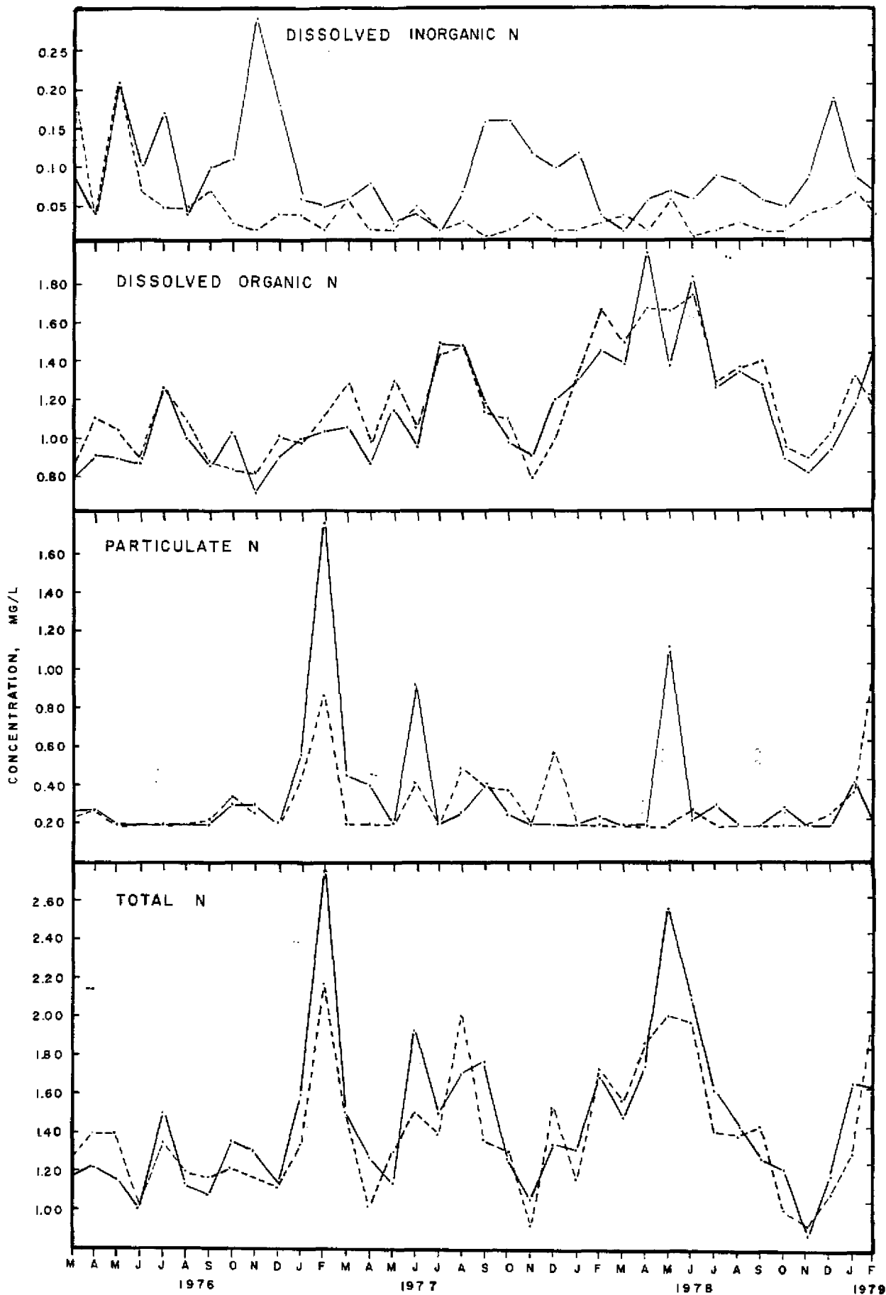
FIG. 4 Monthly average nitrogen concentrations in inflow (solid line) and outflow (dashed line) water of flow-thru marsh.
