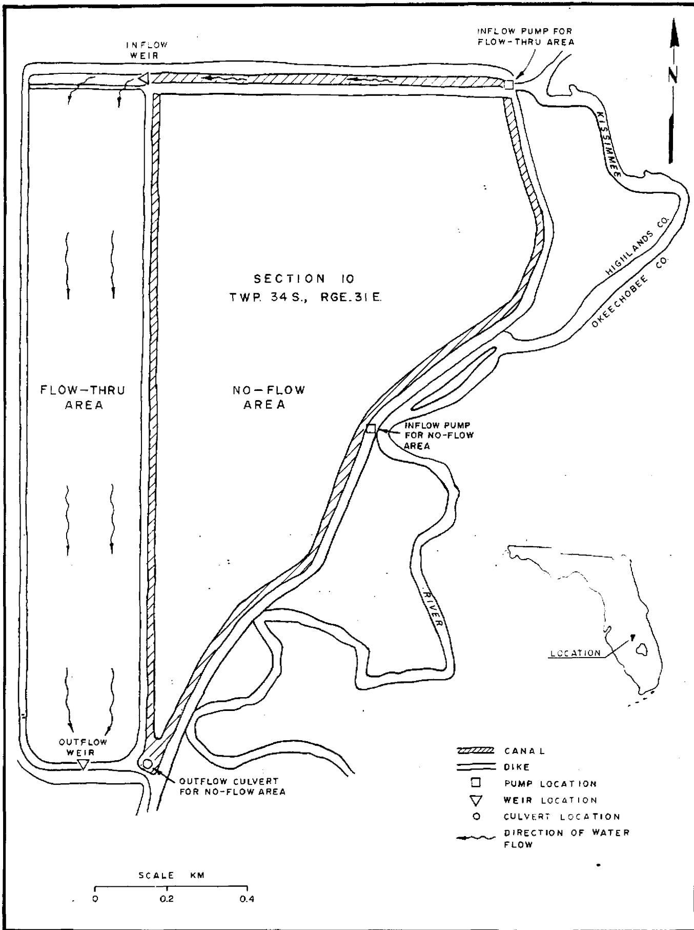
FIG. 1 Boney Marsh Experimental Area
