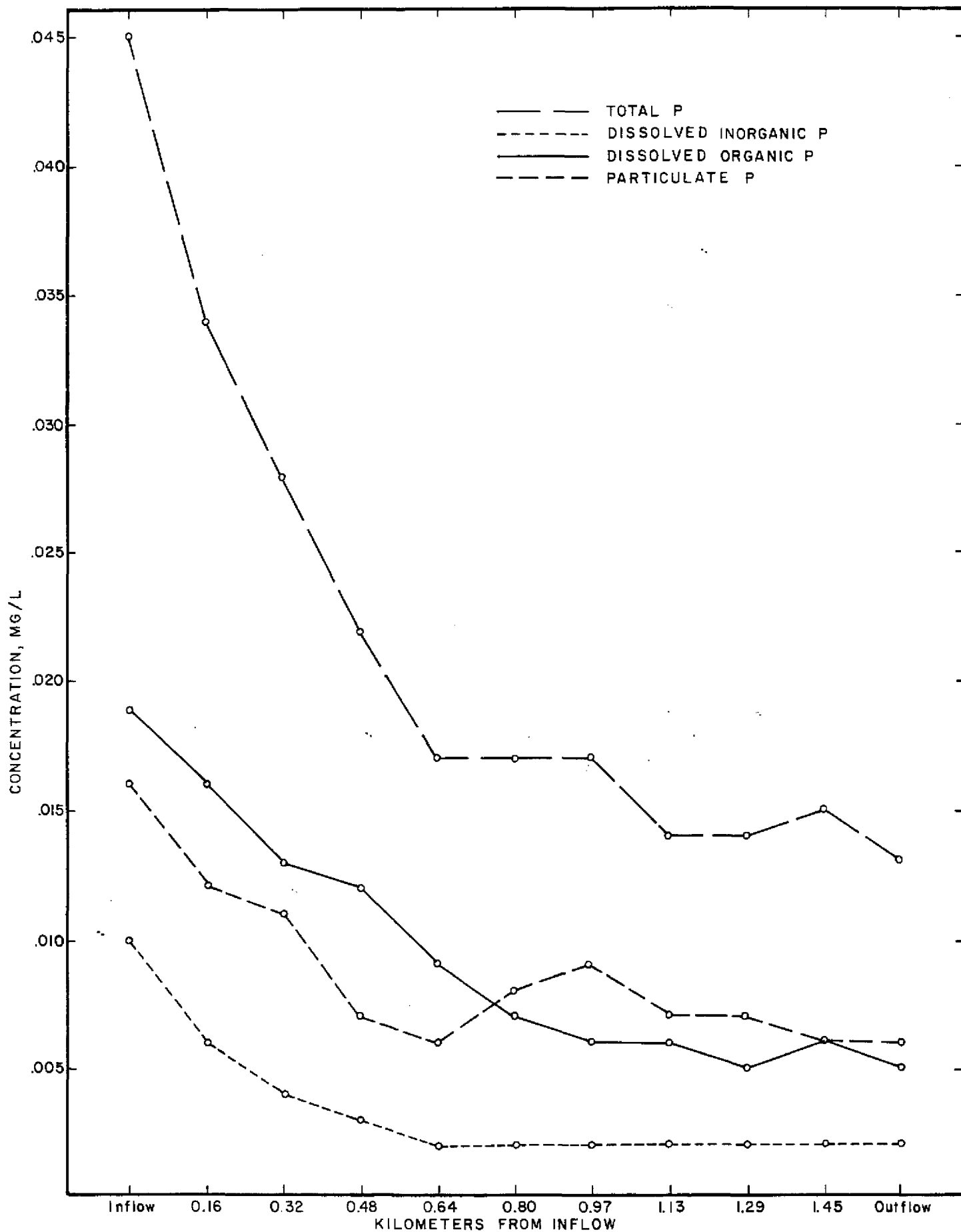
FIG. 3. Reductions in phosphorus concentrations in the water along the length of the flow-thru marsh.
