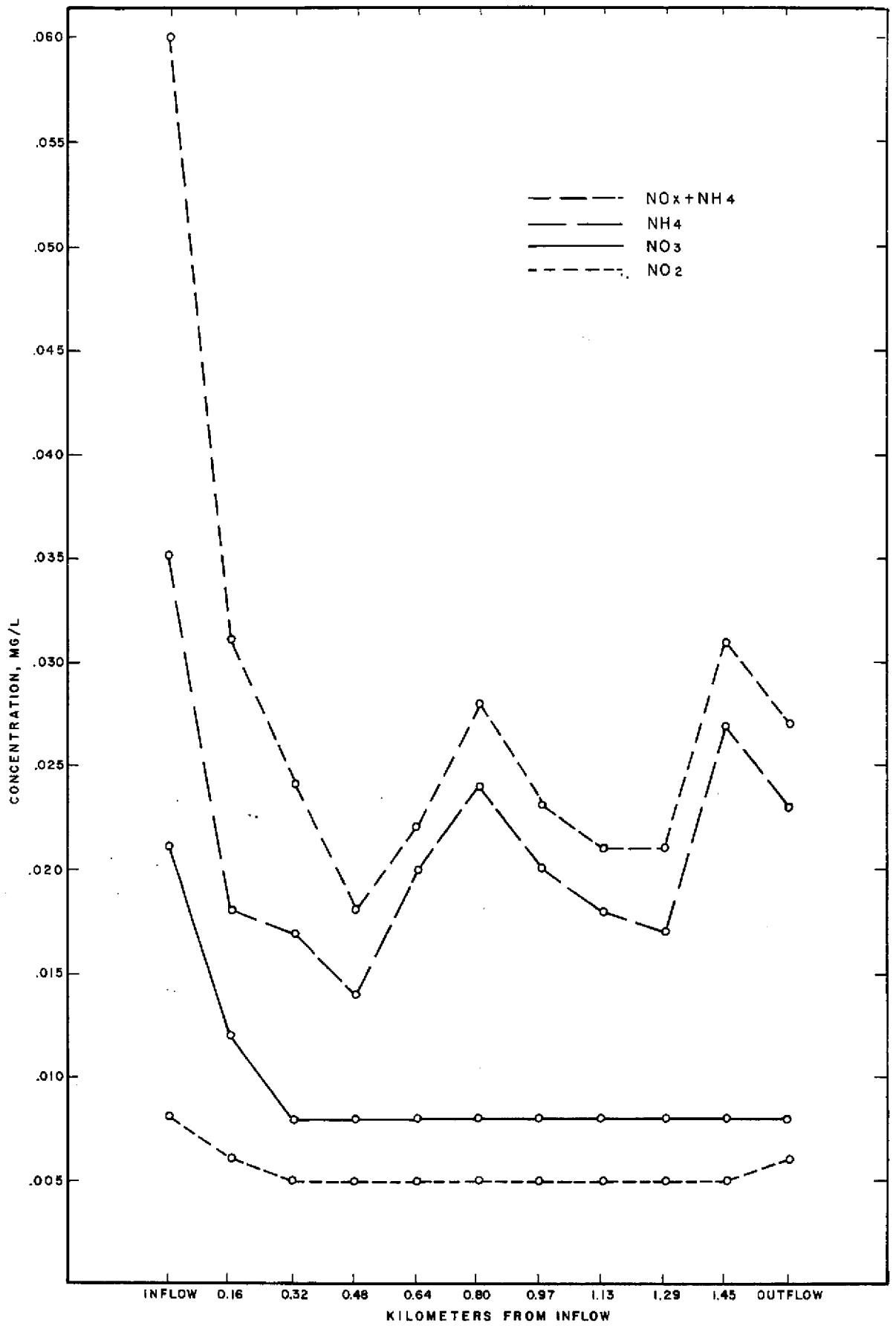
FIG. 5 Reductions in inorganic nitrogen concentrations in the water along the length of the flow-thru marsh.
