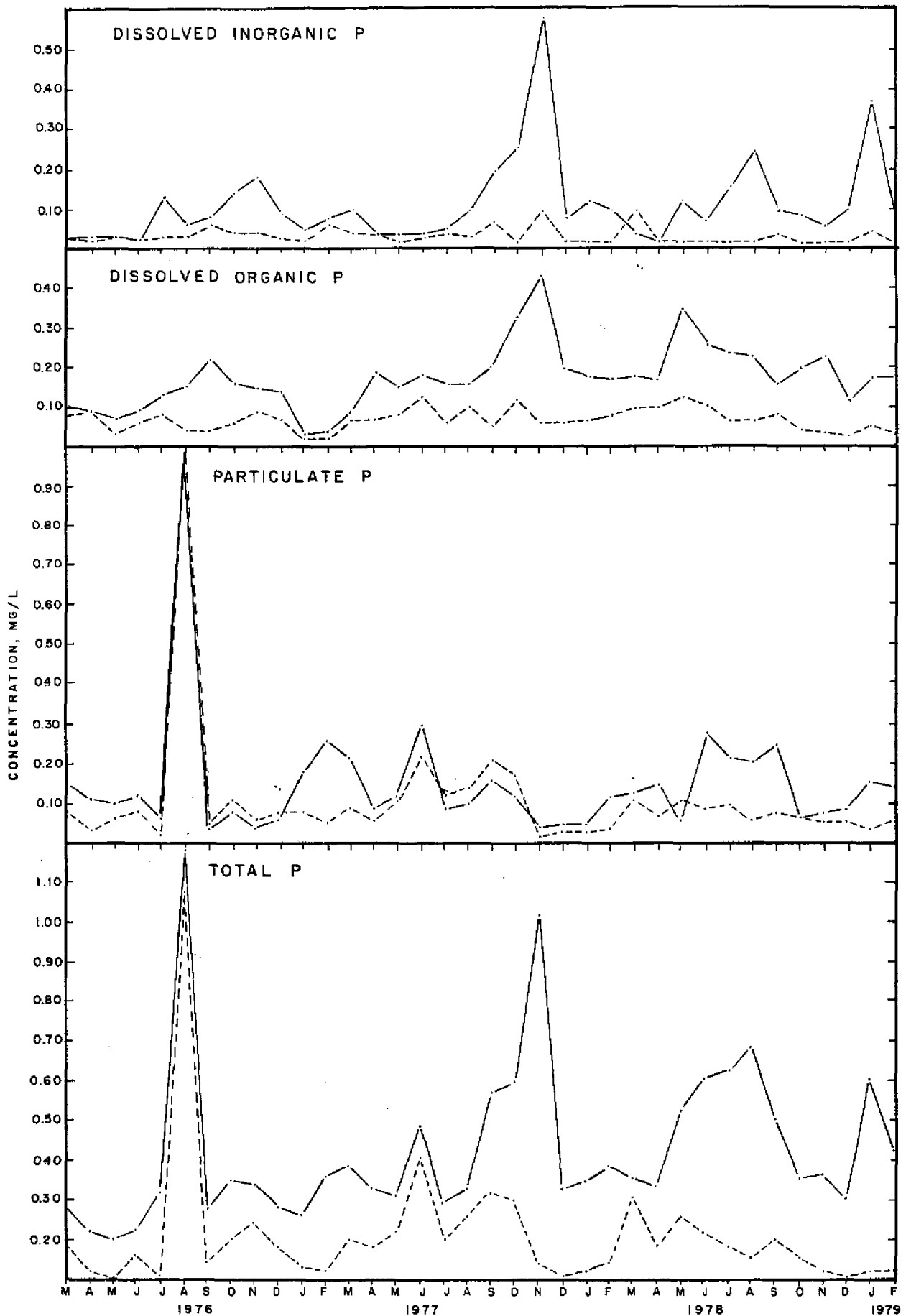
FIG. 2 Monthly average phosphorus concentrations in inflow (solid line) and outflow (dashed line) water of flow-thru marsh.
