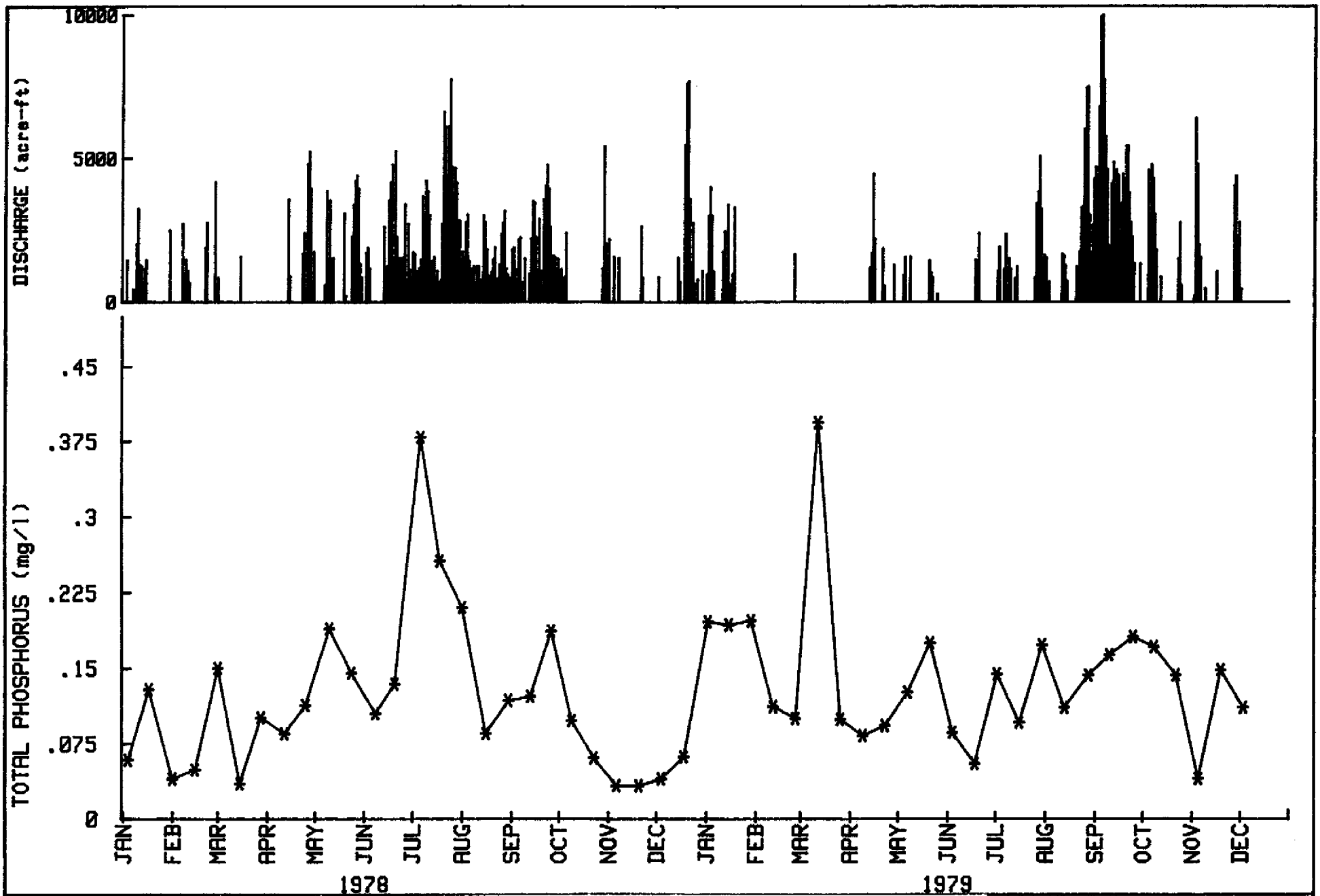
FIGURE 7. TOTAL PHOSPHORUS AND DISCHARGE DATA FOR S5A : 1978-79
