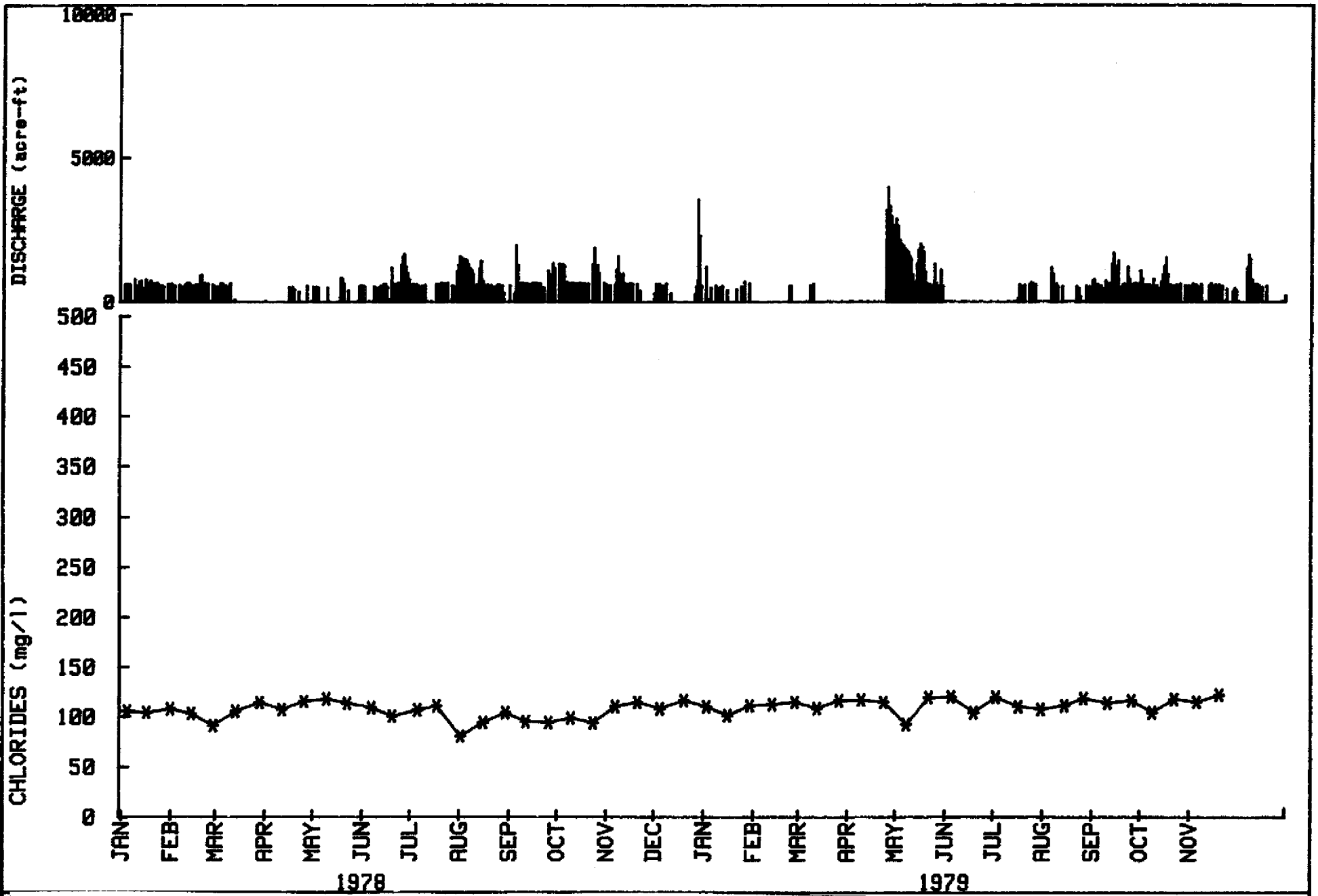
FIGURE 14. CHLORIDE AND DISCHARGE DATA FOR S9 : 1978-79
