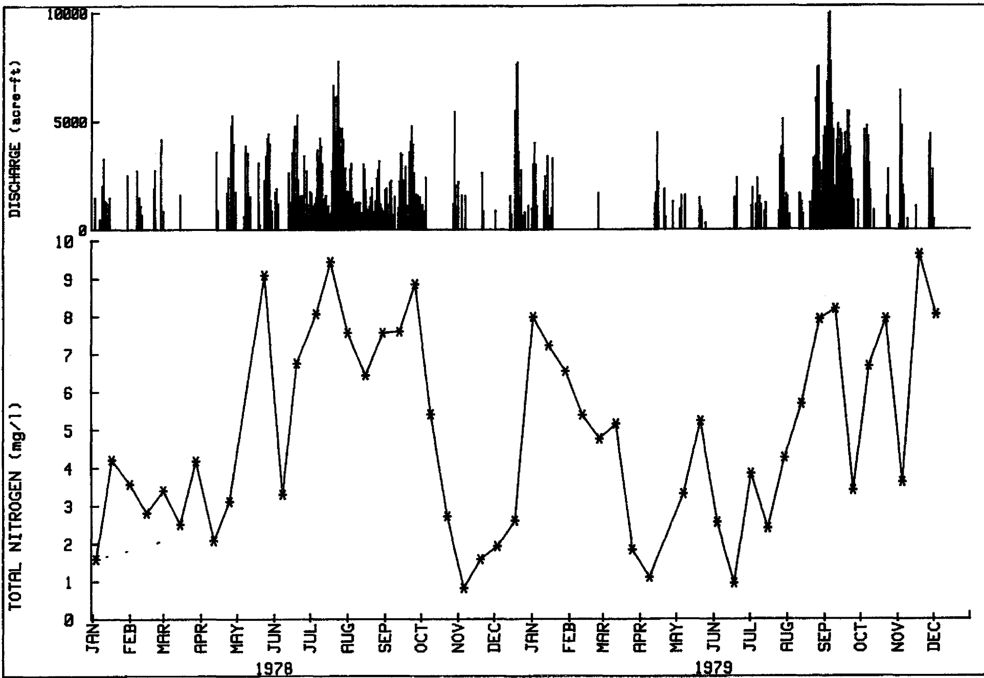
FIGURE 6. TOTAL NITROGEN AND DISCHARGE DATA FOR S5A : 1978-79
