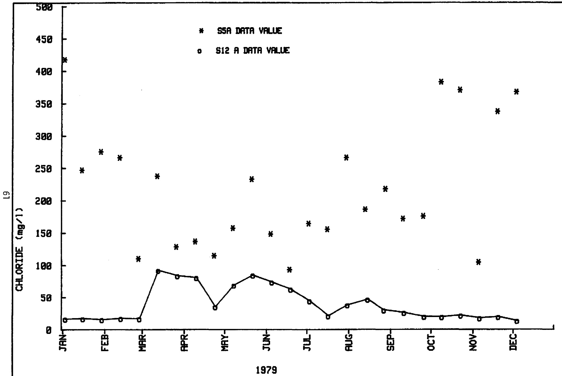
FIGURE 29. COMPARISON OF S5A AND S12A CHLORIDE DATA FOR 1979
