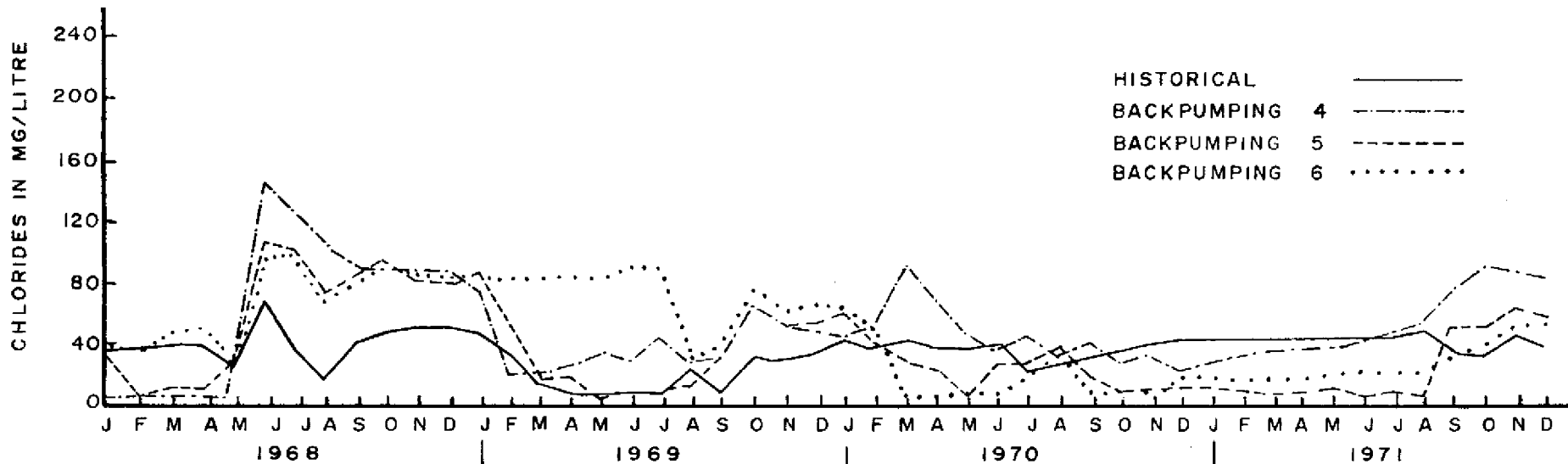
Figure 12. POLLUTOGRAPH OF CHLORIDES FOR NODE 15 OF CONSERVATION AREA I
