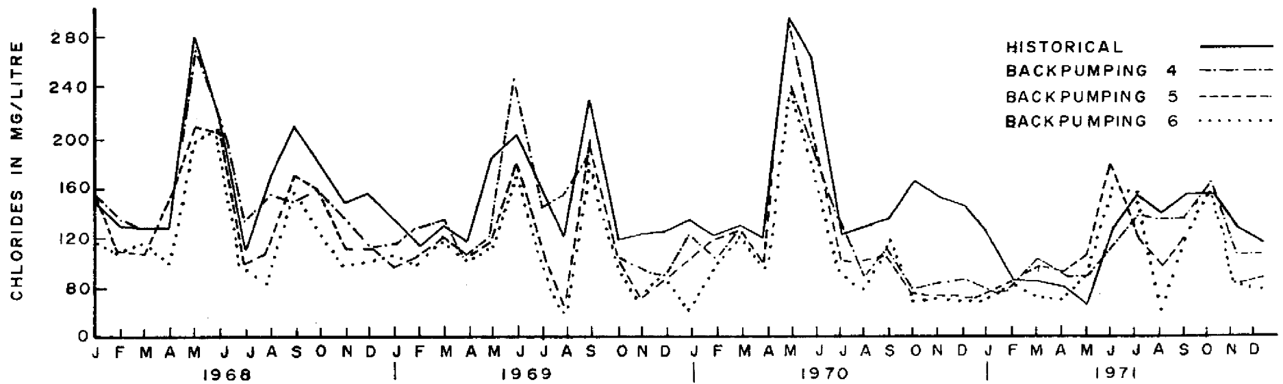
Figure 13. POLLUTOGRAPH OF CHLORIDES FOR NODE 17 OF CONSERVATION AREA I
