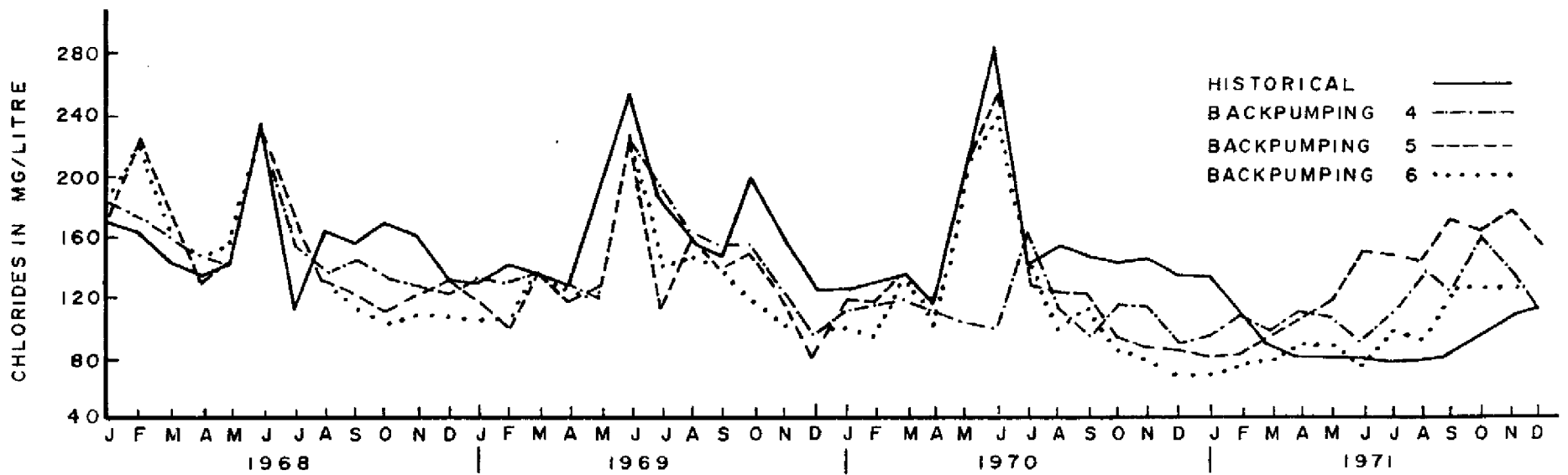
Figure 9. POLLUTOGRAPH OF CHLORIDES FOR NODE I OF CONSERVATION AREA I
