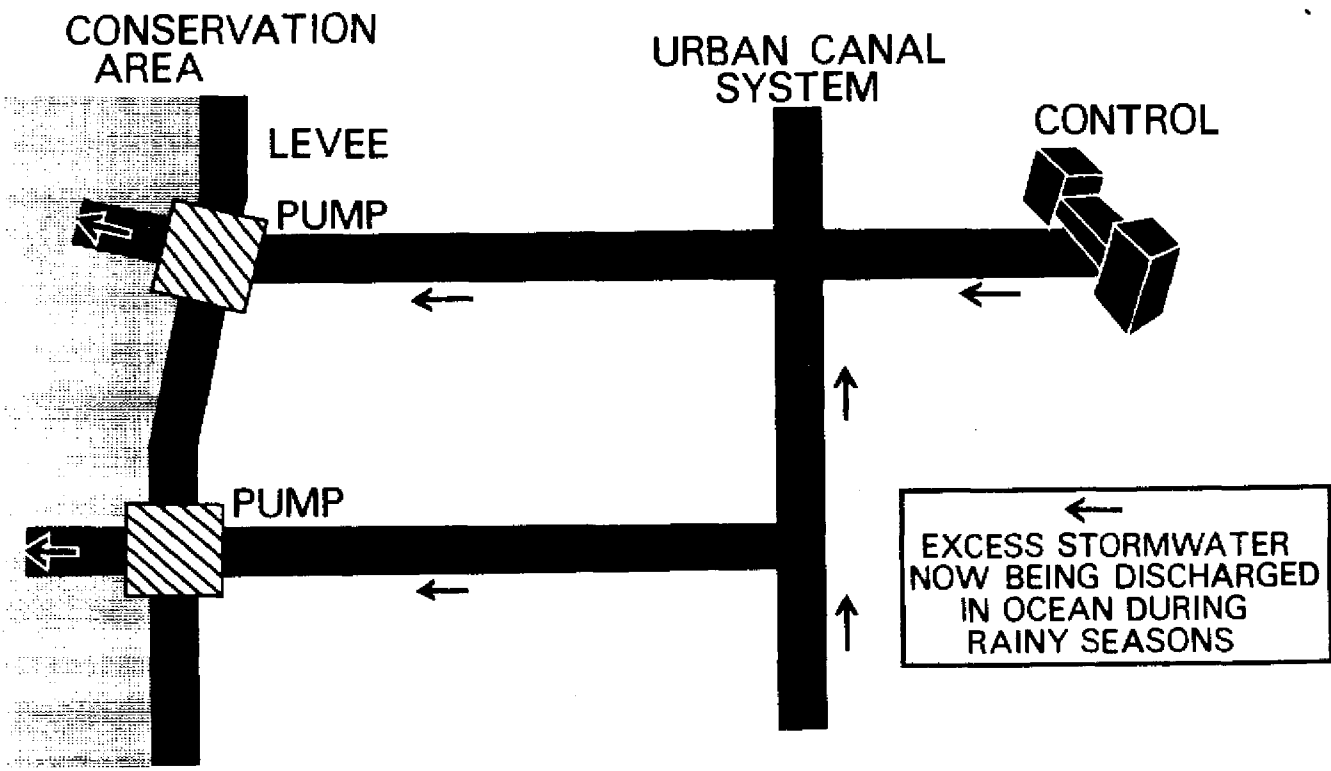
Figure 2. Comparison of Normal and Backpumping Flow Directions.
