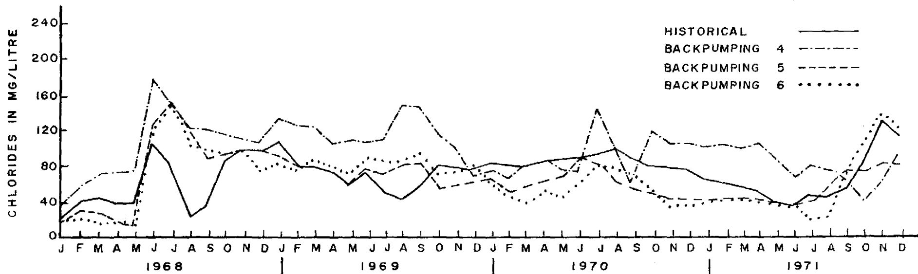
Figure 11. POLLUTOGRAPH OF CHLORIDES FOR NODE 5 OF CONSERVATION AREA I
