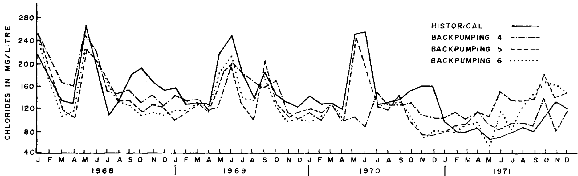
Figure 10. POLLUTOGRAPH OF CHLORIDES FOR NODE 4 OF CONSERVATION AREA I
