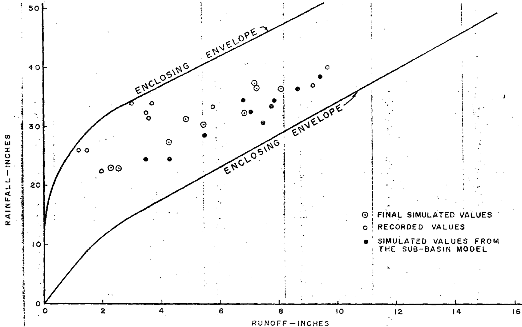
COMPARISON OF RAINFALL-RUNOFF RELATIONSHIPS OBTAINED FROM THE SUB-BASIN MODEL WITH THE HISTORICAL DATA FOR THE ENTIRE KISSIMMEE BASIN FOR THE WET SEASONS DURING 1960-70
