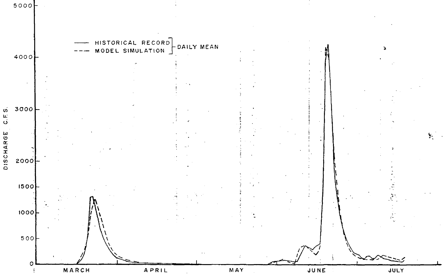
Figure 7 COMPARISON OF SIMULATED AND RECORDED DISCHARGE FOR TAYLOR CREEK (8,9)
