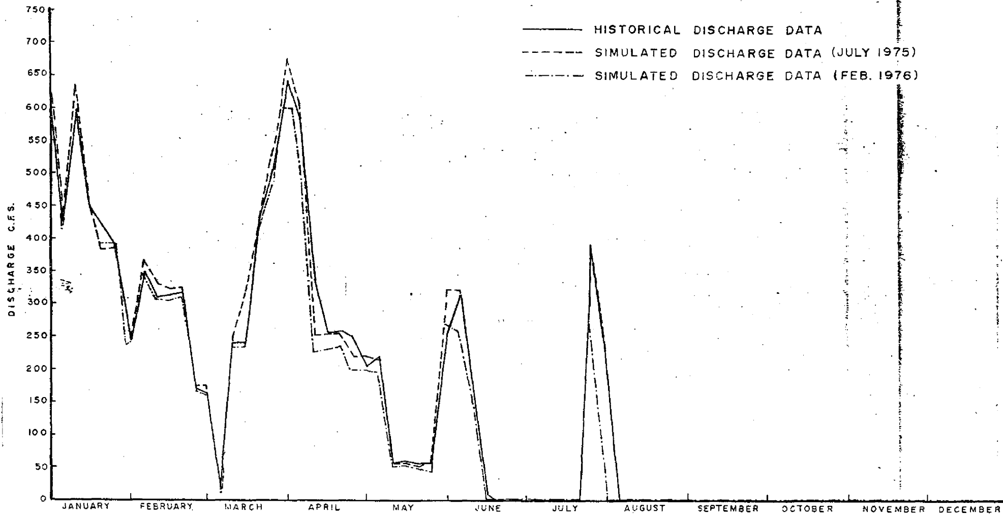
COMPARISON OF SIMULATED AND RECORDED DISCHARGES THROUGH S-59 FOR THE FULL YEAR OF 1970
