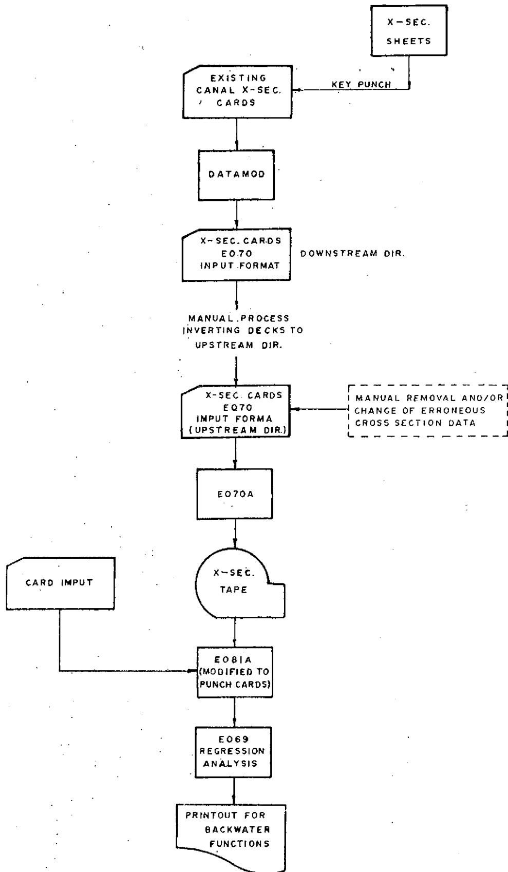
Figure 36. A FLOW CHART OF THE PROCEDURE FOR ARRIVING AT BACKWATER FUNCTIONS
