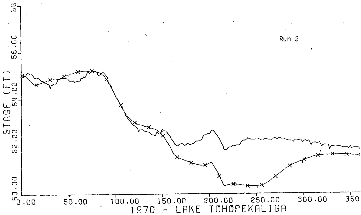
Figure 51. Effects of Parametric Sensitivity Analyses on the Refinement of Simulated Lake Stages for Lake Tohopekaliga
