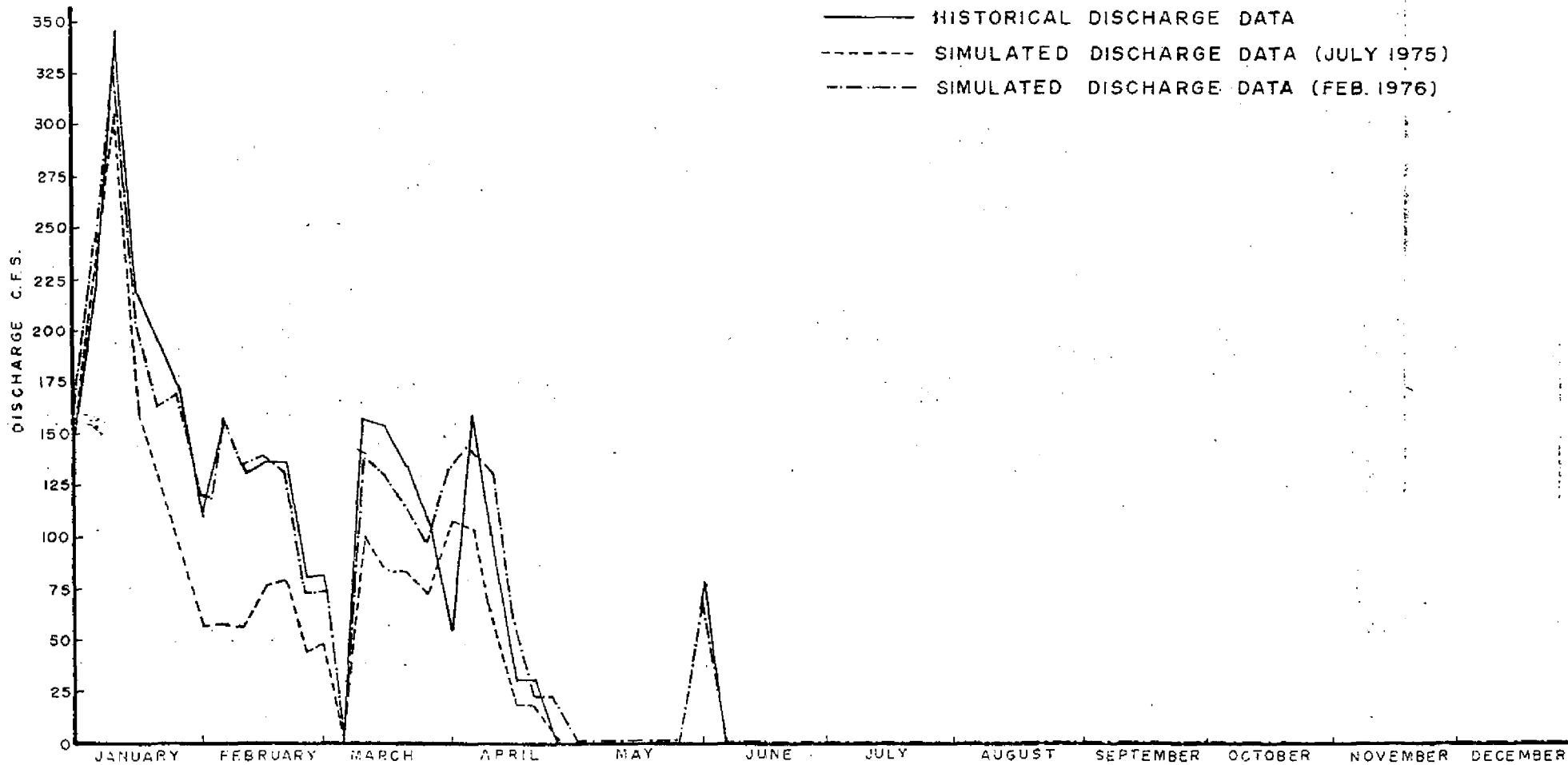
COMPARISON OF SIMULATED AND RECORDED DISCHARGES THROUGH S-62 FOR THE FULL YEAR OF 1970
