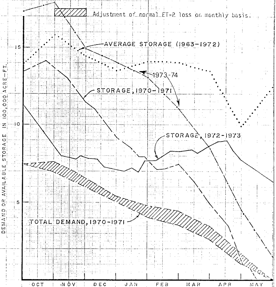
STORAGE AND DEMAND CURVES FOR LAKE OKEECHOBEE
