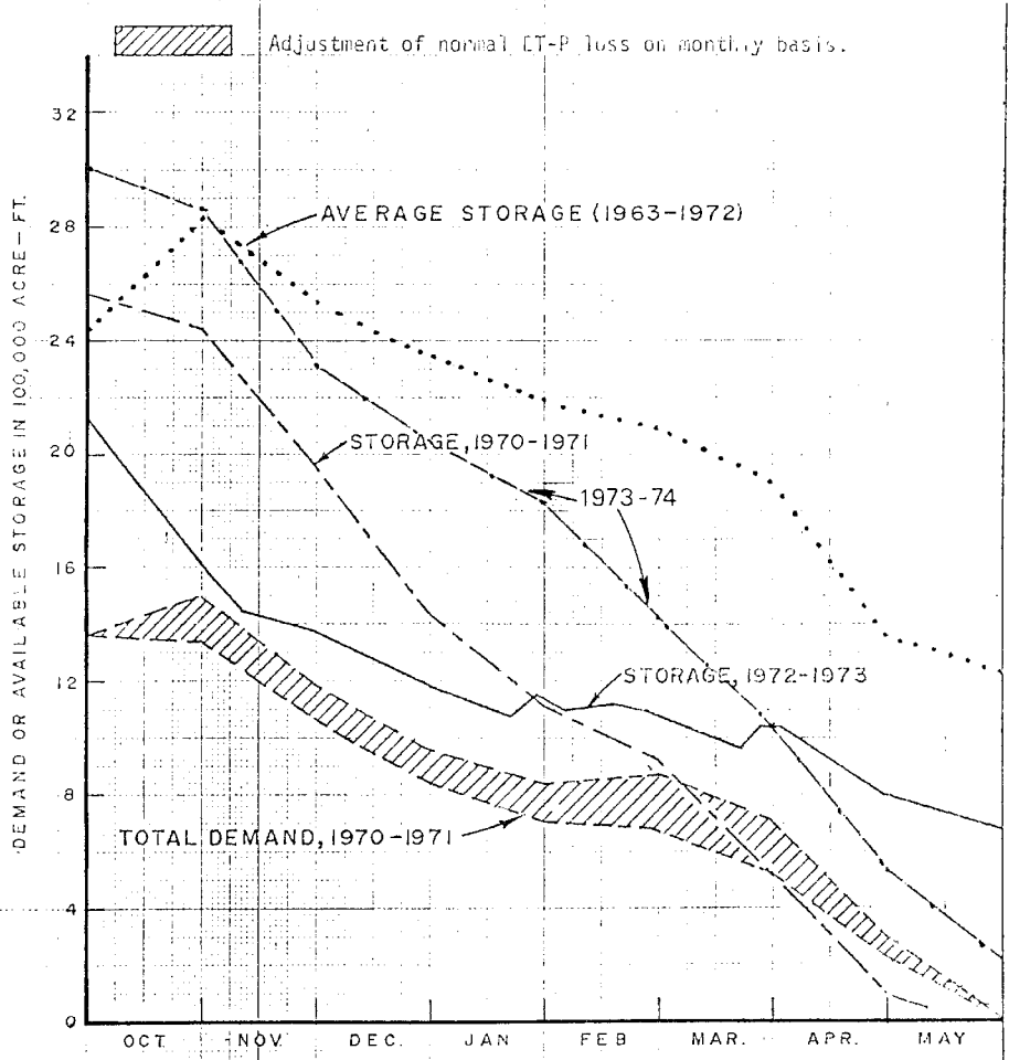
THE DISTRICT TOTAL STORAGE AND DEMAND CURVES
