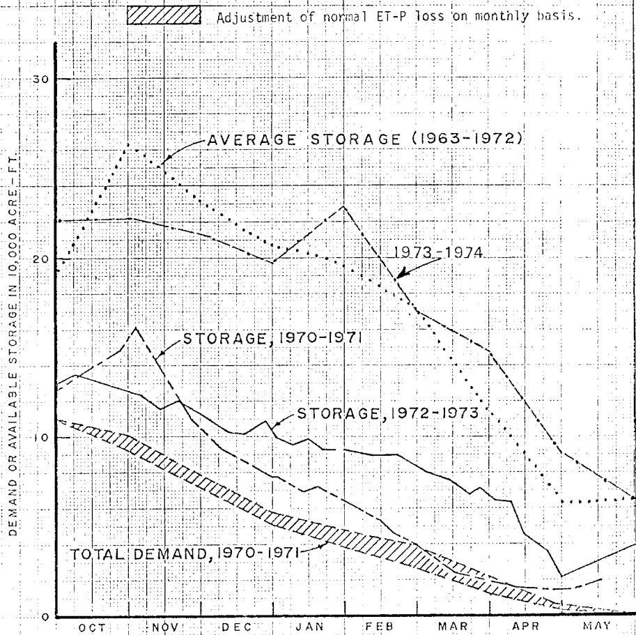
STORAGE AND DEMAND CURVES FOR CONSERVATION AREA 1
