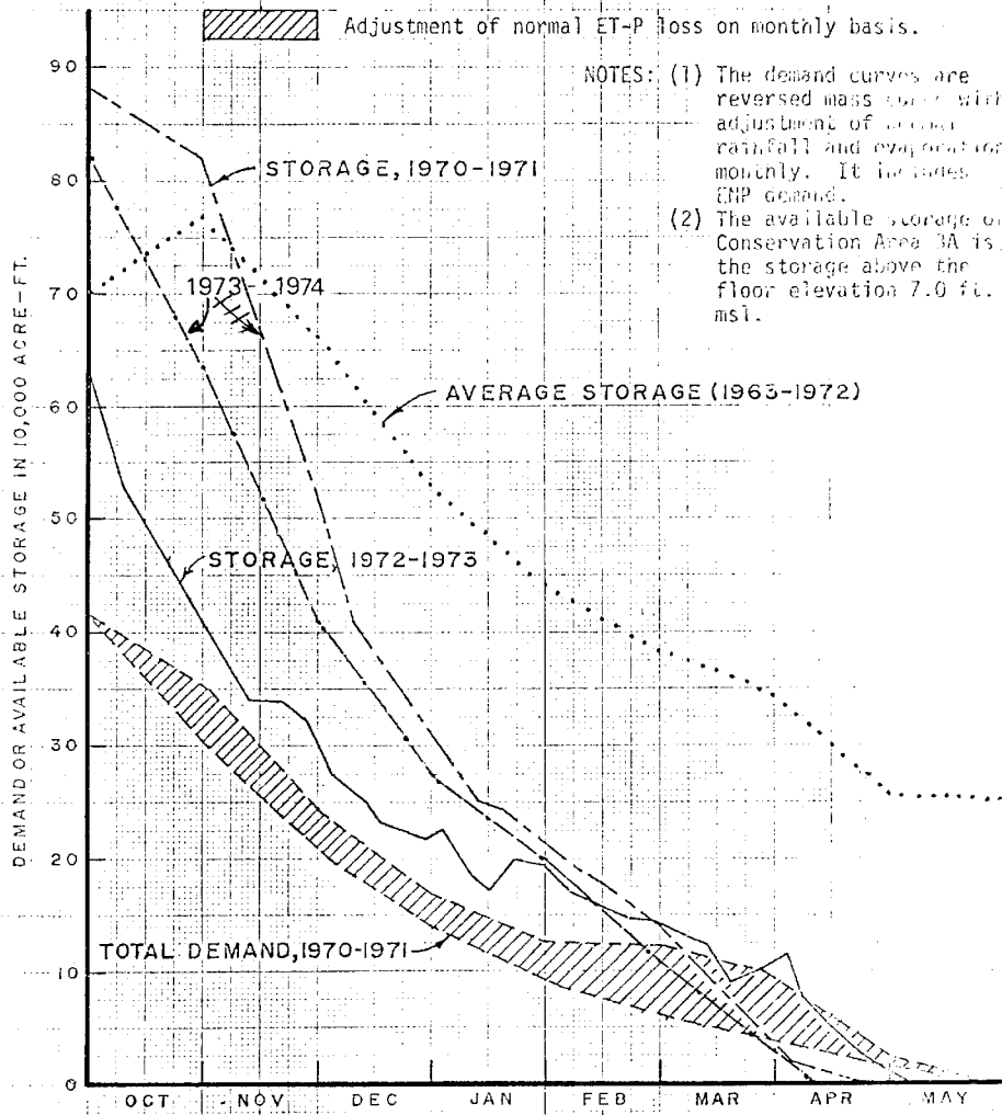
STORAGE AND DEMAND CURVES FOR CONSERVATION AREA 3A
