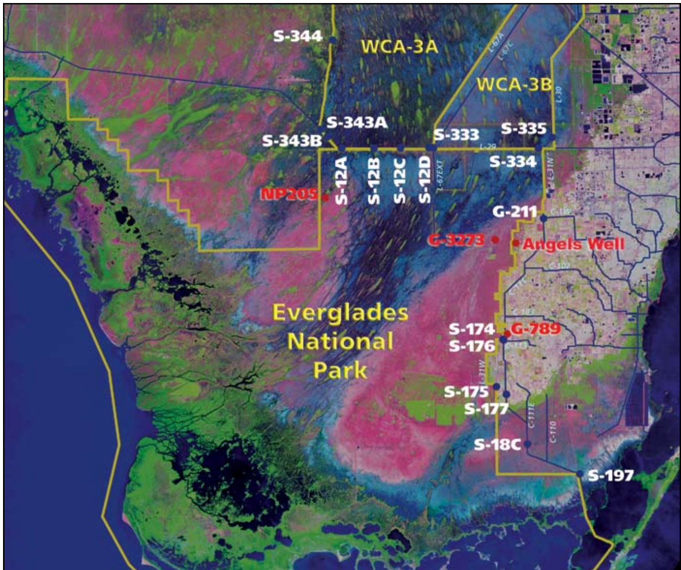
Figure 2. Components of the C&SF Project that affect water deliveries to ENP and some important monitoring sites (red) for controlling deliveries and evaluating potential impacts.
