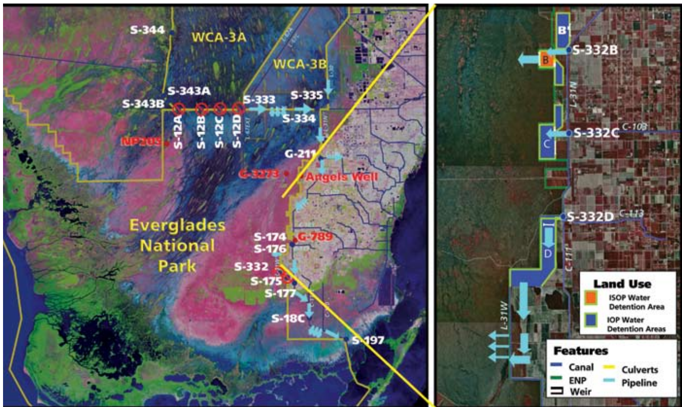
Figure 5. Depiction of the structural and operational components of the ISOP and IOP. The S-332B-C connector detention area has yet to be completed. Problems with the acquisition of the land between the north and south segments prevent complete connection of these two detention areas.
