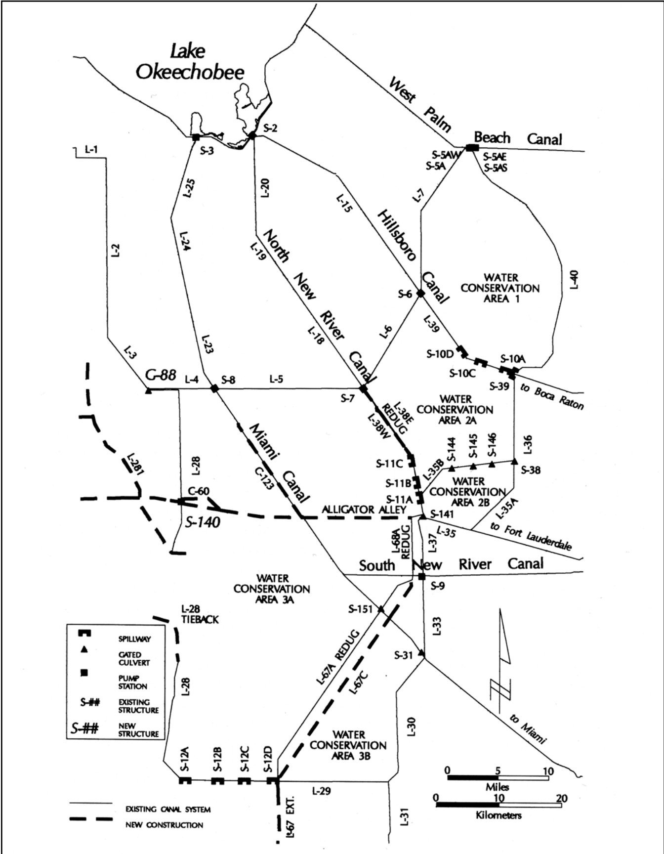
Figure 3. South Dade Conveyance System (reproduced from Davis and Ogden 1994).
