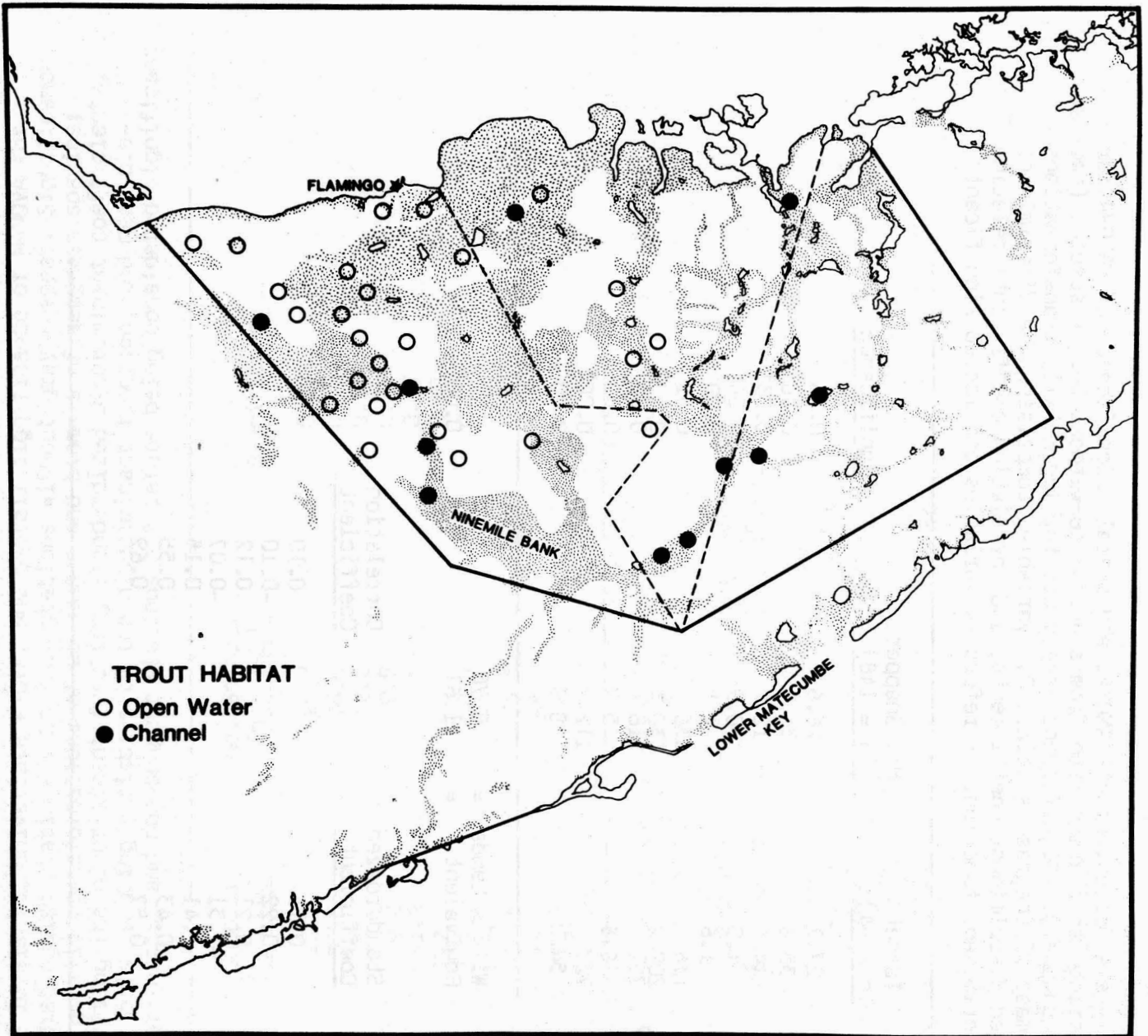
Figure 40. Results of discriminant analysis depicting seatrout habitat.
