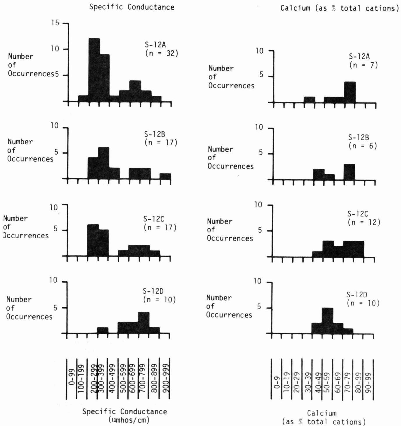
Figure 6. Specific conductance and % calcium frequency histograms for S-12 water delivery sampling sites.
