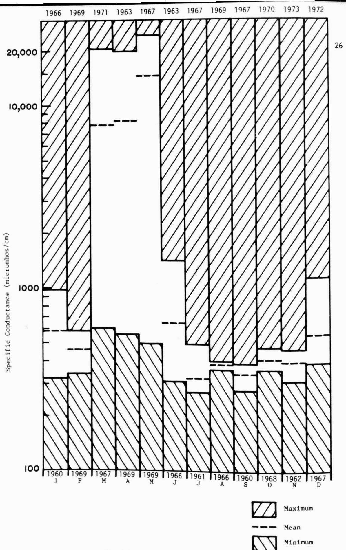
Figure 10: Monthly specific conductance ( \mu mhos/cm) at Shark Slough station P-35 (1960-1979)
