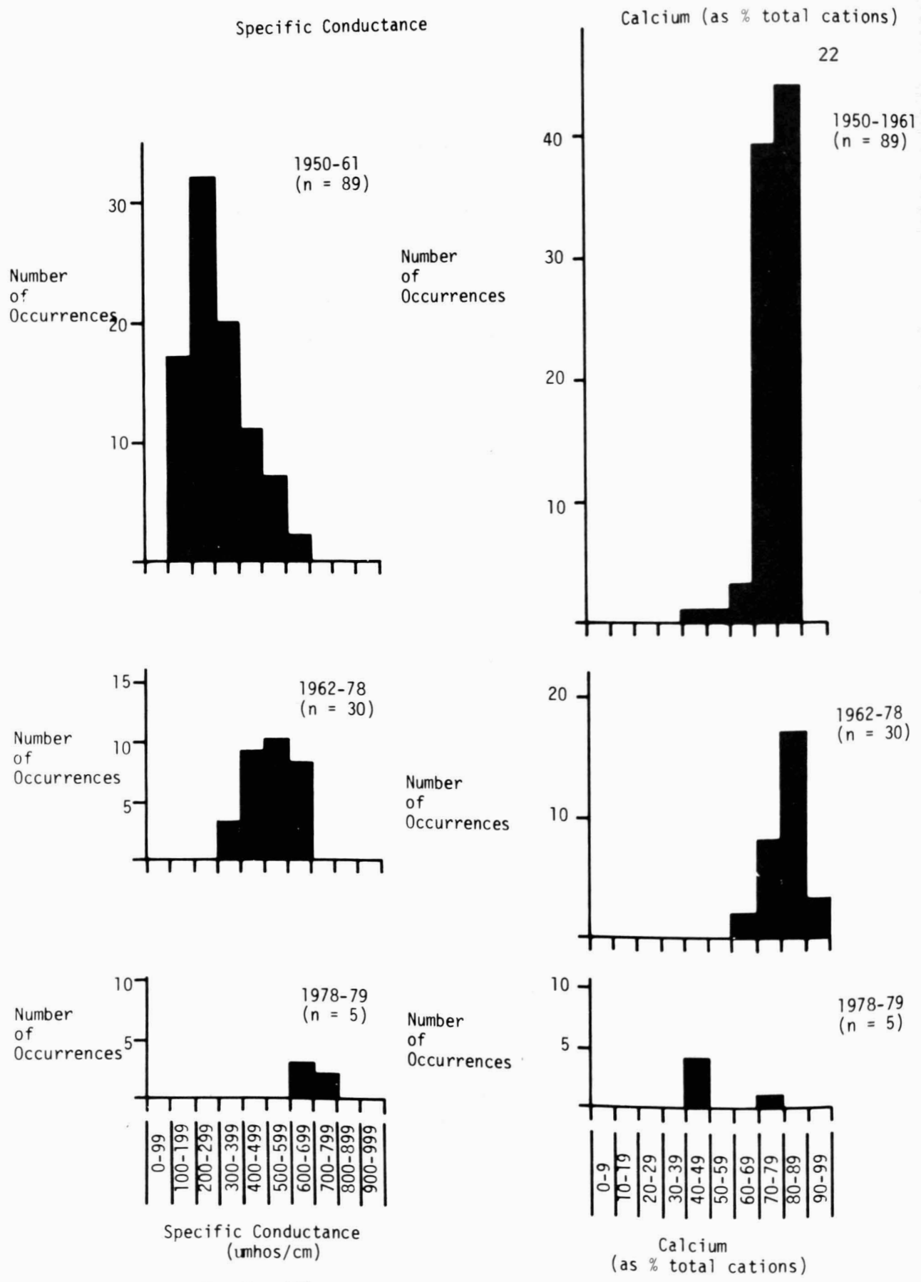
Figure 8. Specific conductance and % calcium frequency histograms for Bridge 53 (1950-61, 1962-78, 1978-79).
