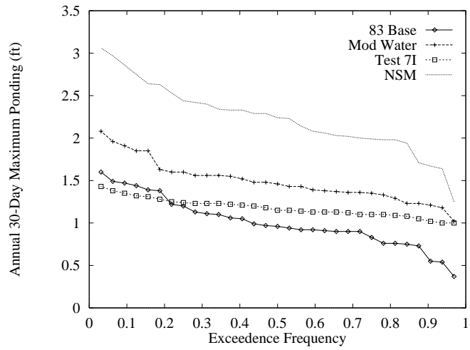
Figure 110: Annual maximum depth exceedence frequency for 30 continuous days for Northeast Shark Slough (Indicator Region 11).
