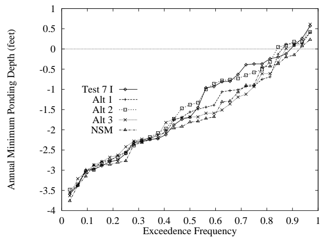
Figure 181: Annual stage exceedance frequency for the minimum for East Slough (Indicator Region 13).
