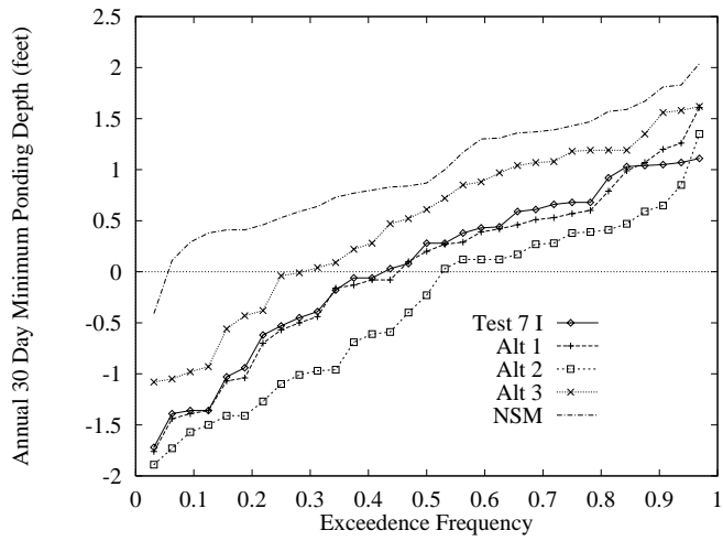
Figure 174: Annual stage exceedence frequency for the 30 Day continuous minimum for North East Shark Slough (Indicator Region 11).
