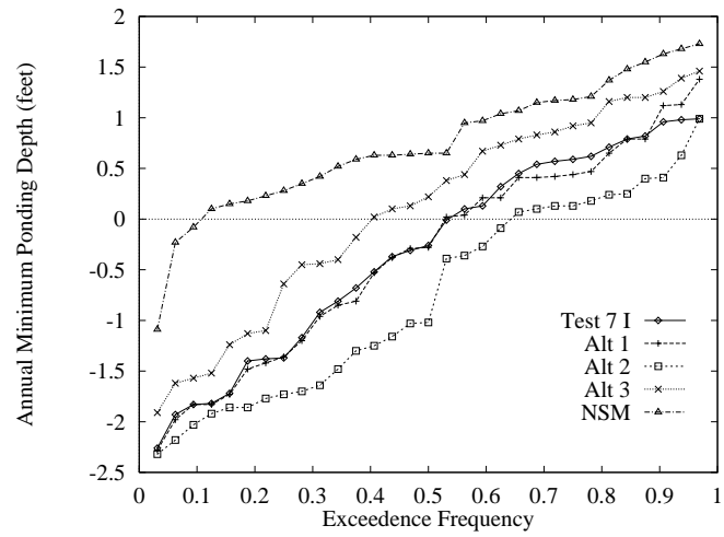
Figure 180: Annual stage exceedance frequency for the minimum for North East Shark Slough (Indicator Region 11).
