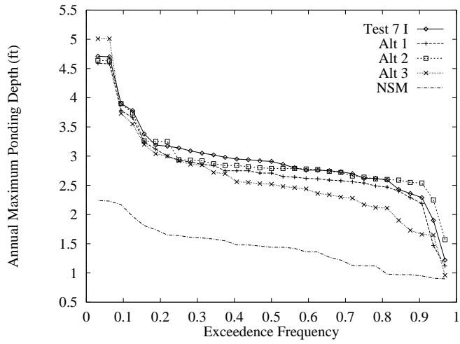
Figure 194: Annual maximum stage exceedence frequency for Southern WCA-3A Snail Kite Habitat.
