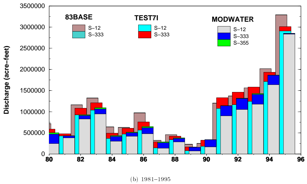
Figure 93: Comparison of Tamiami Trail annual flow volumes.
