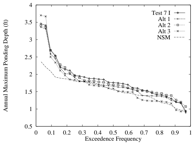
Figure 195: Annual maximum stage exceedence frequency for Western WCA-3A Snail Kite Habitat.
