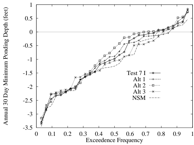
Figure 175: Annual stage exceedence frequency for the 30 Day continuous minimum for East Slough (Indicator Region 13).
