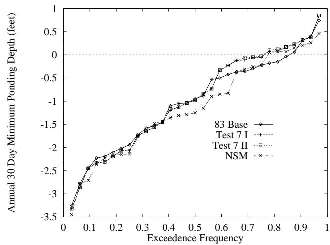
Figure 152: Annual stage exceedence frequency for the 30 Day continuous minimum for East Slough (Indicator Region 13).
