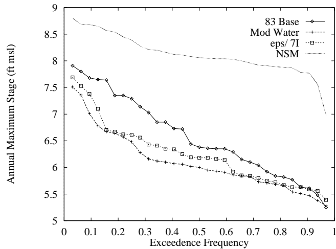
Figure 106: Annual maximum stage exceedence frequency for the 8.5 SMA.
