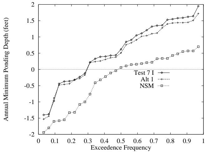
Figure 186: Annual stage exceedence frequency for the minimum for Southern WCA-3A Snail Kite Habitat.
