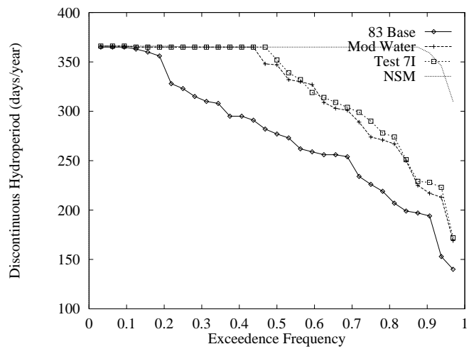
Figure 111: Hydroperiod exceedence frequency for Northeast Shark Slough (Indicator Region 11).
