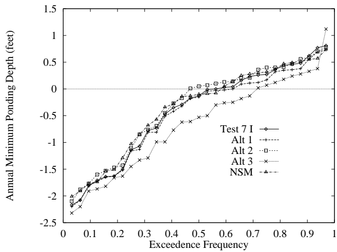
Figure 187: Annual stage exceedence frequency for the minimum for Western WCA-3A Snail Kite Habitat.
