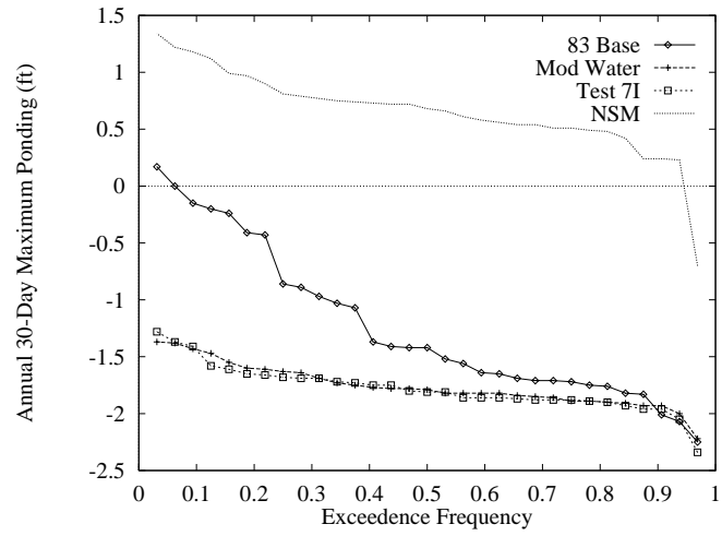
Figure 107: Annual maximum depth exceedence frequency for 30 continuous days for the 8.5 SMA.
