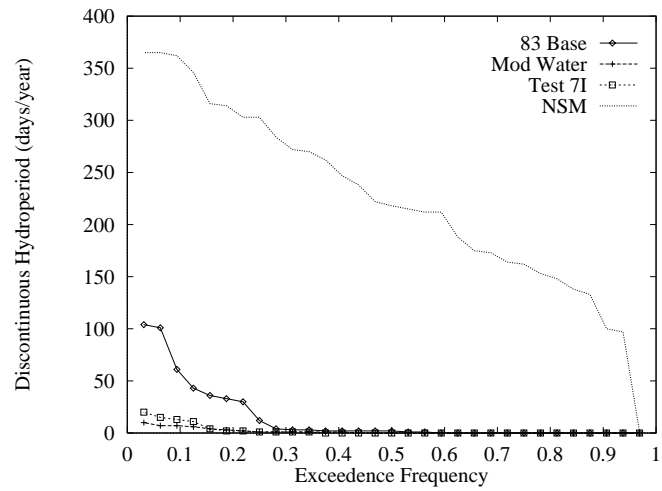
Figure 108: Hydroperiod exceedence frequency for the 8.5 SMA.
