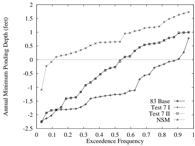
Figure 20: Annual Minimum Ponding Depth for Northeast Shark Slough (Indicator region 11).
