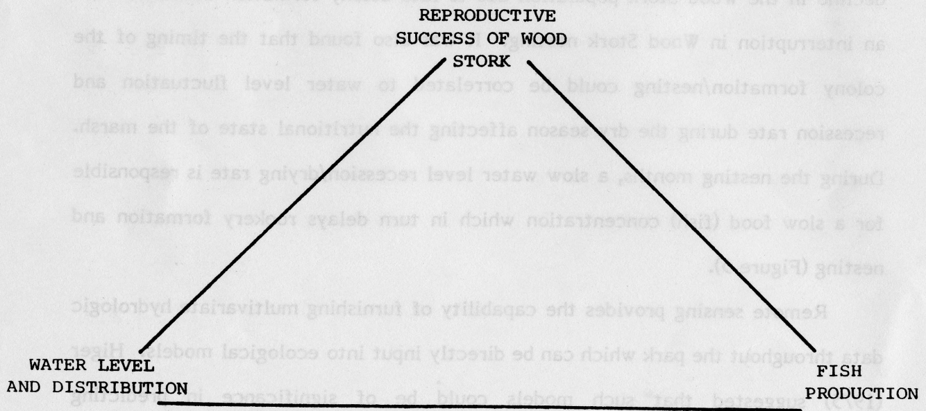
Figure 6. Wildlife ecological model of the Shark River Slough, Florida (Higer, 1975).
