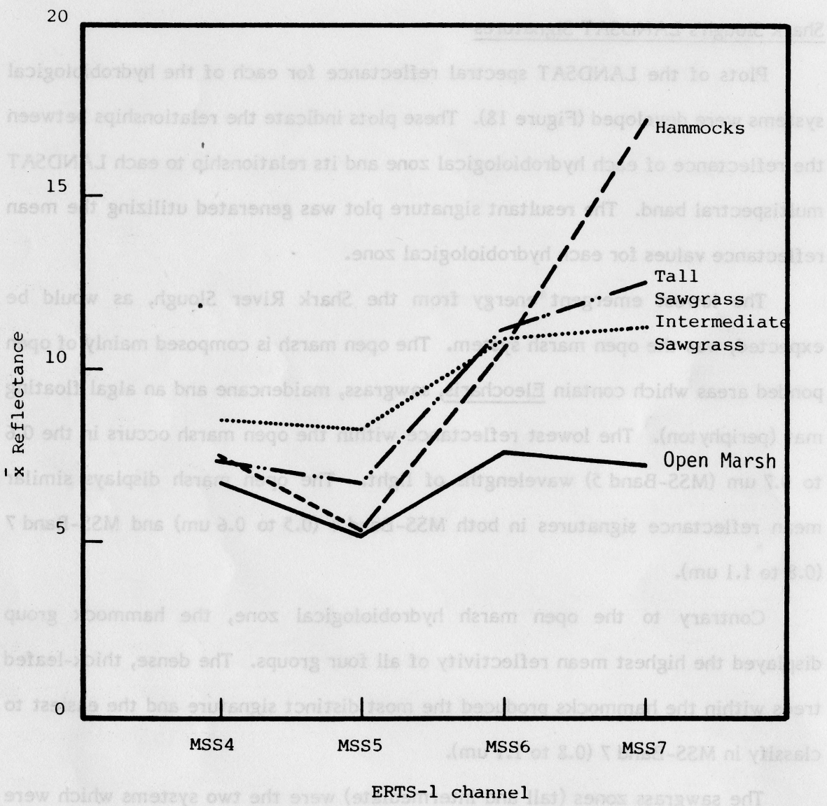
Figure 18. LANDSAT signatures of Shark Slough.
