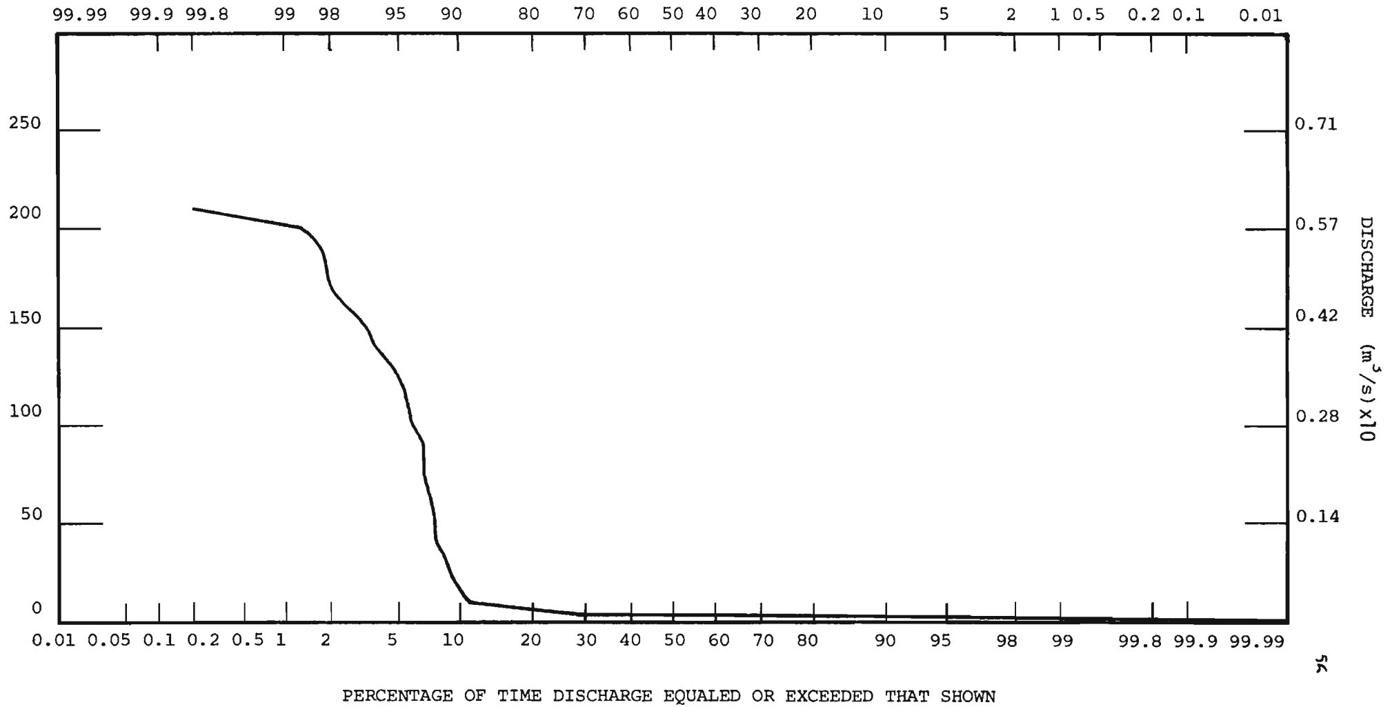
Figure 16: Flow Duration Curve: Taylor Slough at Context Road
