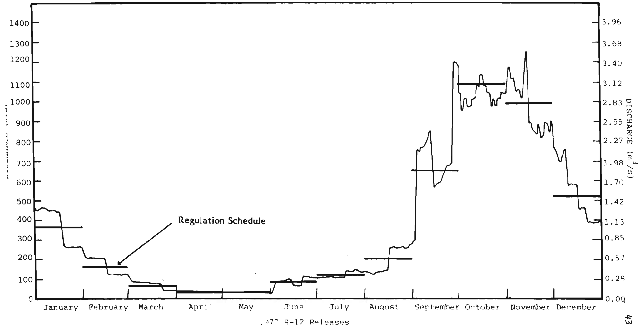
Figure 11: 1977 S-12 Release Hydrograph
