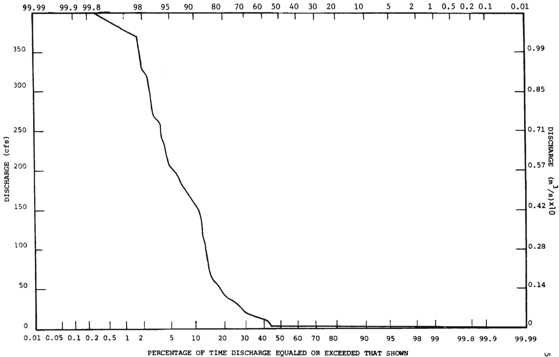
Figure 15: Flow Duration Curve, Taylor Slough at Bridge
