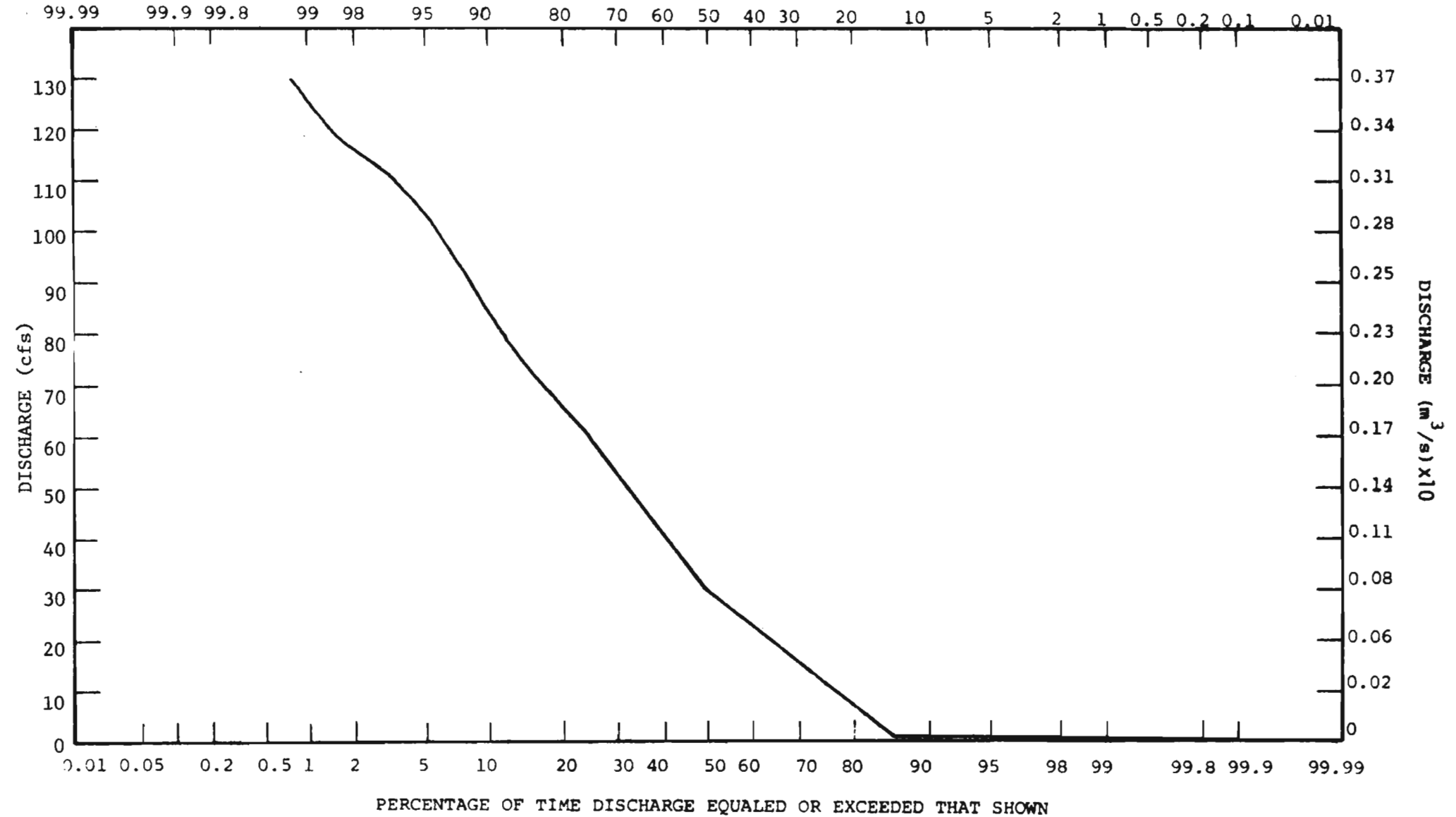
Figure 14: 1977 Flow Duration Curve, L-30 to L-67A
