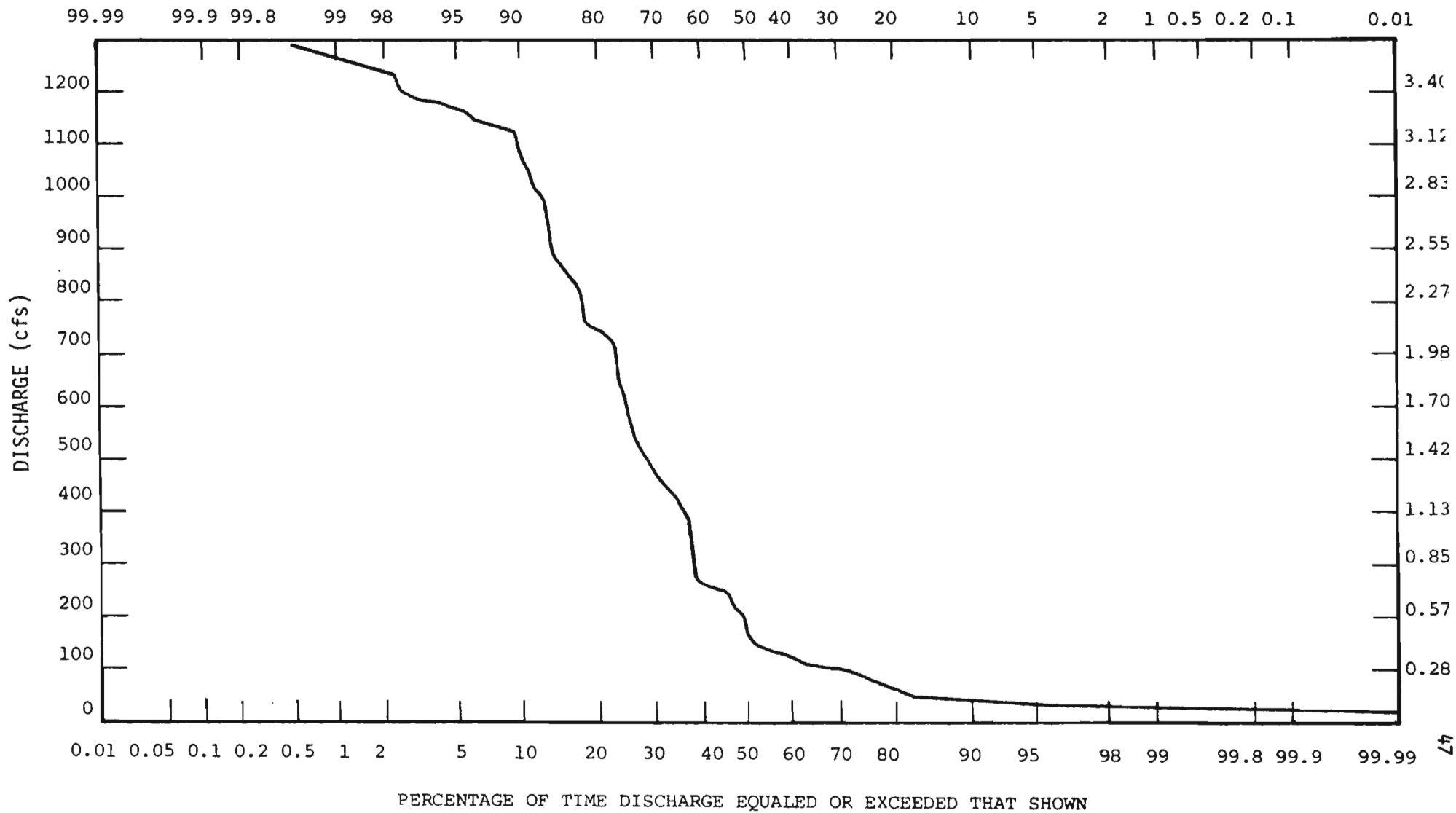
Figure 13: 1977 Flow Duration Curve, L-67A to 40 Mile Bend
